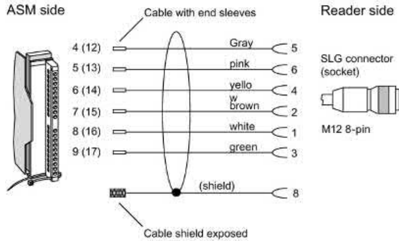
Figure A-14 Connecting cable between the ASM 475 and RF2xx reader (RS-422)
