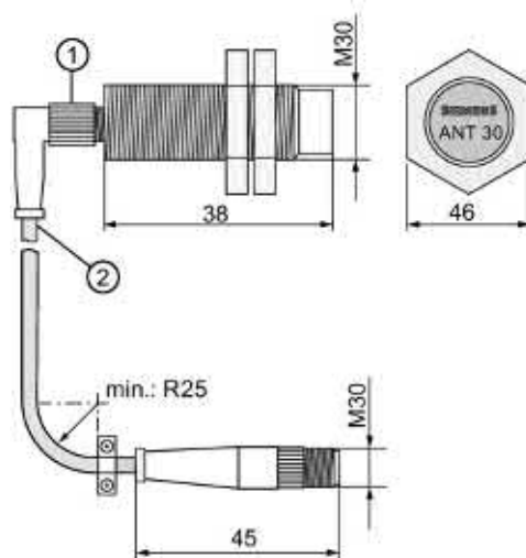
Figure 6-49 Dimension drawing ANT 30 (stainless steel variant)
