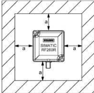
Figure 4-12 Metal-free space for RF260R
