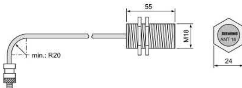
Figure 6-34 Dimension drawing ANT 18 (all values in mm)
