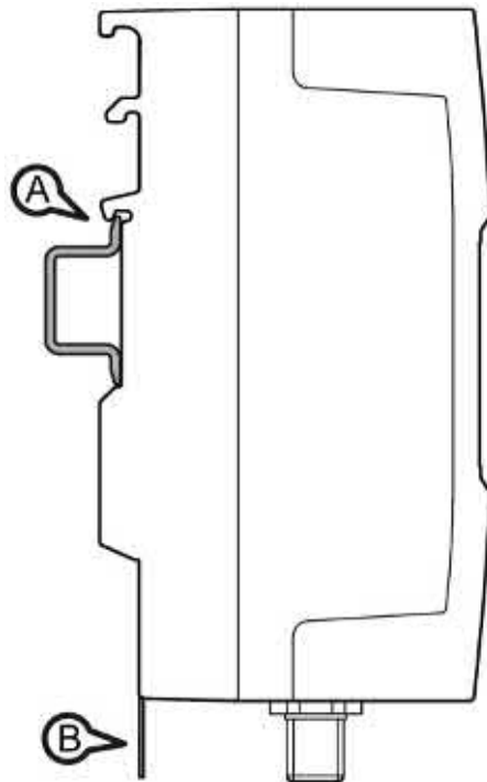
Figure 5-28 Mounting the RF290R reader on a DIN rail
