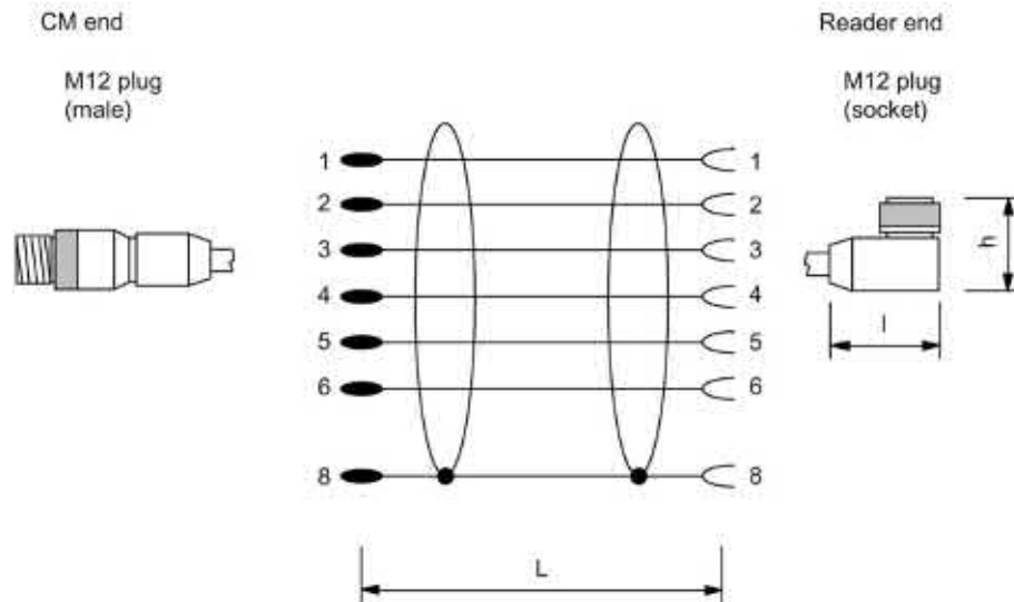
Figure A-12 Connecting cable between ASM 456, RF160C, RF170C, RF180C, RF18xC and RF2xxR reader (RS-422) with angled connector
