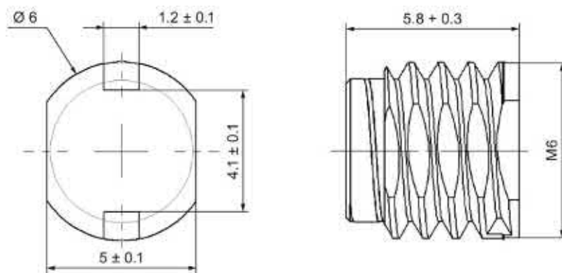
Figure 7-14 Dimensions in mm
