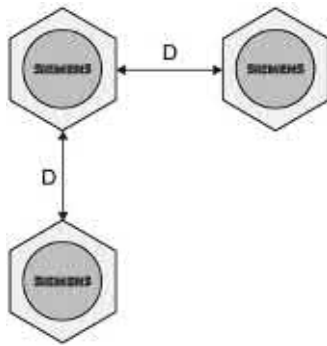
Figure 6-42 Minimum distance for ANT 30
