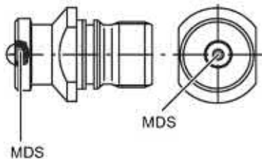
Figure 7-64 Installation example of MDS D521 in a stud bolt
