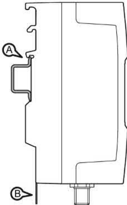
Figure 5-22 Installing the RF285R reader on a DIN rail
