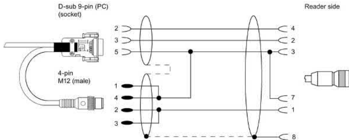
Figure A-16 Connecting cable between PC and RF240R/RF260R/RF285R/RF290R (RS232) with 4-pin power supply connector
