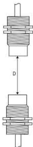
Figure 6-47 Minimum distance ANT 30 (stainless steel variant)
