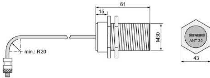
Figure 6-44 Dimension drawing ANT 30 (all values in mm)
