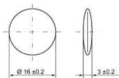
Figure 7-82 Dimension drawing of MDS D560
