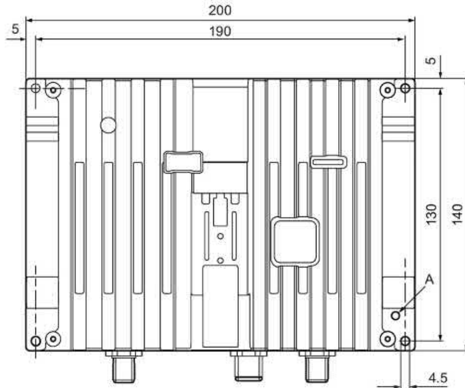
Figure 5-25 Drilling pattern for the RF290R (dimensions in mm)
