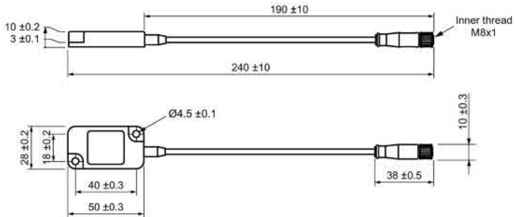
Figure 6-9 Dimension drawing ANT 3 (all values in mm)
