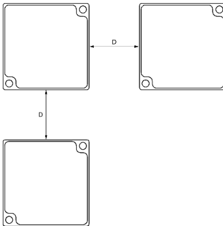
Figure 6-2 Minimum distance ANT 1
