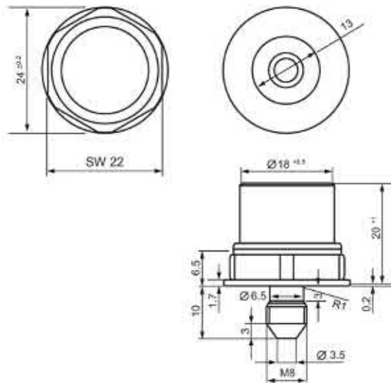
Figure 7-80 Dimensional drawing of MDS D528
