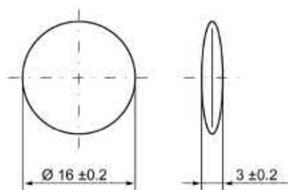
Figure 7-59 Dimensional drawing of MDS D460
