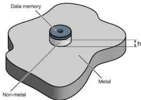
Figure 7-15 Mounting the MDS D139 on metal with spacer
