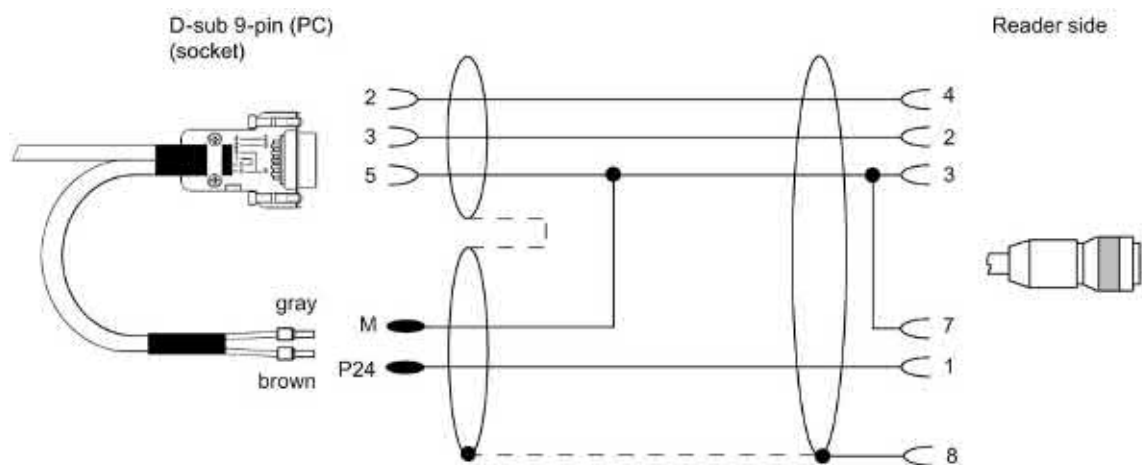
Figure A-17 Connecting cable between PC and RF240R/RF260R/RF285R/RF290R (RS232) with open ends for the power supply
