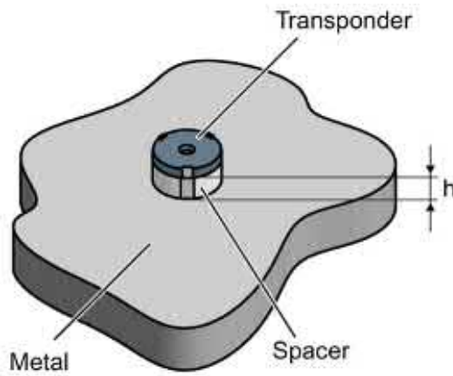
Figure 7-10 Mounting the MDS D126 / D426 / D526 on metal with spacer
