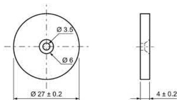
Figure 7-73 Dimensional drawing of MDS D524
