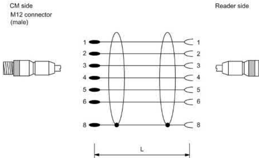
Figure A-11 Connecting cable between ASM 456, RF160C, RF170C, RF180C, RF18xC, RF182C and RF2xxR reader (RS422)
