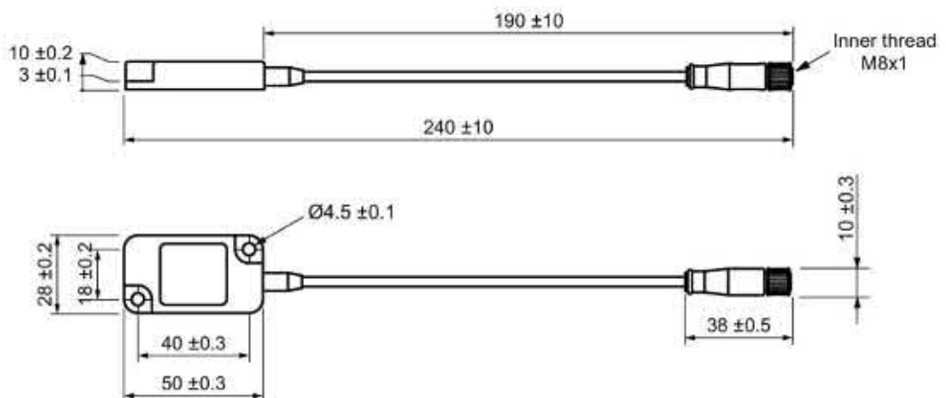
Figure 6-14 Dimension drawing ANT 3S (all values in mm)
