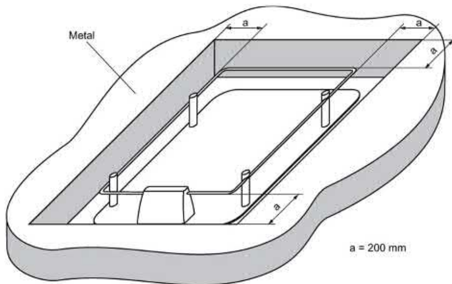
Figure 6-59 Metal-free area for ANT D6
