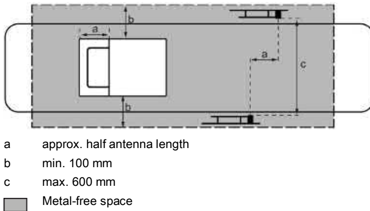
Figure 4-21 Metal-free space, view from above (based on the example of a tunnel arrangement on a conveyor belt)
