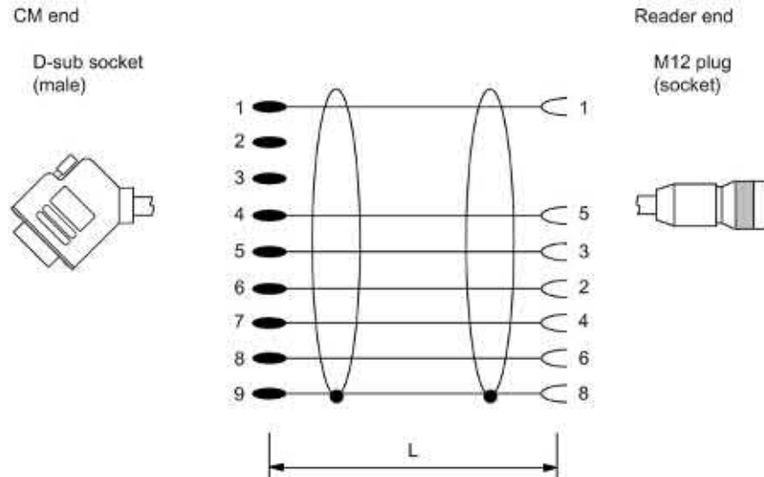
Figure A-15 Connecting cable between RF120C and RF2xxR reader (RS-422)
