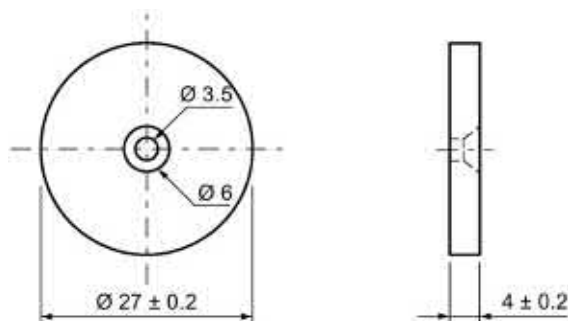
Figure 7-9 Dimension drawing of MDS D124
