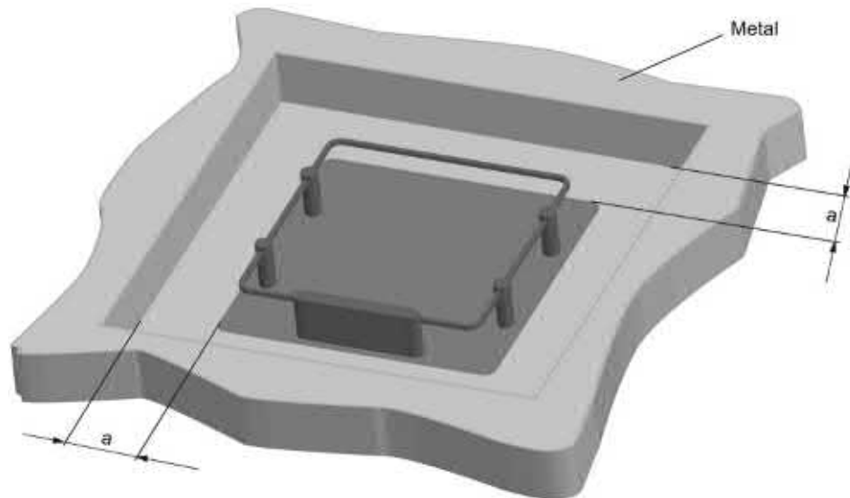
Figure 6-55 Metal-free area for ANT D5
