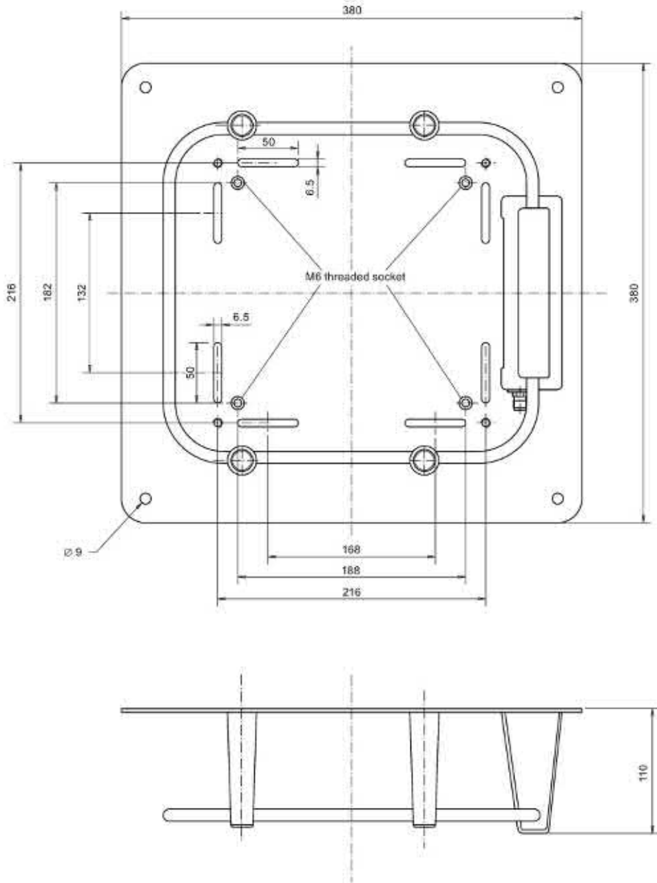
Figure 6-57 Dimension drawing for ANT D5
