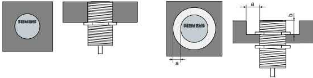
Figure 4-11 Metal-free space for ANT 8 / ANT 12 and ANT 18 / ANT 30
