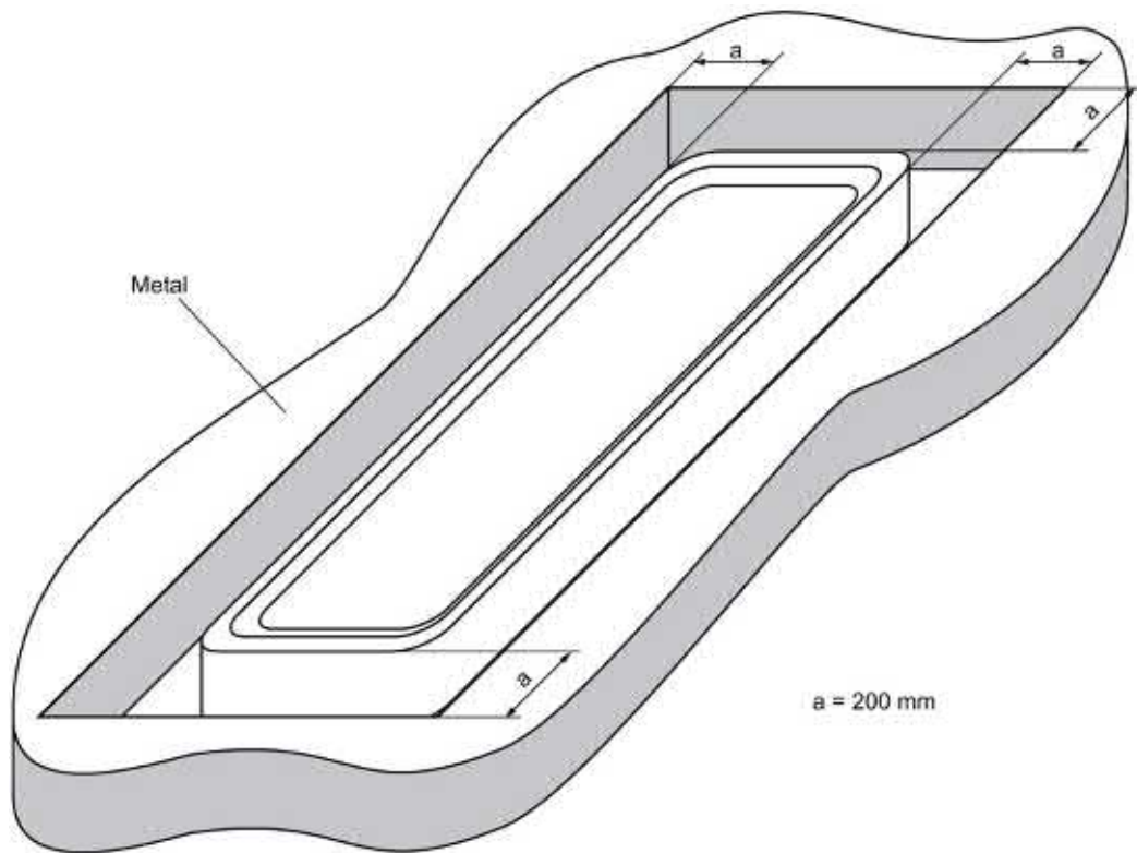
Figure 6-63 Metal-free area for ANT D10
