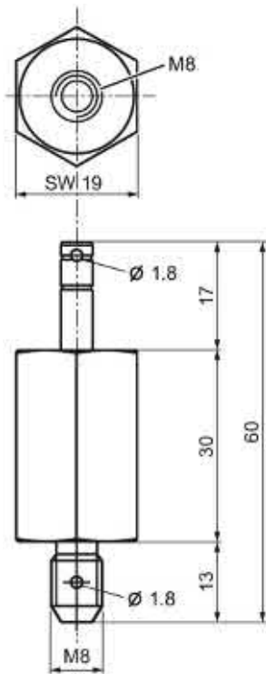
Figure A-5 Dimension drawing of quick change holder 6GT2690-0AH00
