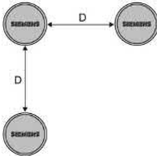
Figure 6-17 Minimum distance for ANT 8
