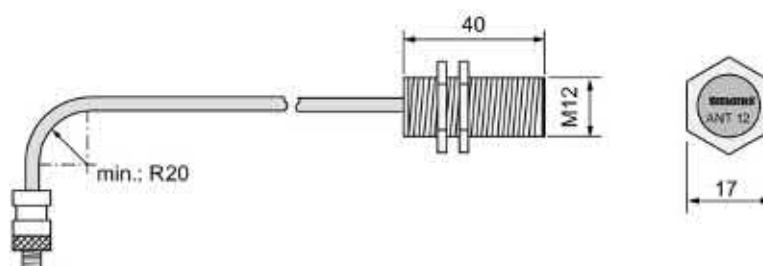
Figure 6-24 Dimension drawing ANT 12 (all values in mm)
