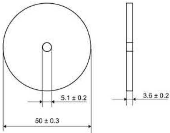
Figure 7-12 Dimension drawing of MDS D126
