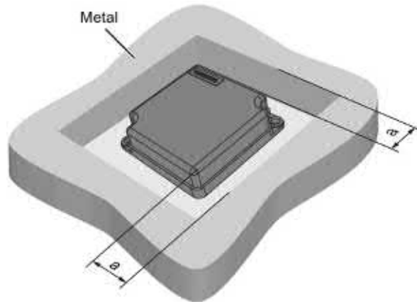
Figure 6-50 ANT D1 flush-mounted in metal
