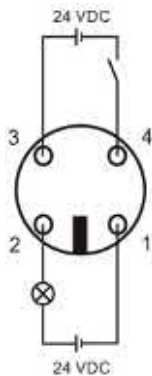
Figure 5-24 Pin assignment of the power supply connector
