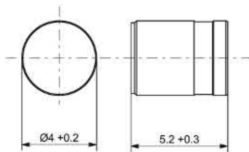
Figure 7-5 Dimensions in mm
