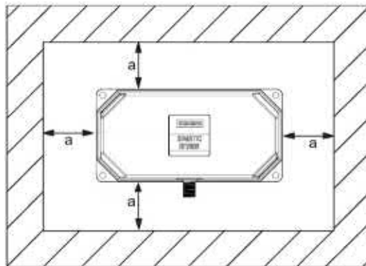
Figure 4-13 Metal-free area RF280R
