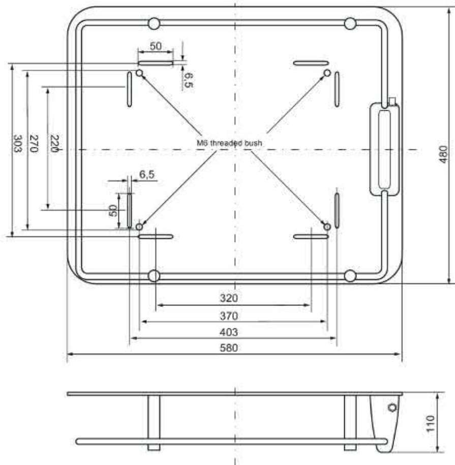
Figure 6-61 Dimension drawing for ANT D6
