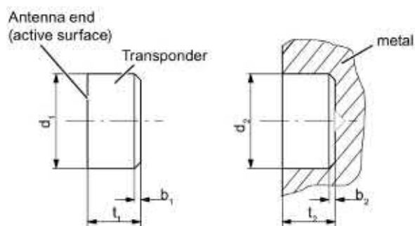
Figure 7-62 Flush-mounting of MDS D521 in metal with tools
