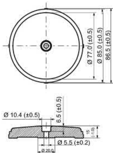
Figure 7-18 Dimensional drawing of MDS D139
