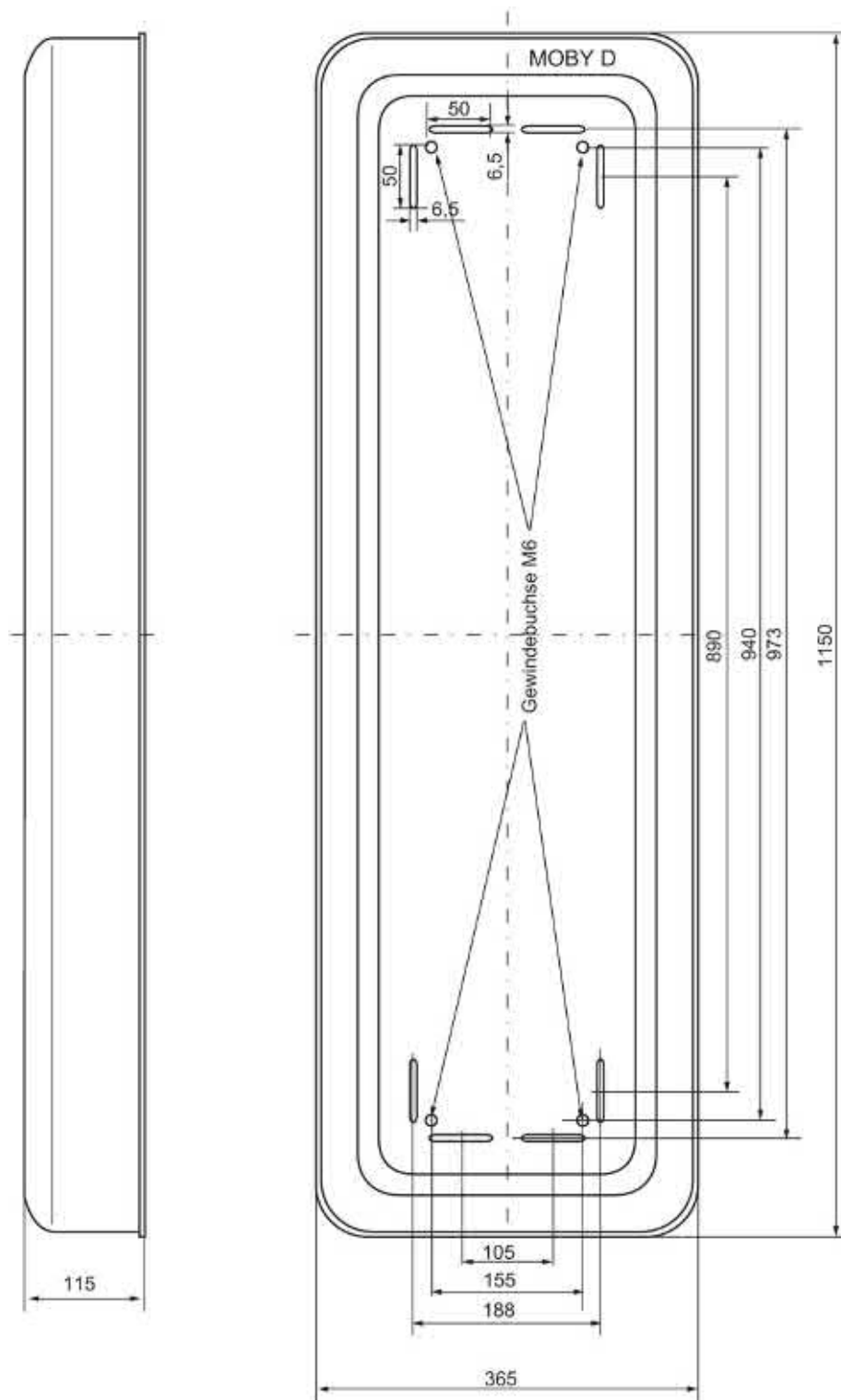
Figure 6-65 Dimension drawing for ANT D10
