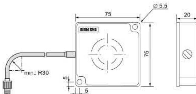
Figure 6-53 Dimension drawing ANT D1 (all values in mm)
