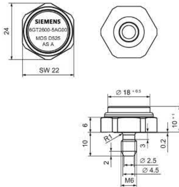
Figure 7-75 Dimensional drawing of MDS D525
