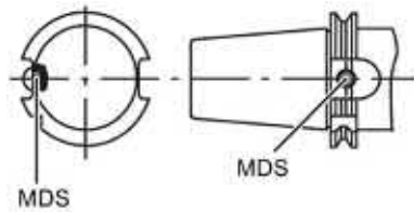
Figure 7-39 Installation example of MDS D421 in a steep cone
