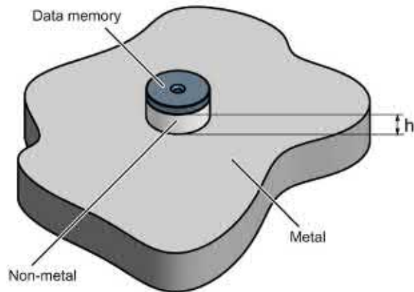
Figure 7-71 Mounting the MDS D124/D324/D424/D524/E624 and RF320T on metal with spacer
