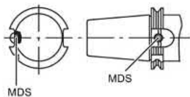
Figure 7-63 Installation example of MDS D521 in a steep cone
