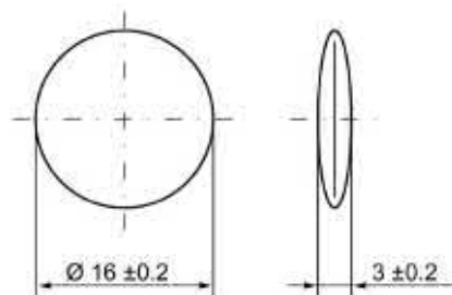
Figure 7-20 Dimensional drawing of MDS D160
