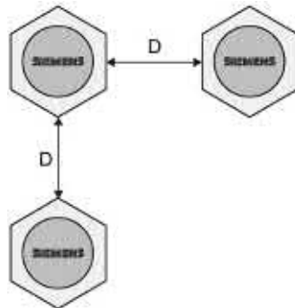
Figure 6-37 Minimum distance ANT 18 (stainless steel variant)
