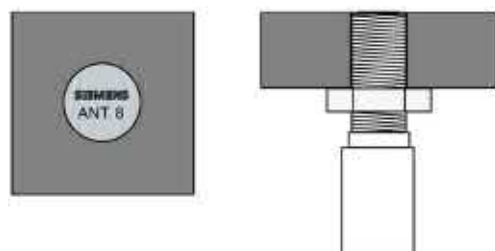
Figure 6-16 ANT 8 flush-mounted in metal
