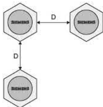
Figure 6-47 Minimum distance ANT 30 (stainless steel variant)
