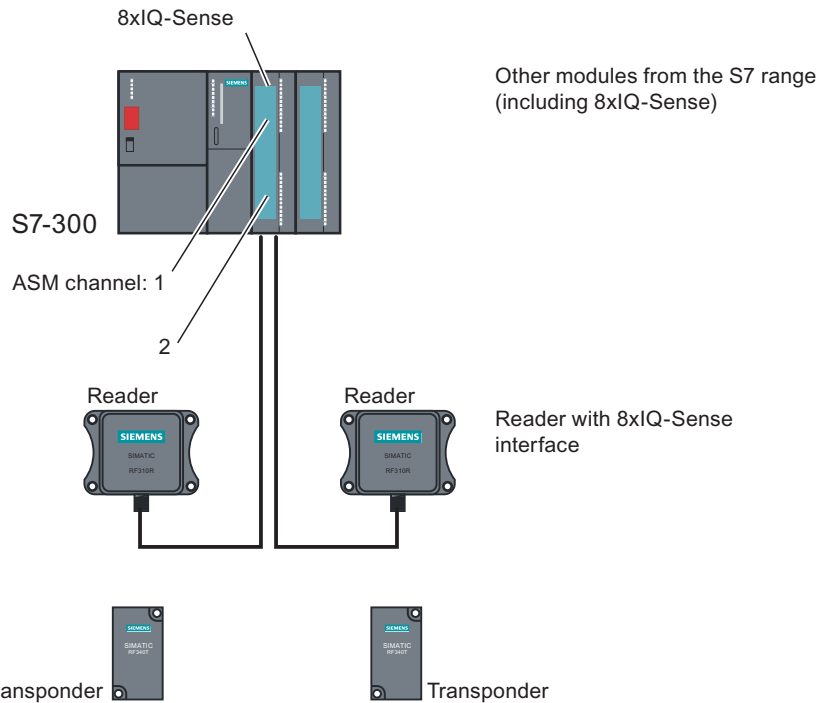
Figure 7-2 RF310R reader with 8xIQ-Sense interface
