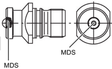
Figure 8-63 Installation example of MDS D421/D521/E623 in a stud bolt
