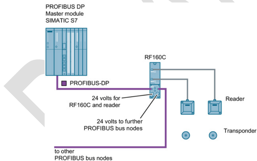
Figure 9-8 Configuration RF160C
