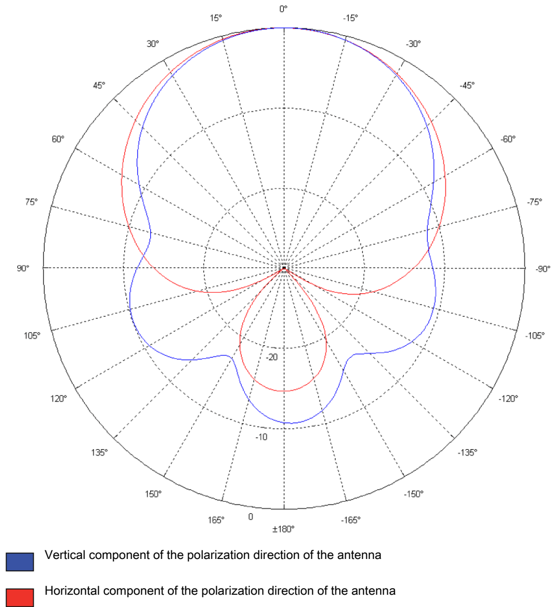
Figure 1-1 Azimuth section
