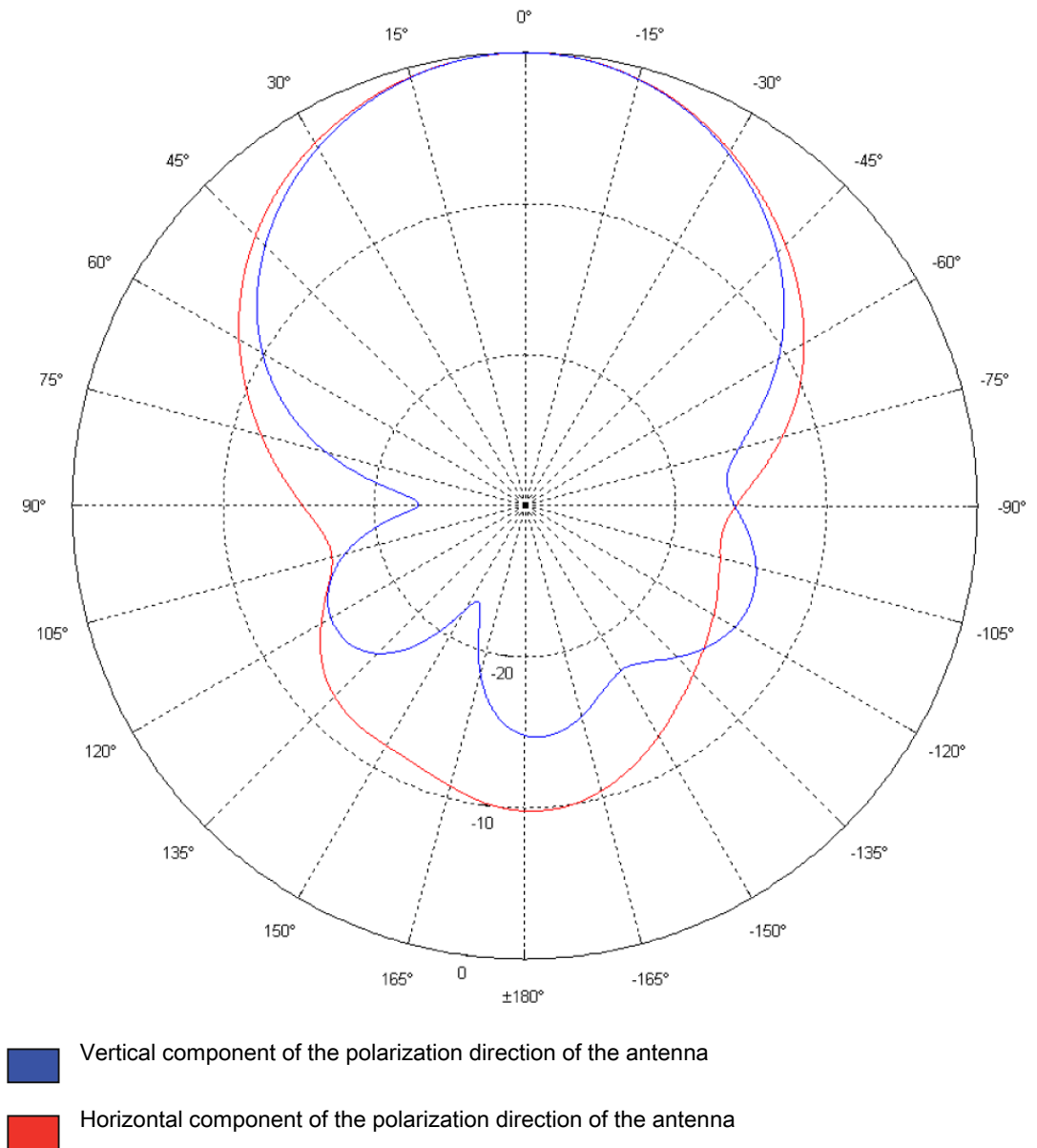
Figure 1-2 Elevation section
