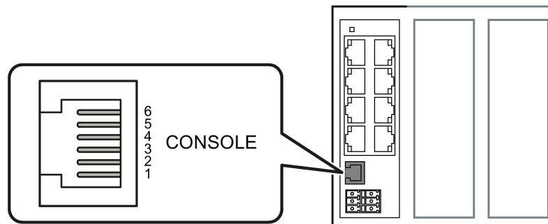
Figure 4-2 Position and pin assignment of the serial interface (RJ-12 jack), for example on the SCALANCE XB213-3
