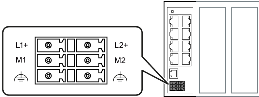
Figure 4-1 Position of the power supply, for example on the SCALANCE XB213-3
