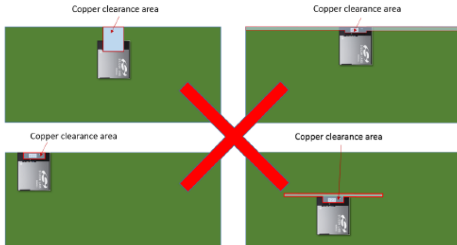
Figure 6.2. Non-optimal Module Placements for MGM12P
