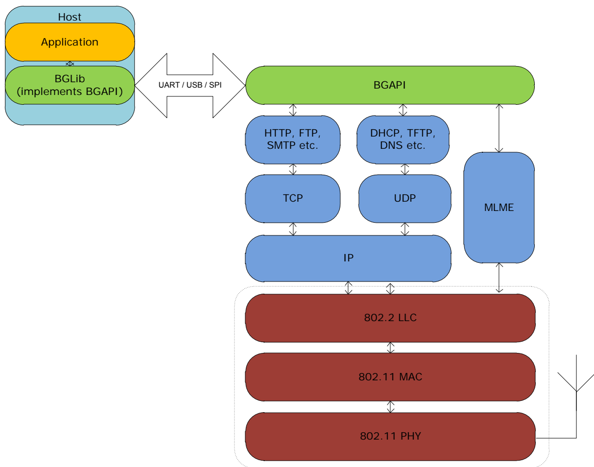
Figure 3: WF121 software
