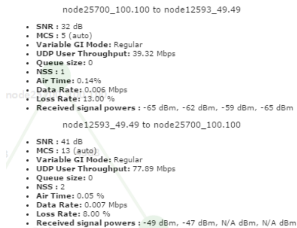
Figure 55 Link Characteristics
