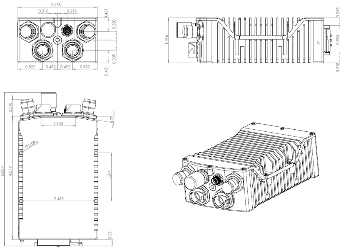
Figure 19 SC4200 Mechanical Drawing (top) and Mounting Pattern (bottom)
