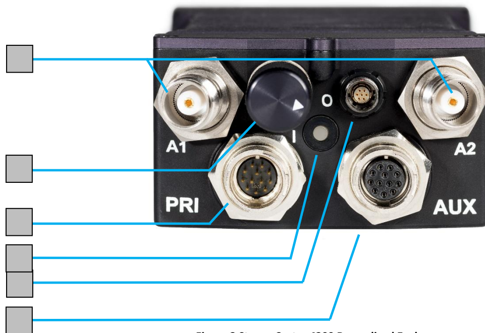
Figure 3 StreamCaster 4200 Ruggedized Enclosure
