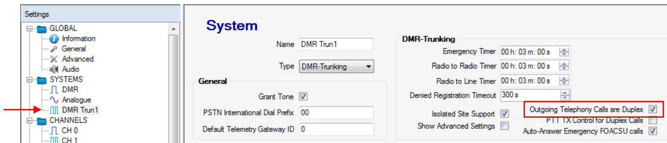
Figure 8. Duplex Setup in FPP.
