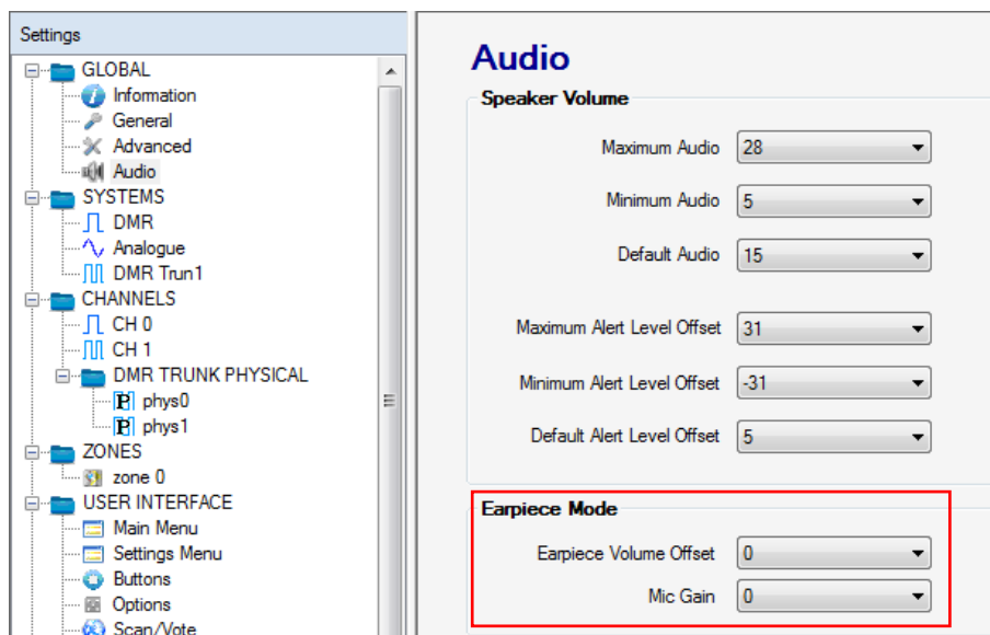
Figure 10. FPP – Earpiece Volume and Mic Gain settings.
