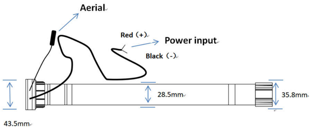
M3310EIG Side view
