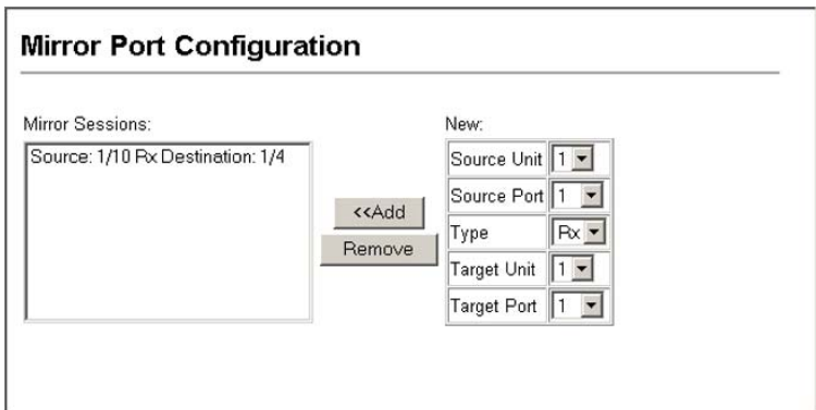
Figure 3-49 Mirror Port Configuration
