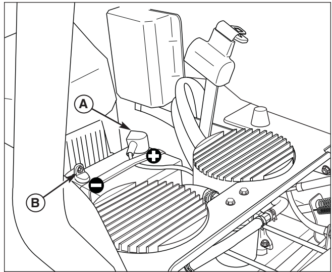
Figure 45. Battery Compartment A. Positive (+) Cable & Terminal B. Negative (-) Cable & Terminal
