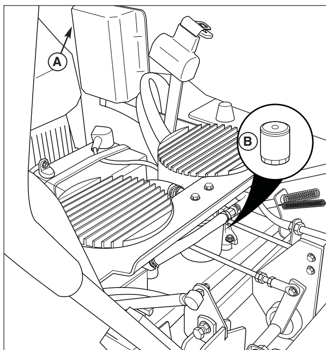
Figure 26. Battery Compartment A. Hydraulic Oil Reservoir B. Hydraulic Oil Filter
