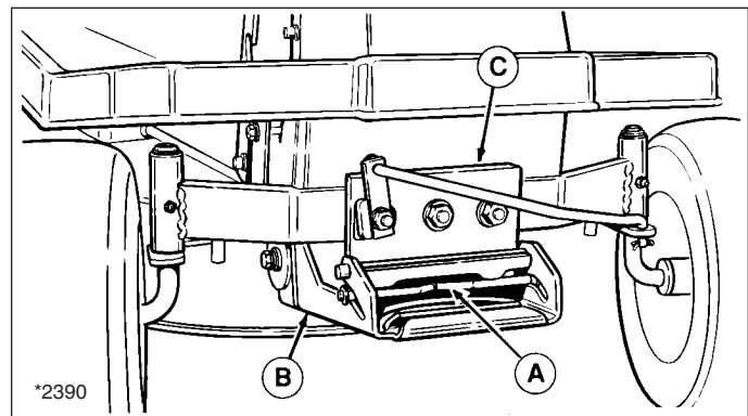
Figure 8. Mower Hitch
