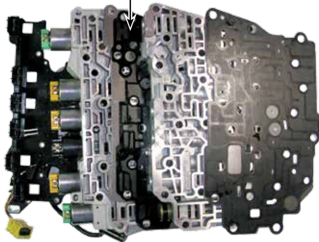
Separator Plate
