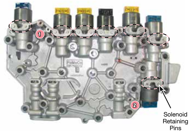
Assembled Valve Body with Lead Frame Removed
