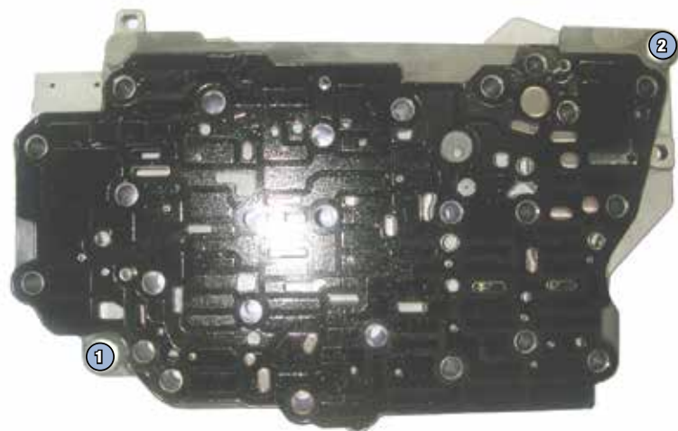
Separator Plate Removal
