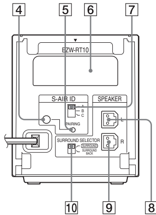
Rear panel
