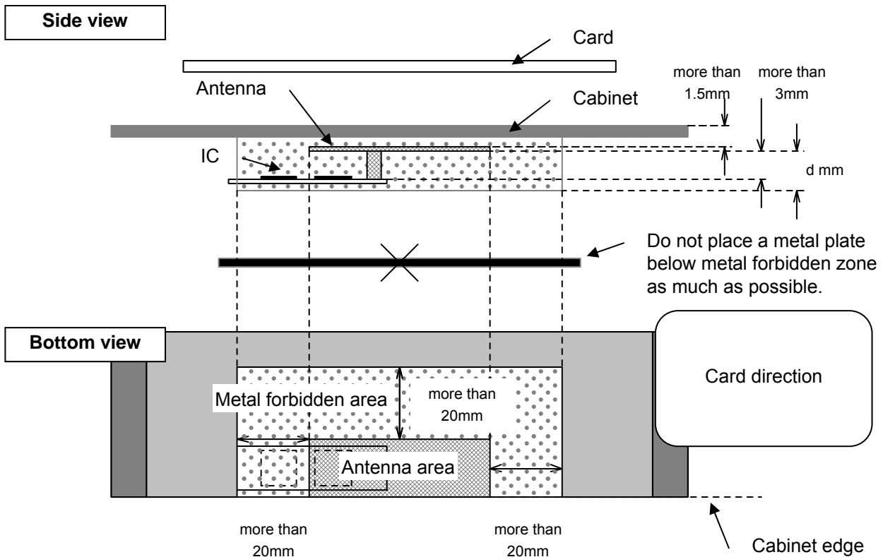
Figure A-1: Installation requirements
