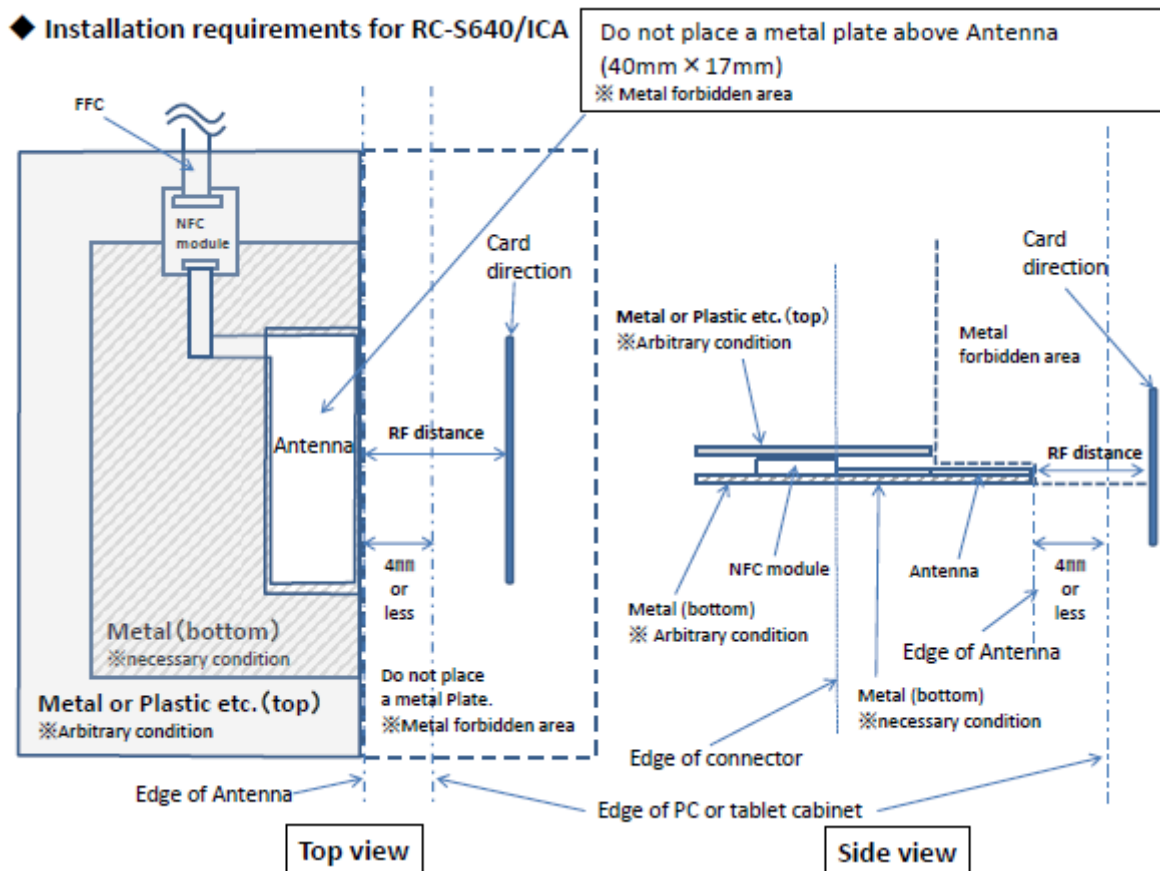
Figure B-1: Installation requirements
