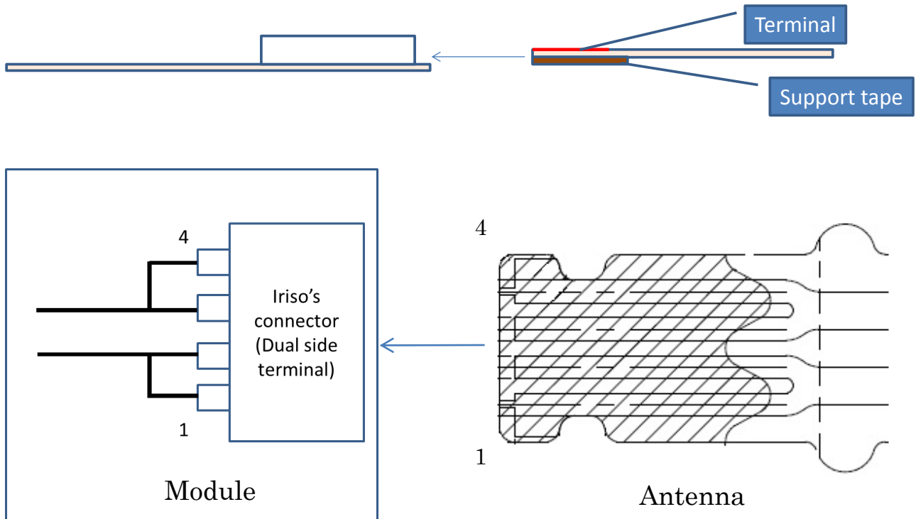
Figure A-2 Connection of a module and an antenna
