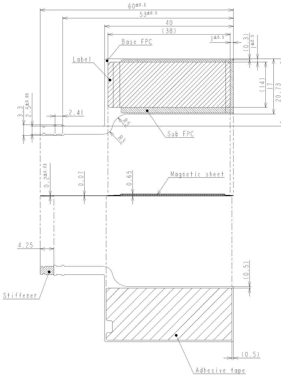
Figure A-1 External dimensions of antenna.
