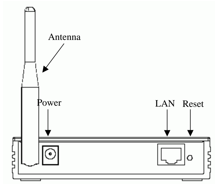
Figure 2 – Wireless 802.11g Multi-mode AP Rear Panel
