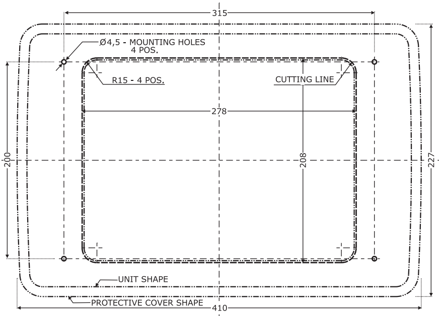
Figure 18a - CP500 Flush Mount cutout (Dimensions are in mm)
