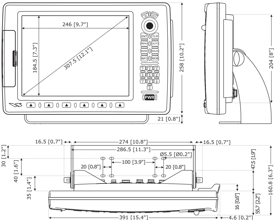
Figure 18 - CP500 Dimensions [mm/inch]
