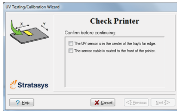
Figure 6-89: Sensor placement screen
