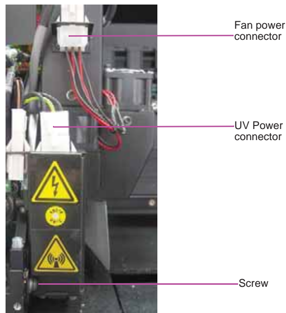
Figure 6-30: Disconnecting the right UV assembly
