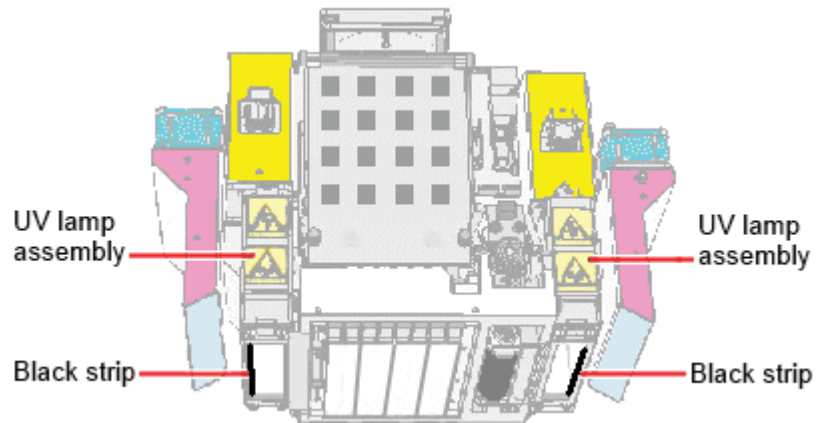
Figure 6-104: Print block and UV lamp assembly, showing correct placement of black strip
