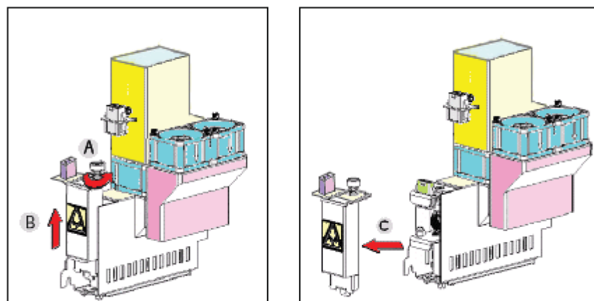
Figure 6-102: Removing the UV lamp cover
