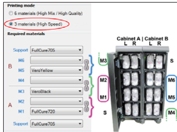
Figure 6-12: Manual cartridge placement
