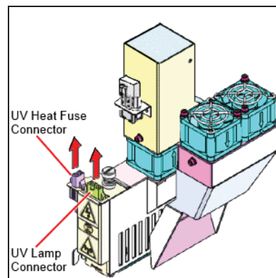
Figure 6-101: Disconnecting the UV lamp
