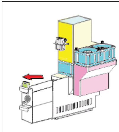
Figure 6-103: Removing the UV lamp reflector
