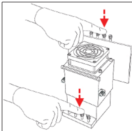
Figure 6-67: Releasing the print head
