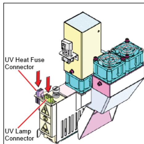
Figure 6-106: Connecting the UV lamp
