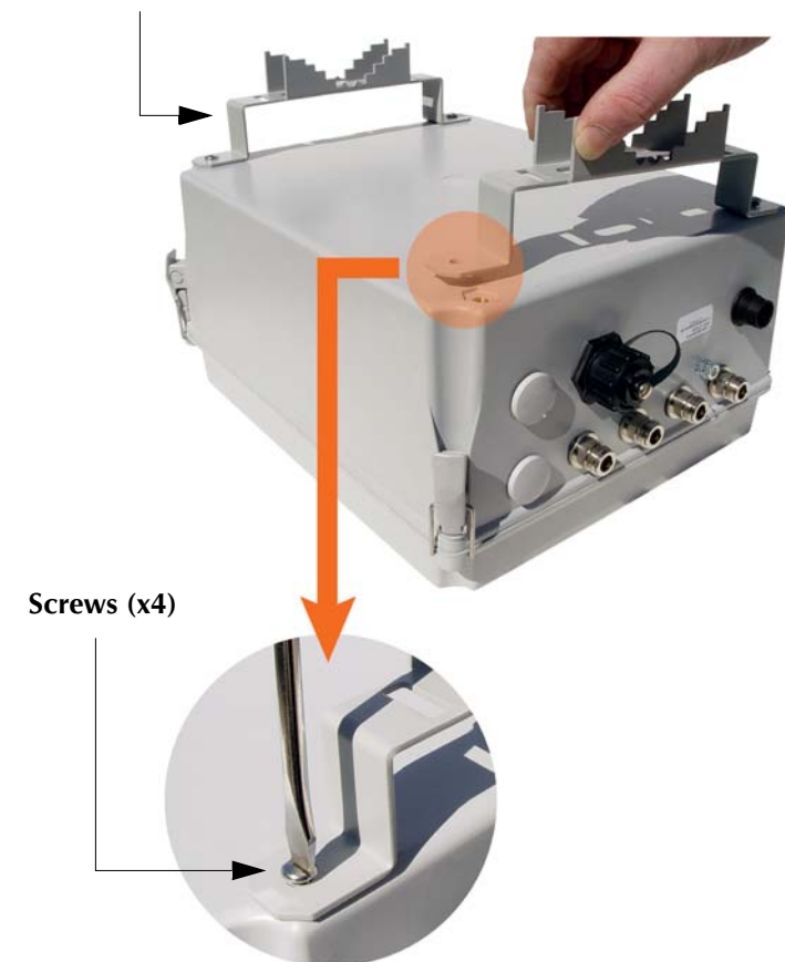
Mounting Brackets (x2)
