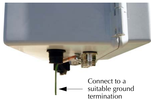
Ground Wire
