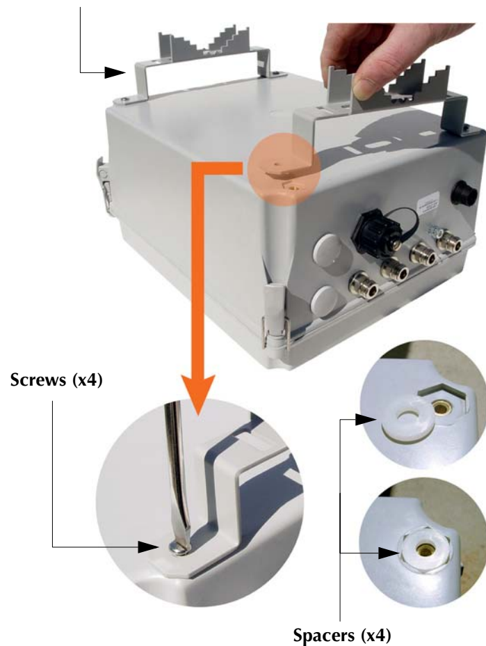
Mounting Brackets (x2)
