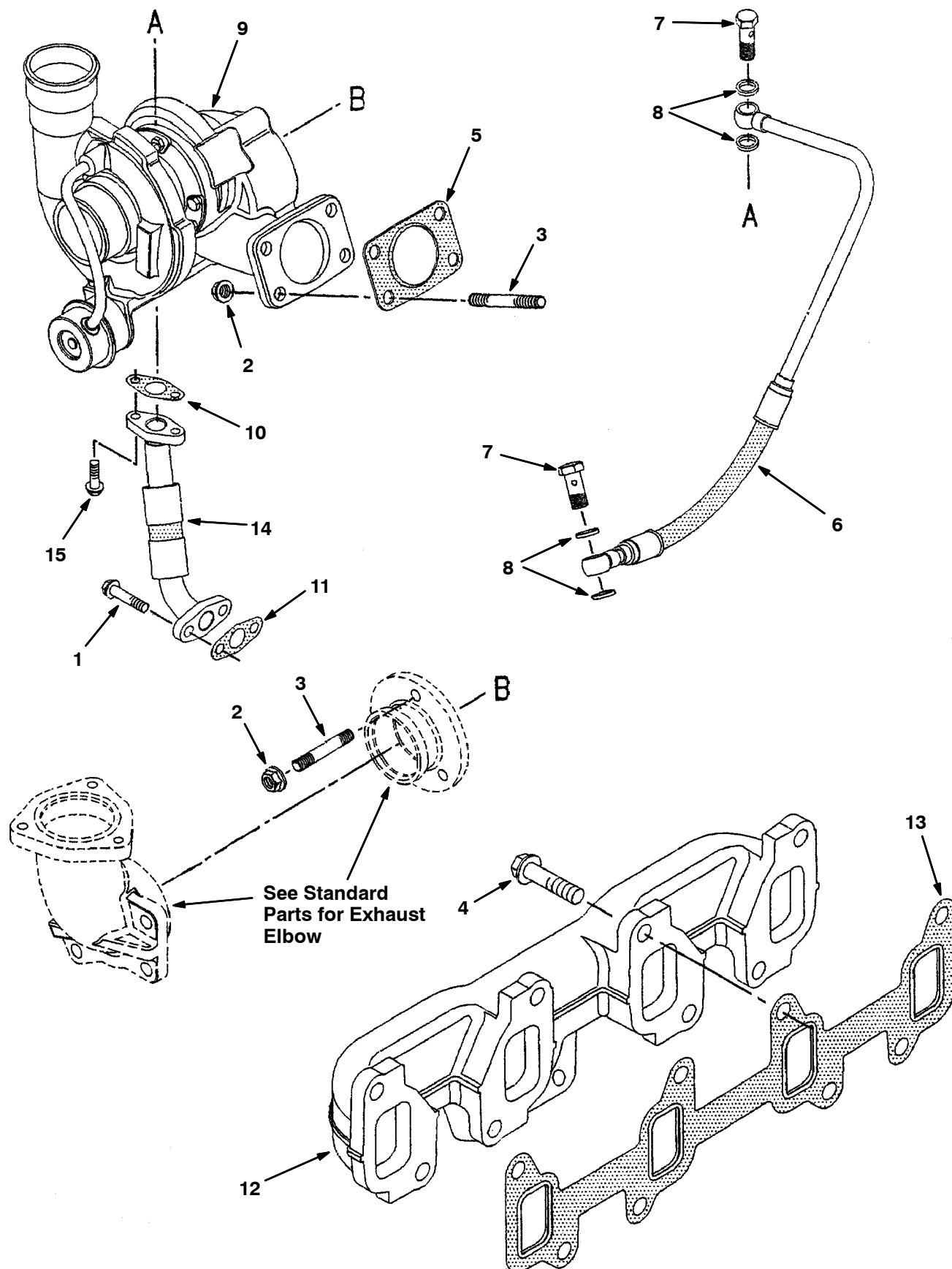
Fig. 25 - Turbocharger Group
