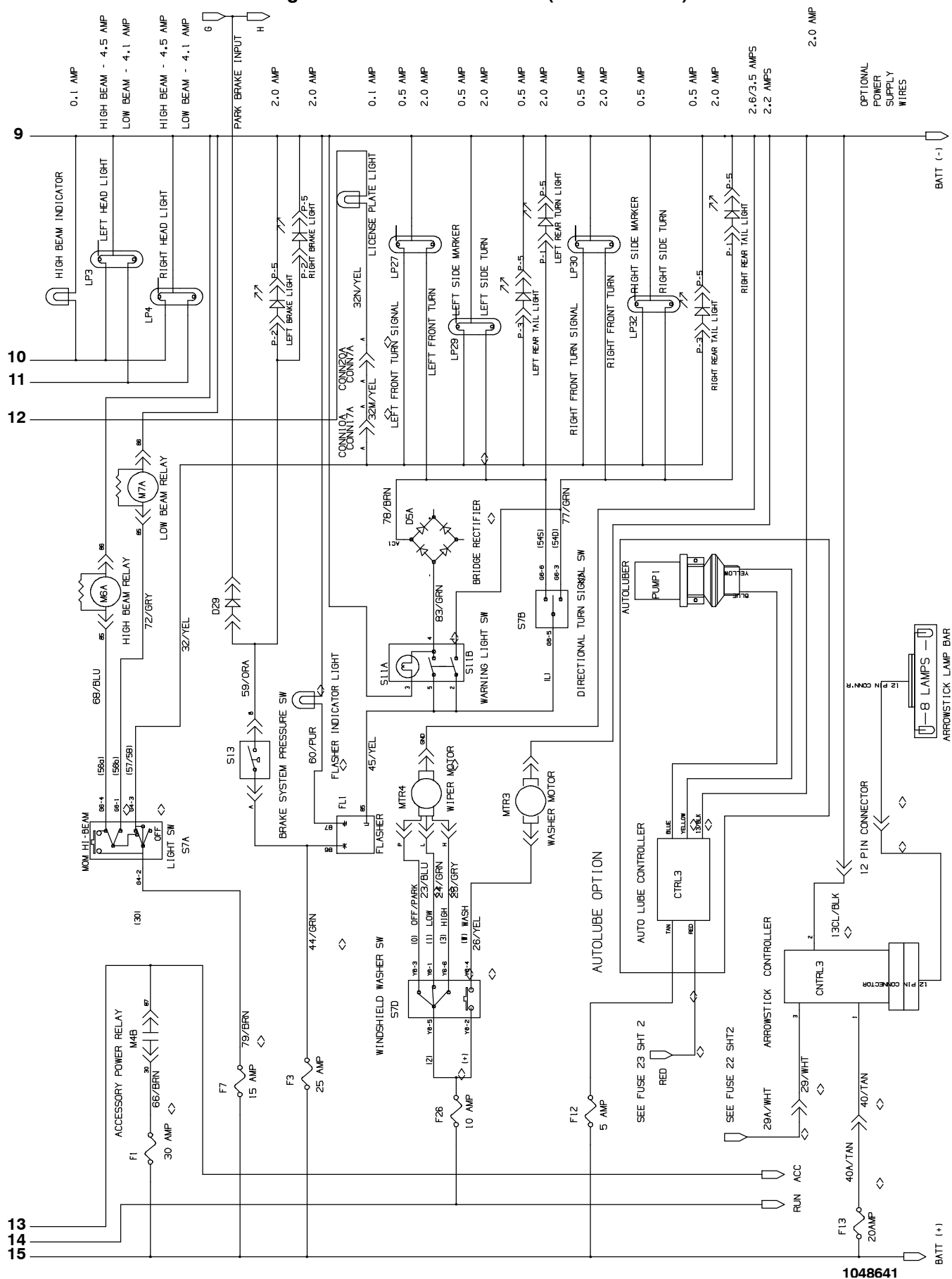
Fig. 72 - Electrical Schematic (008500- )
