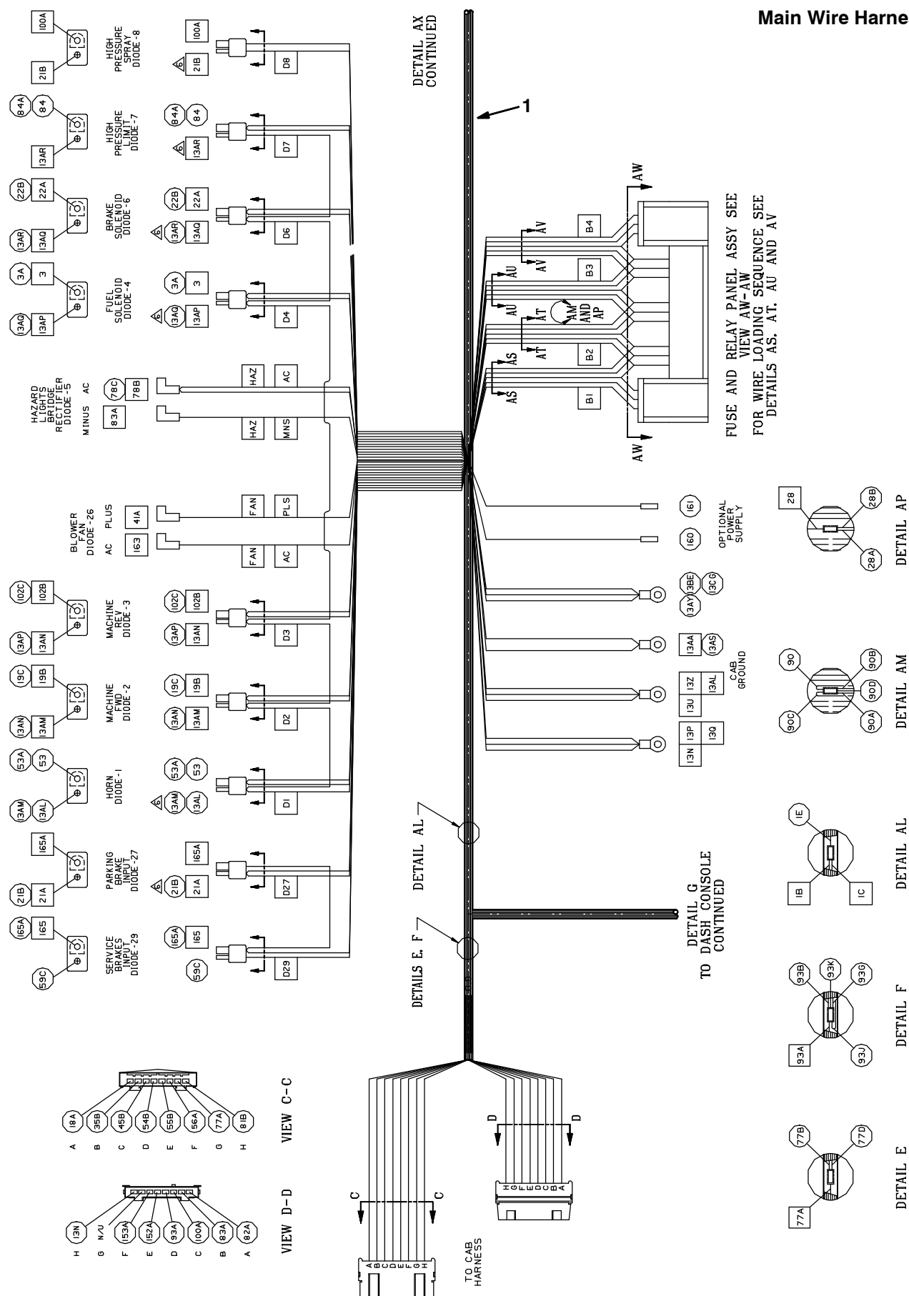
Fig. 73 - Wire Harnesses Group (000000-008499)
