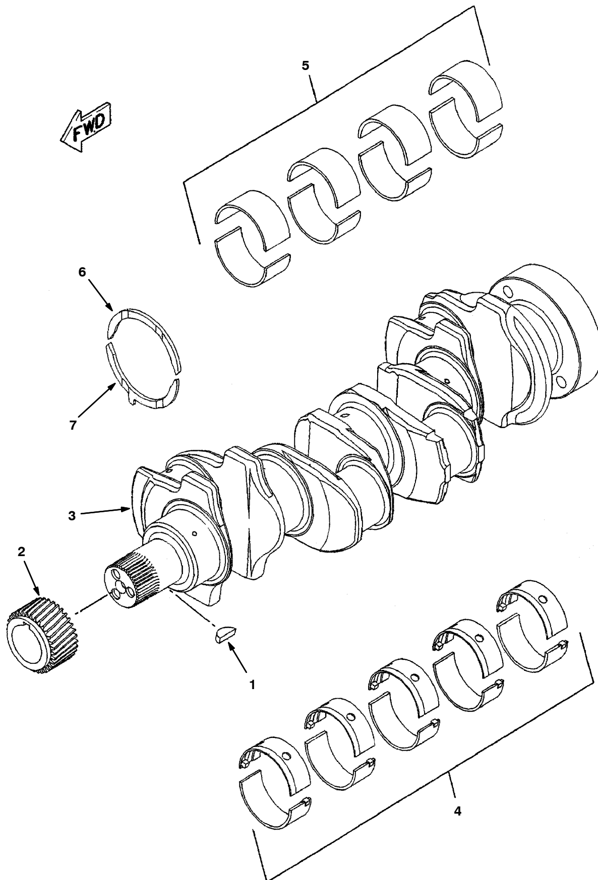
Fig. 20 - Crankshaft Group
