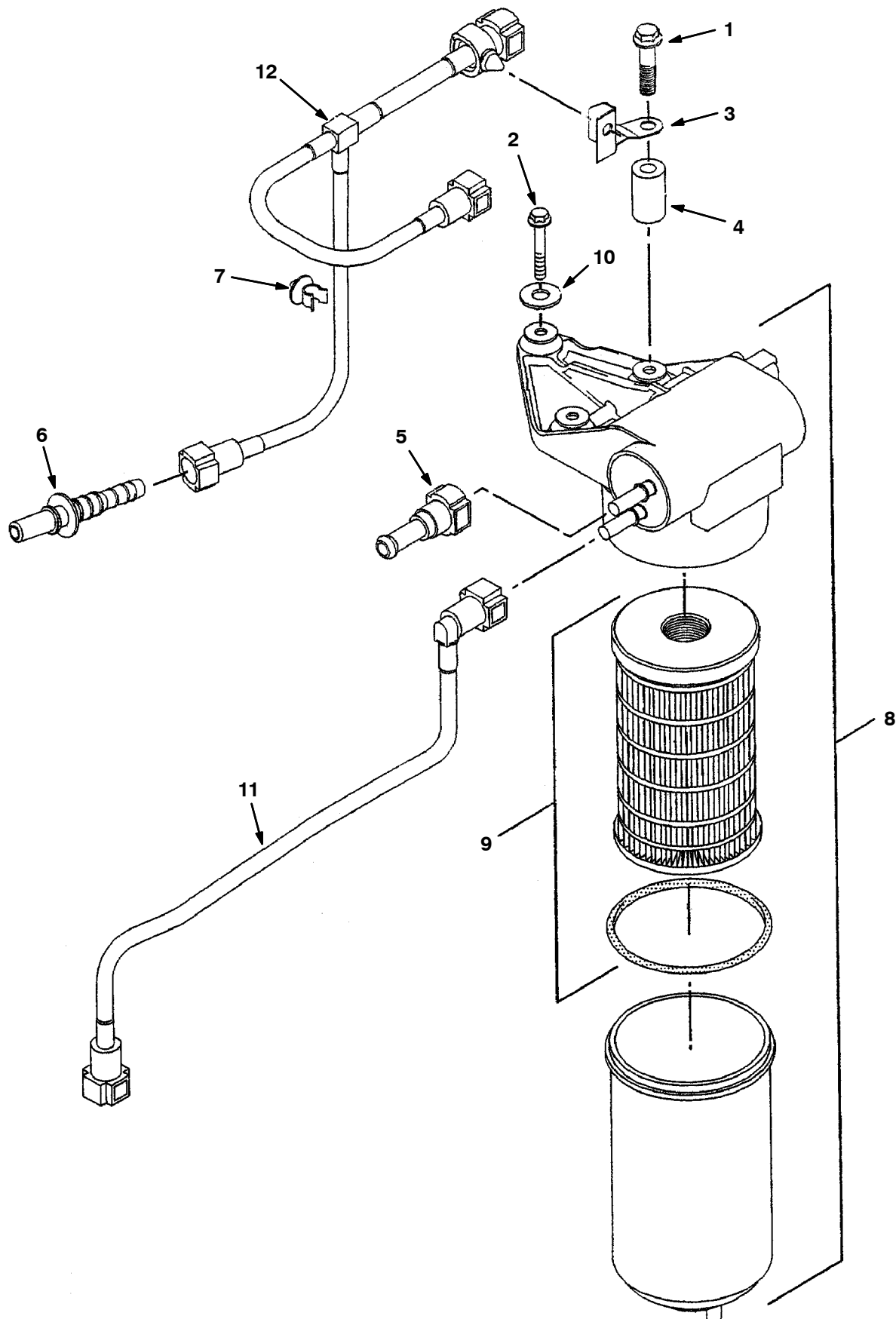
Fig. 6 - Fuel Filter Group
