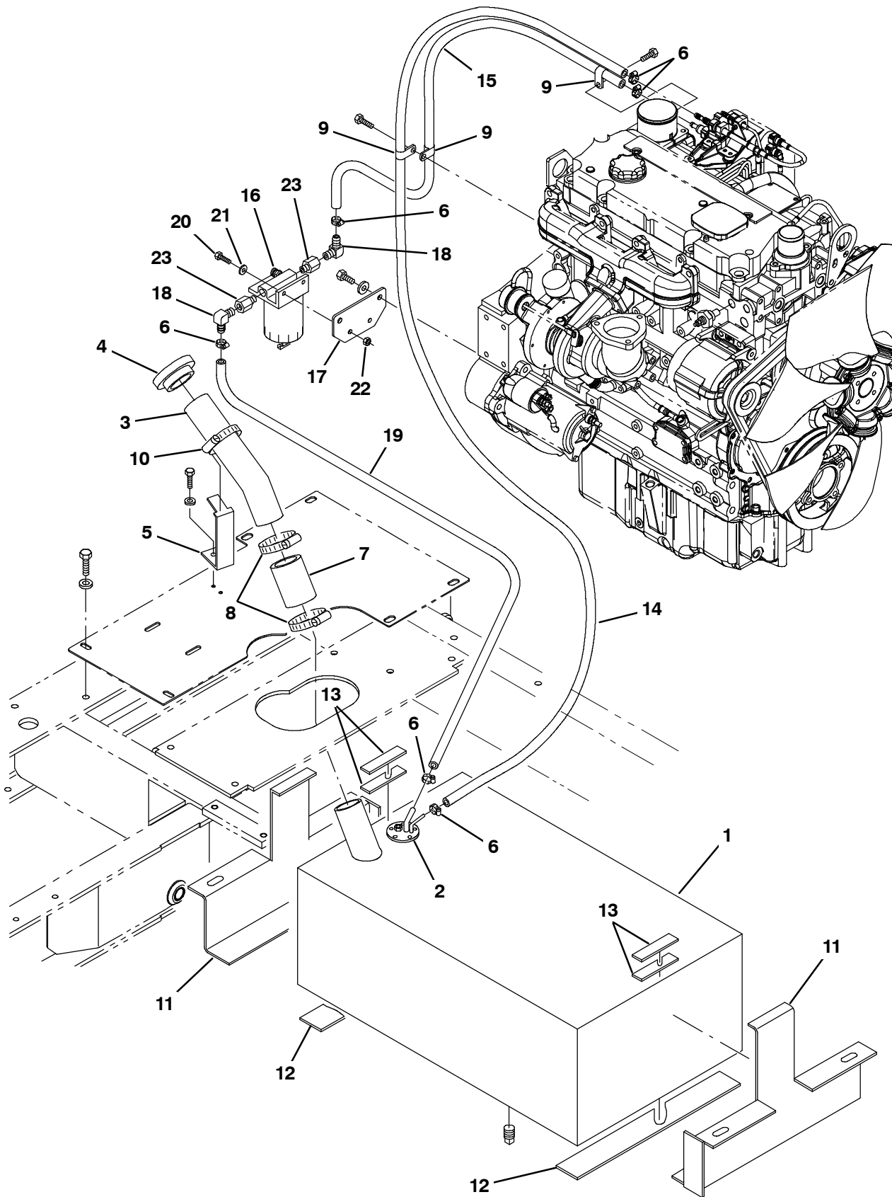
Fig. 17 - Engine Fuel Tank and Lines Group (008500- )
