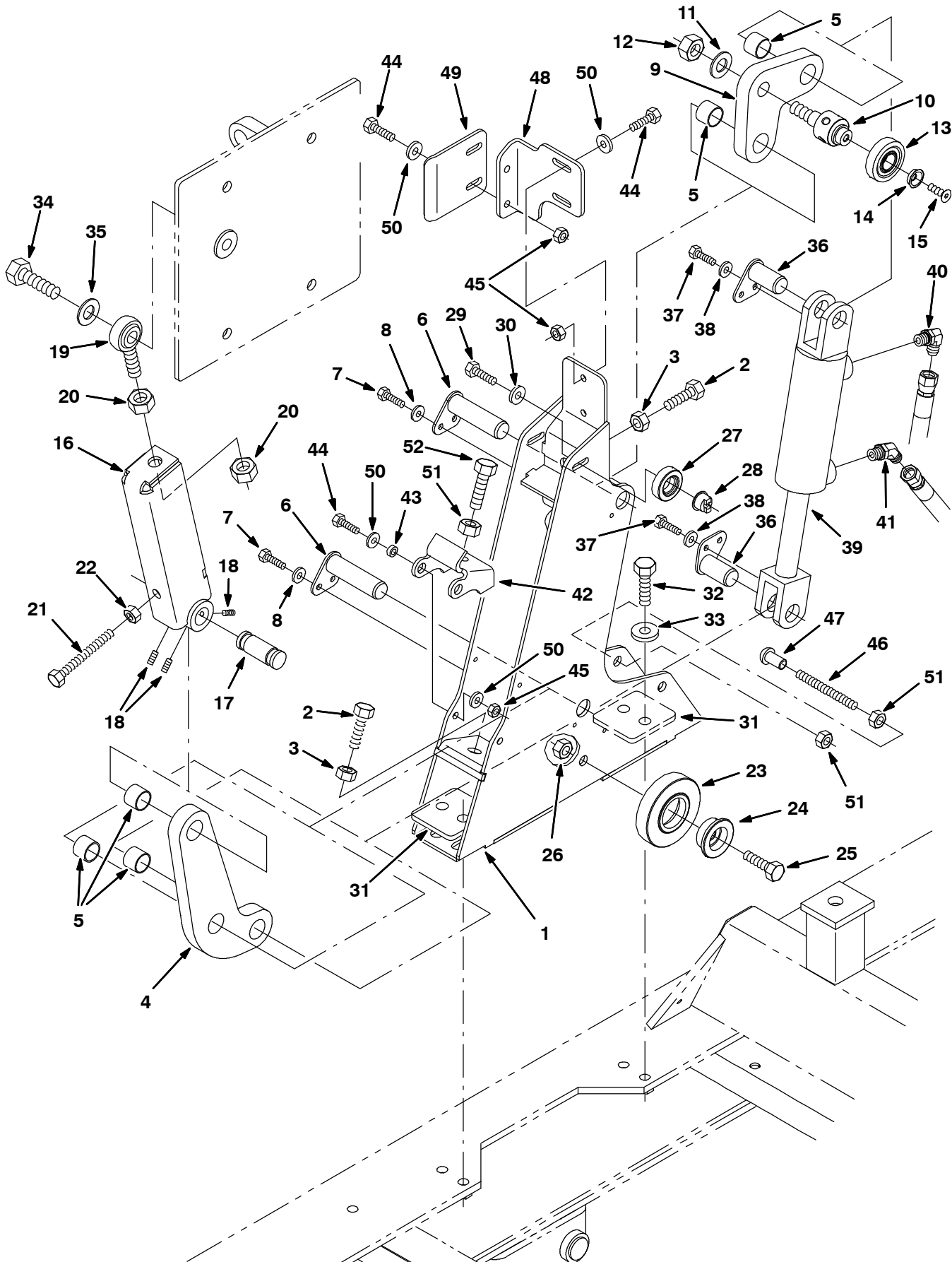
Fig. 32 - Conveyor Lift Group, Right
