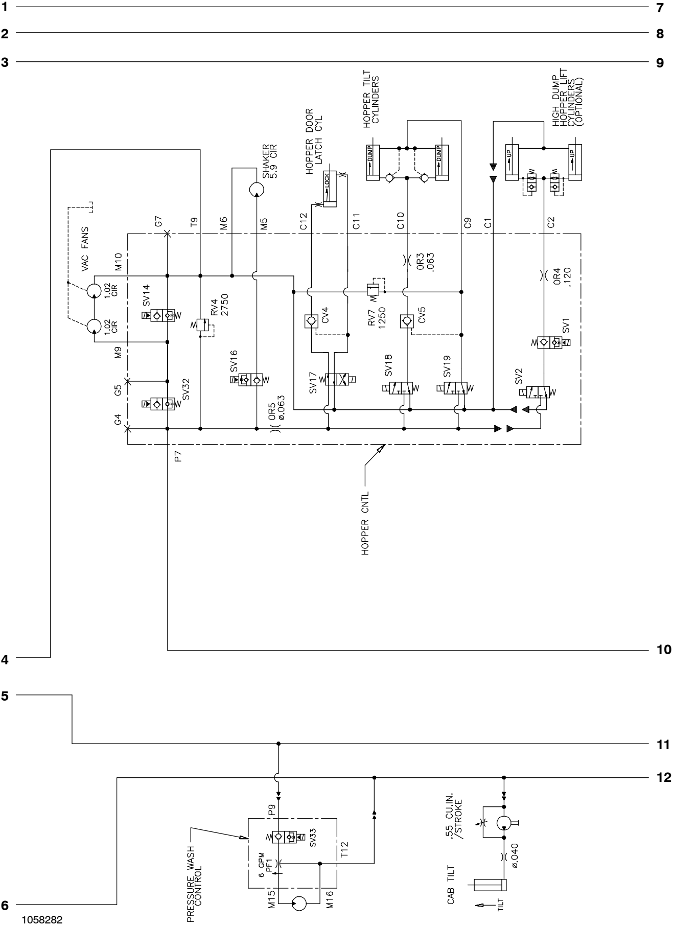
Fig. 53 - Hydraulic Schematic (008743- )
