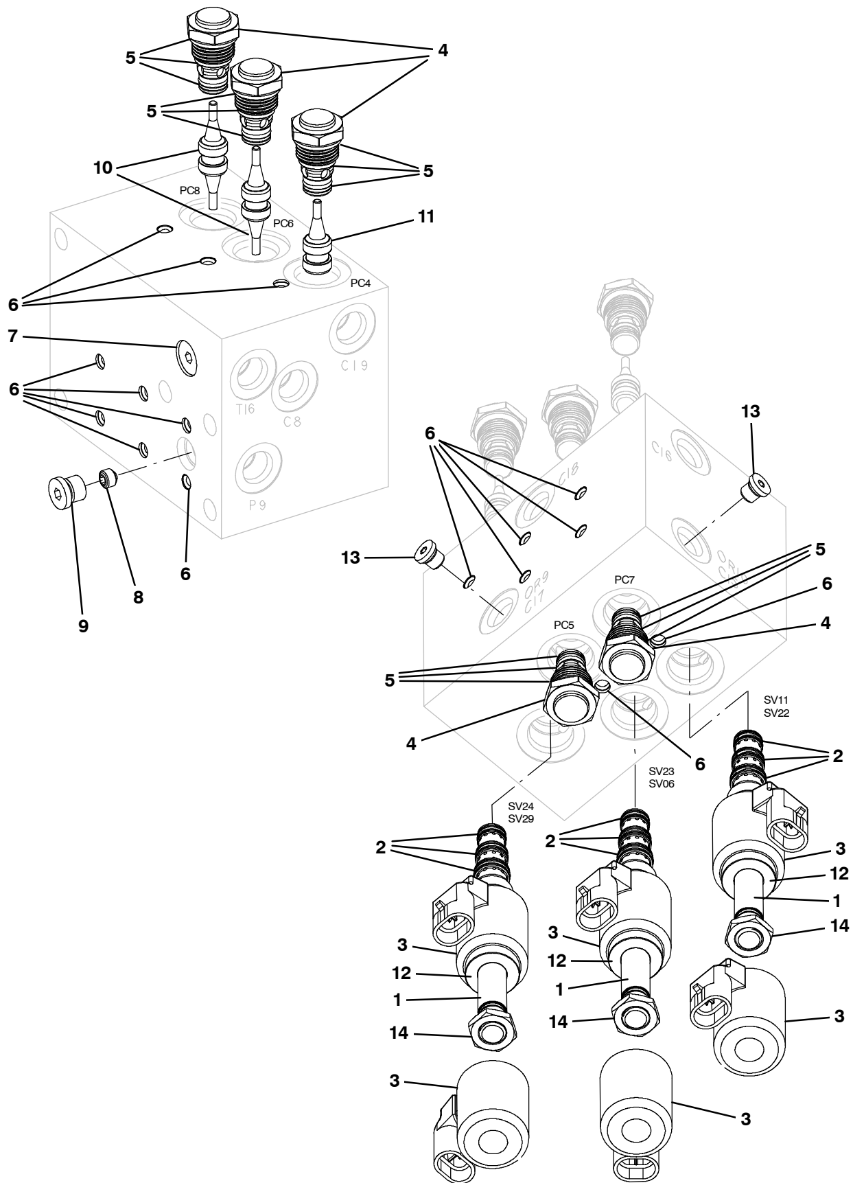
Fig. 28 - Hydraulic Solenoid Valve Breakdown, 1053648
