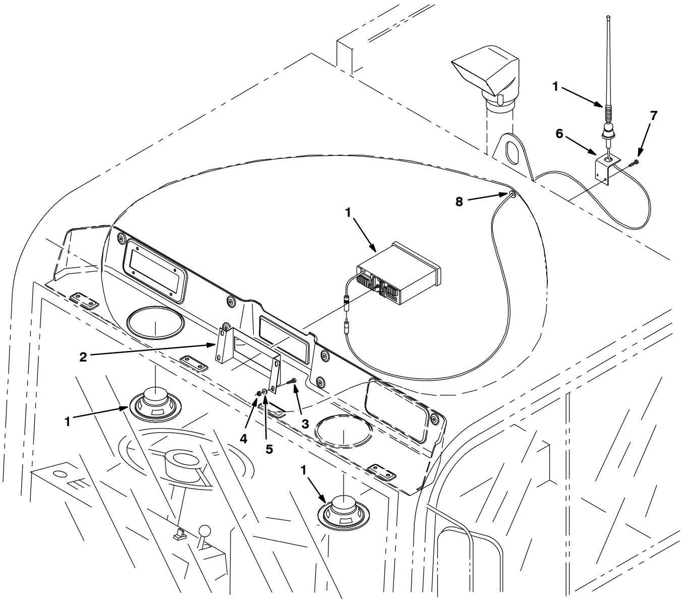
Fig. 39 - Radio Kit
