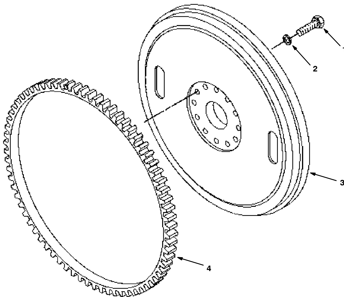
Fig. 23 - Flywheel Group
