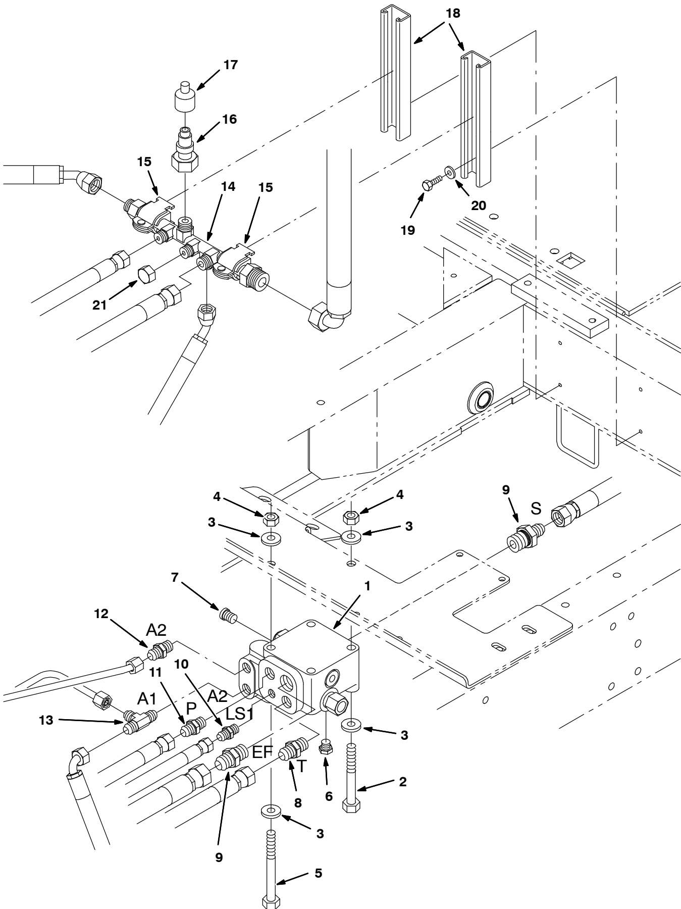
Fig. 67 - Hydraulic Manifold and Priority Valve Group
