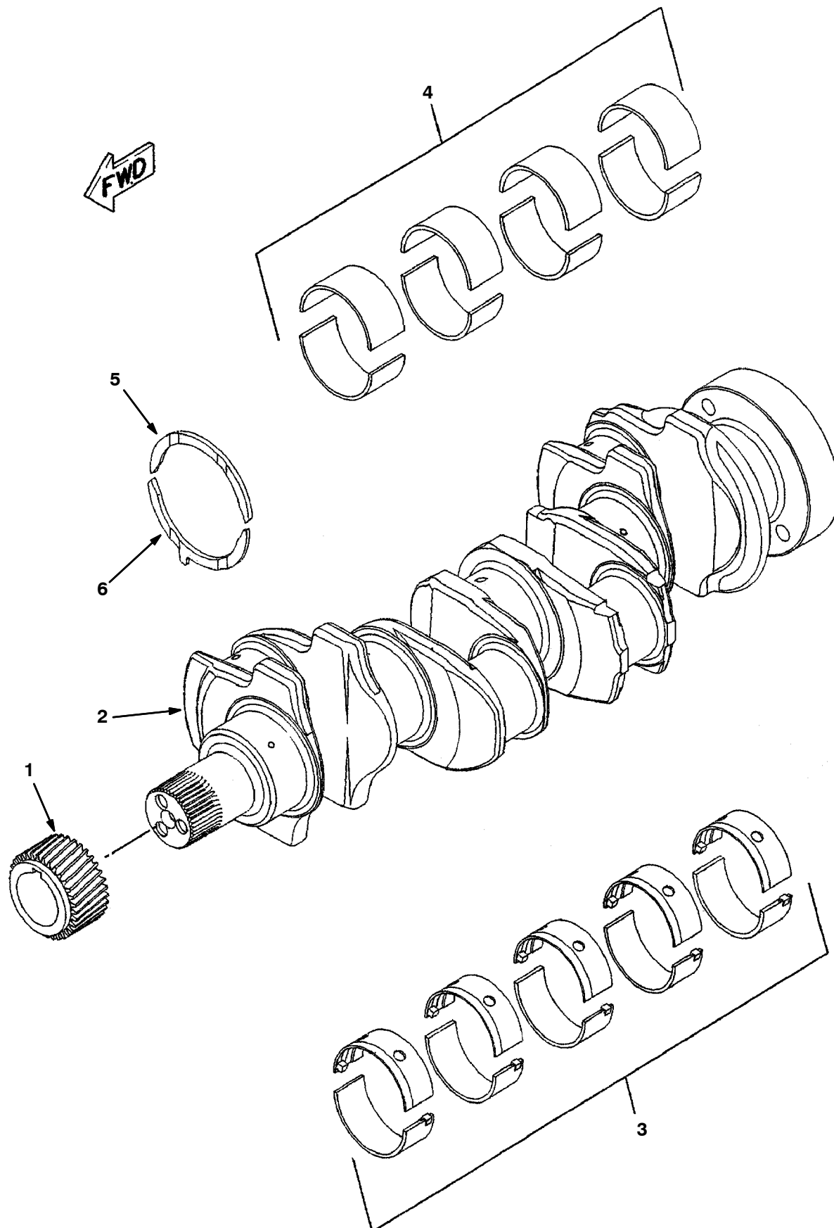
Fig. 17 - Crankshaft Group
