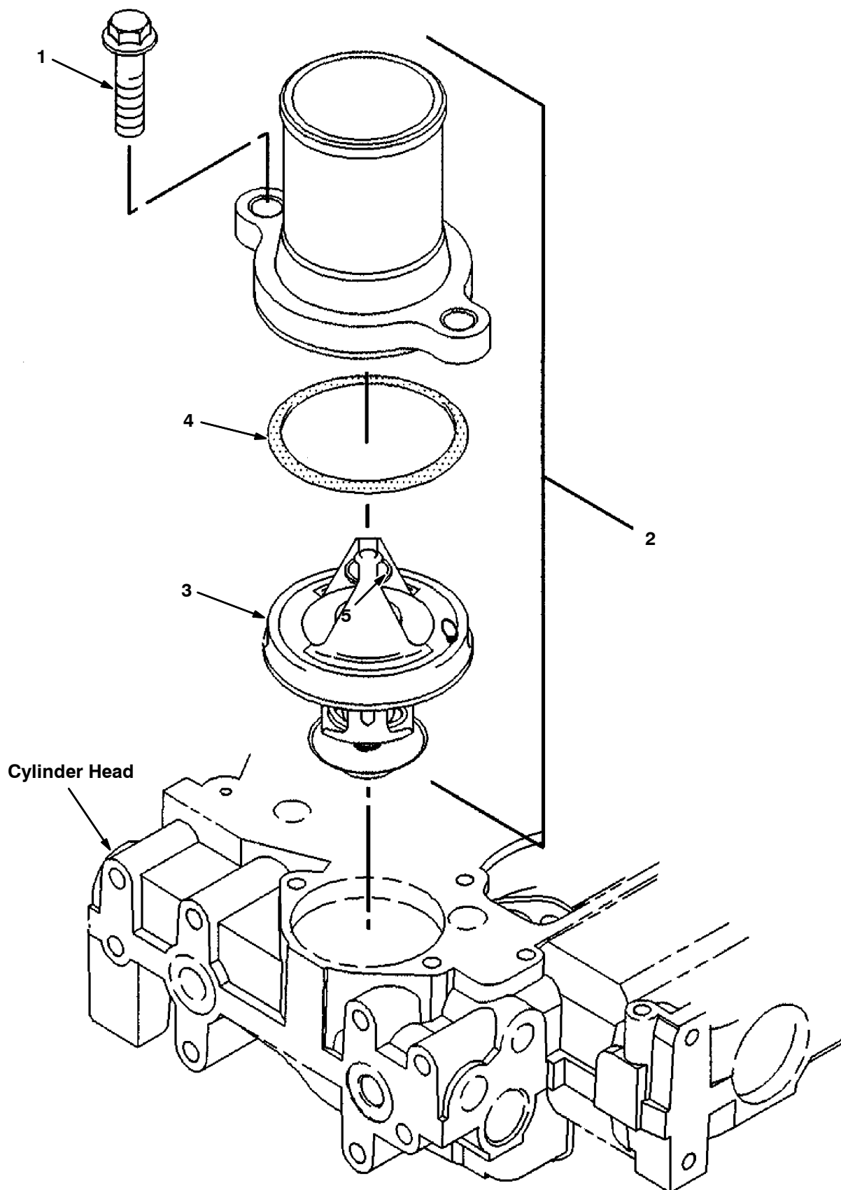
Fig. 2 - Water Connection Group
