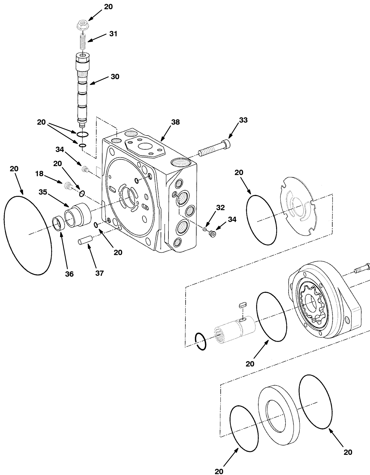
Fig. 1 - Hydraulic Piston Pump Breakdown, 767200
