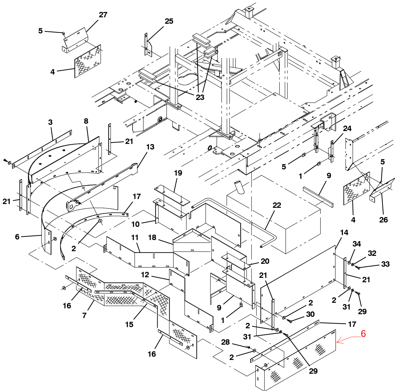
Fig. 69 - Dry Dust Control Group
