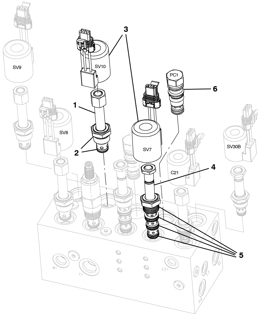
Fig. 26 - Hydraulic Solenoid Valve Breakdown, 1048792 (For Left Hand Side Brush Option)
