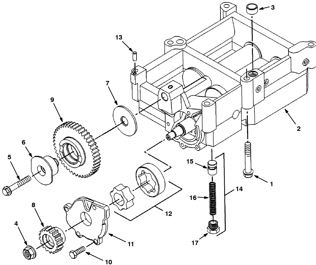
Fig. 1 - Balancer Group
