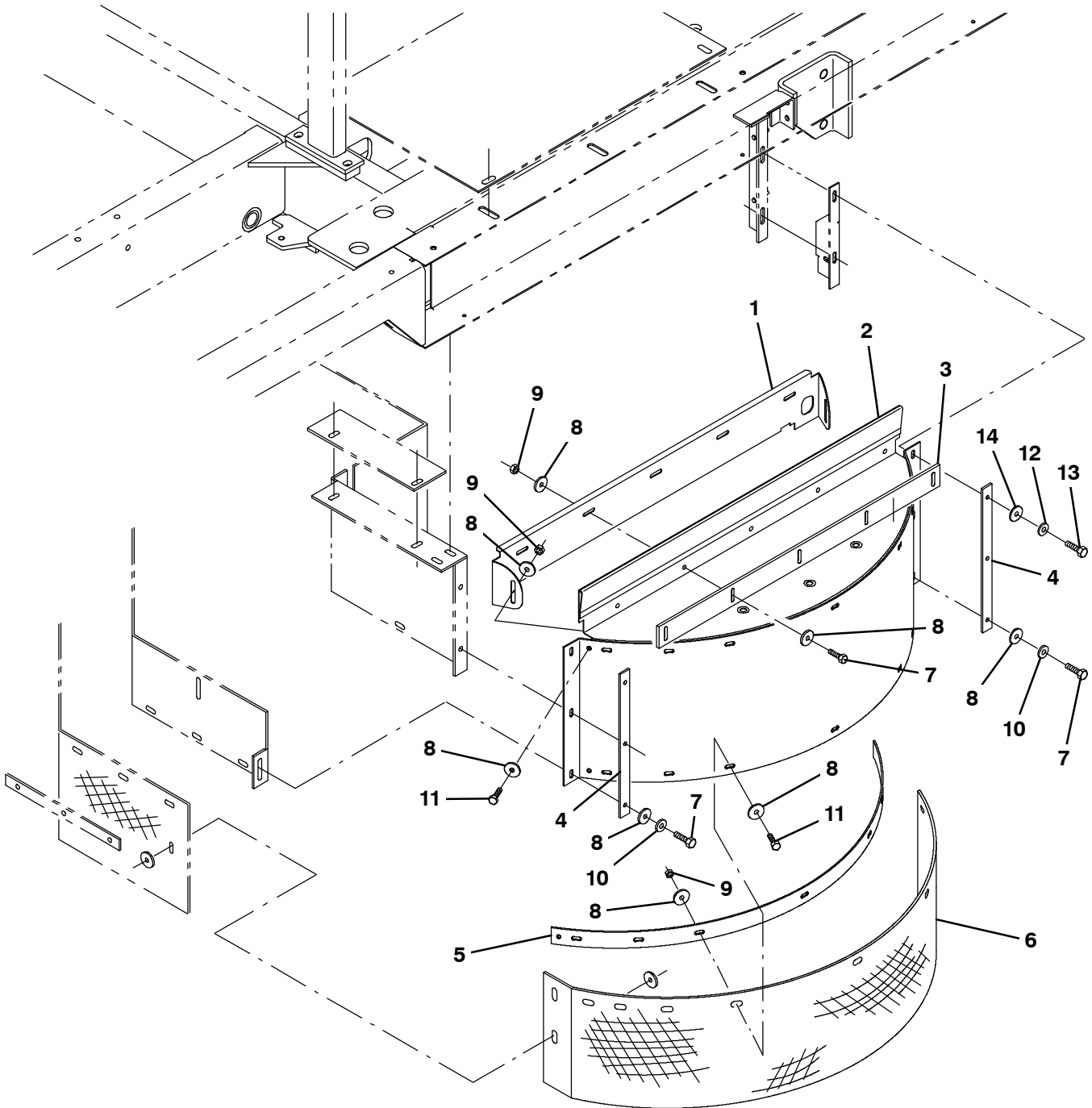
Fig. 70 - Dry Dust Control Group, Left Side Brush
