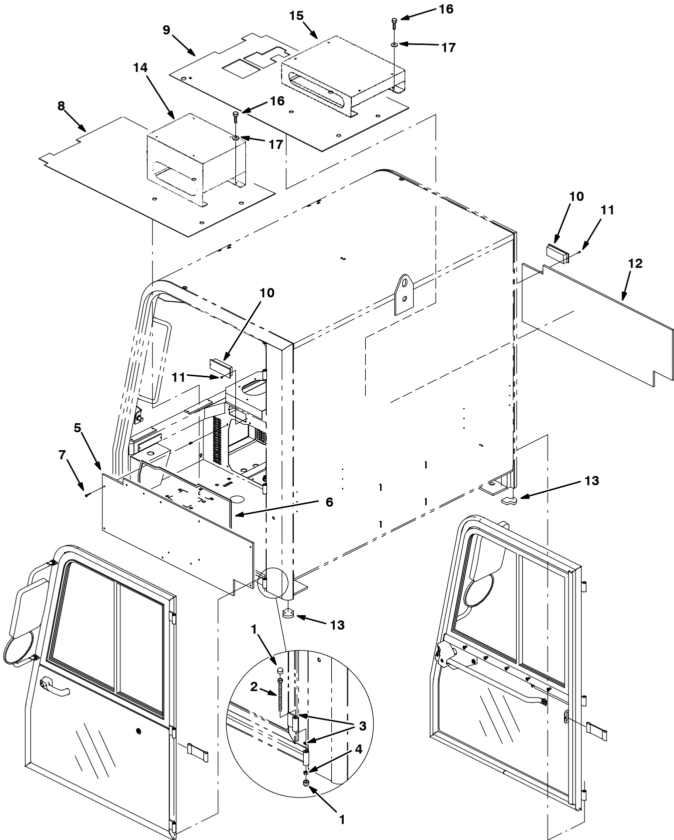
Fig. 41 - Cab Door Mount and Covers Group
