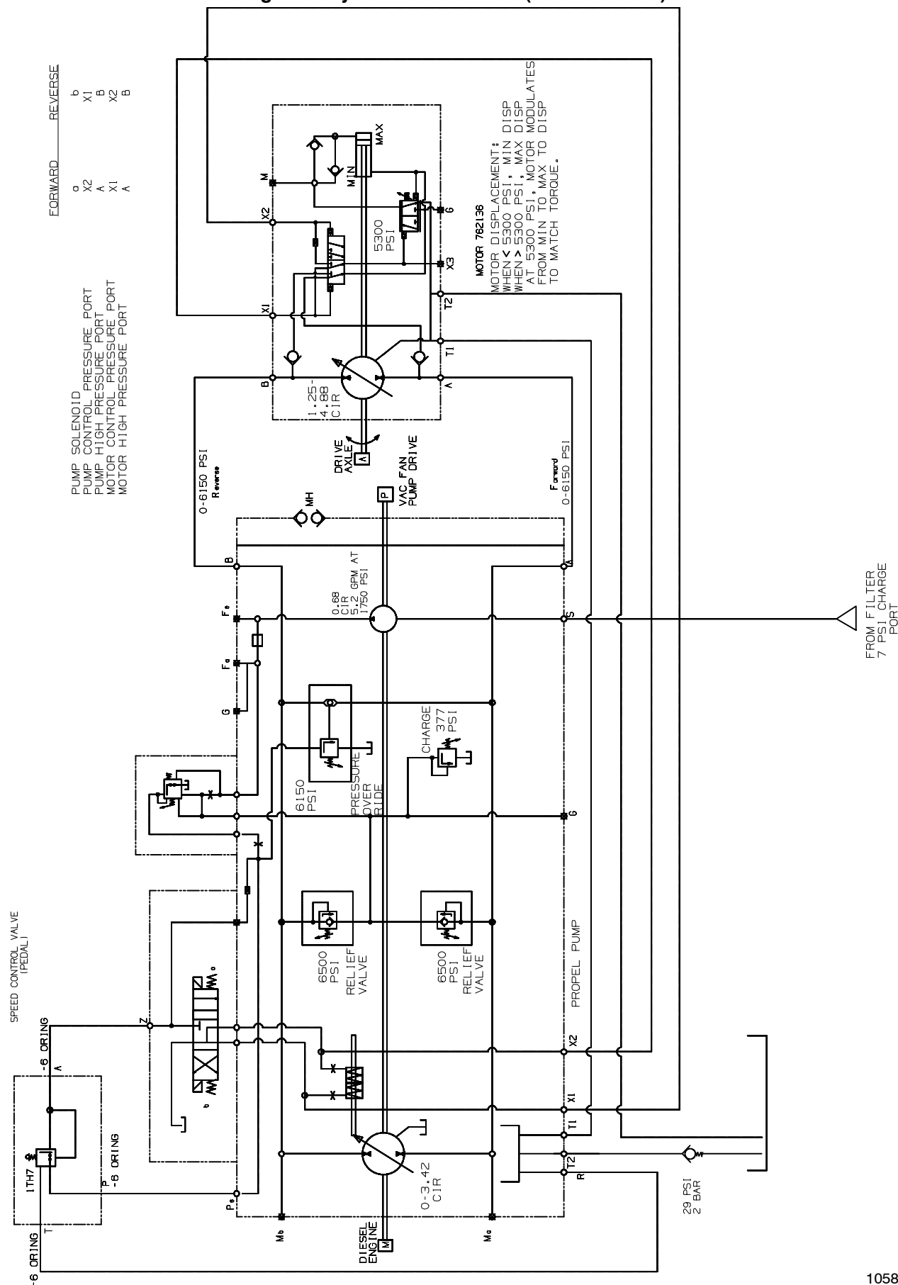
Fig. 53 - Hydraulic Schematic (008743- )
