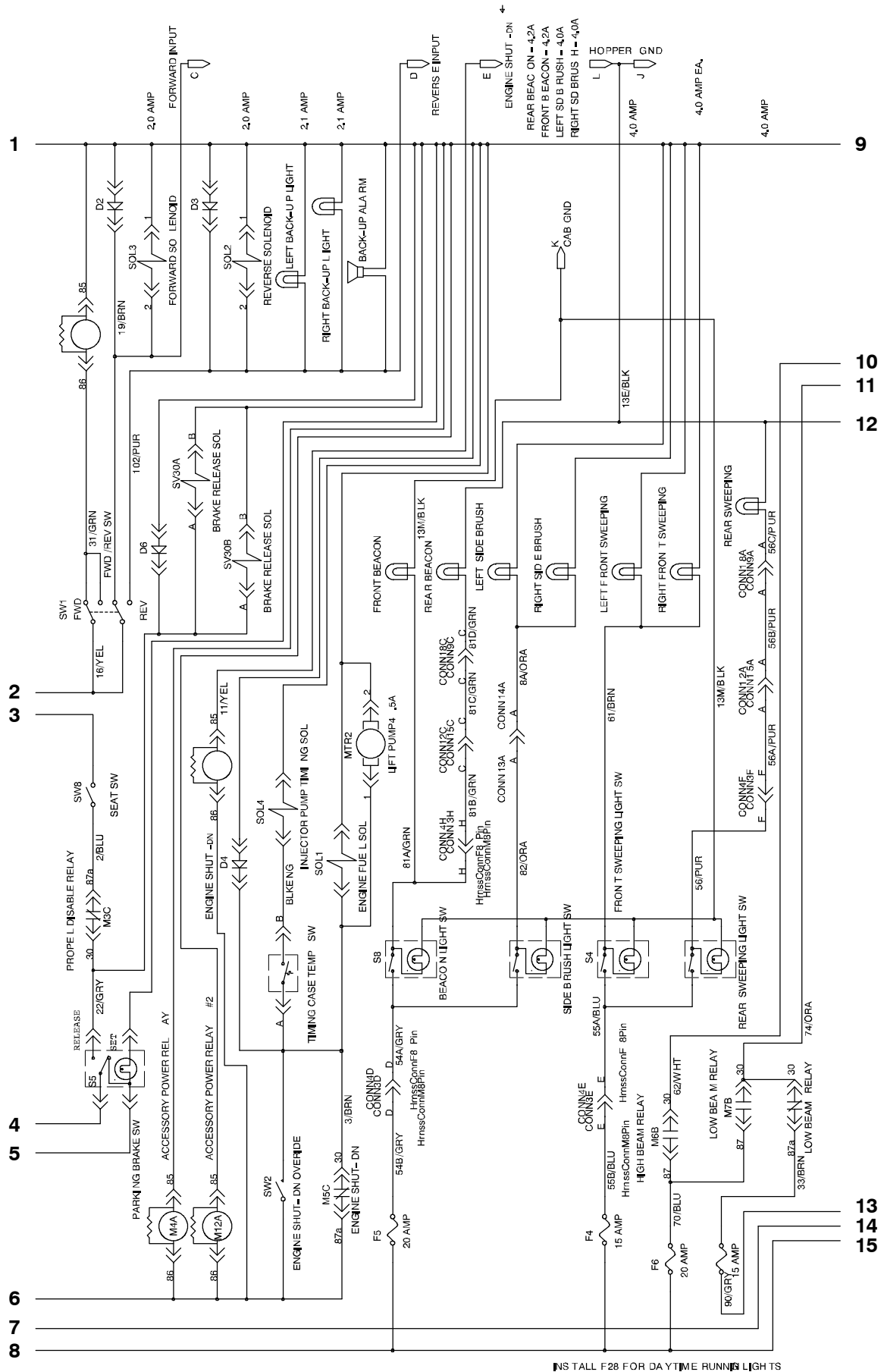
Fig. 71 - Electrical Schematic (000000-008499)
