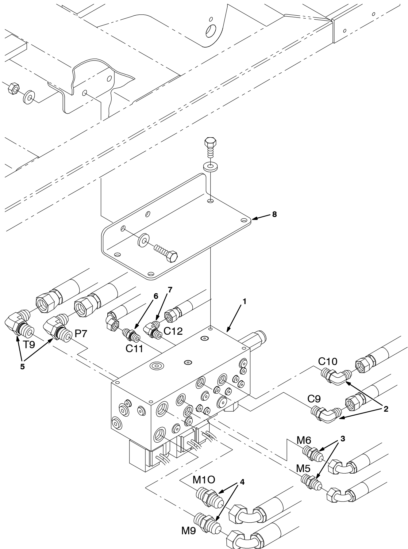
Fig. 65 - Hydraulic Hopper Control Valve Group
