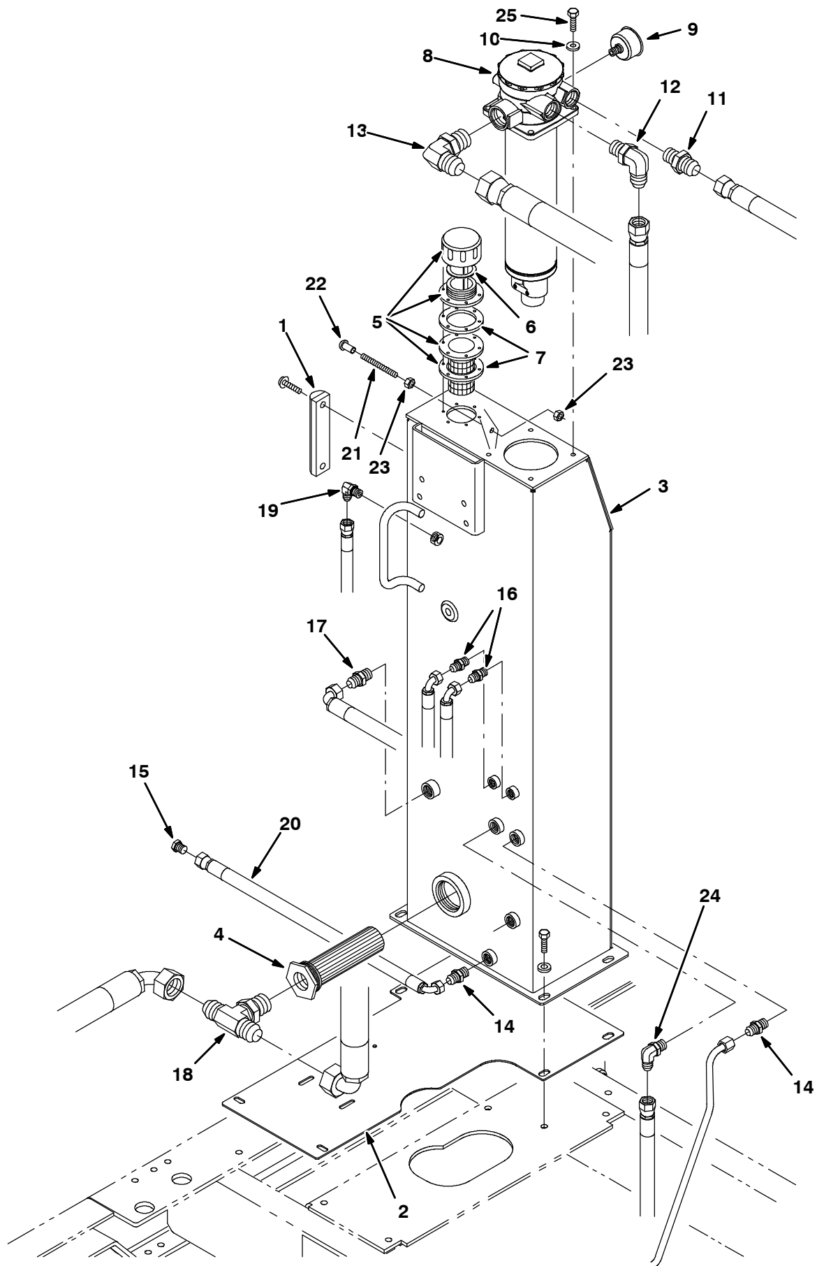
Fig. 61 - Hydraulic Reservoir Group
