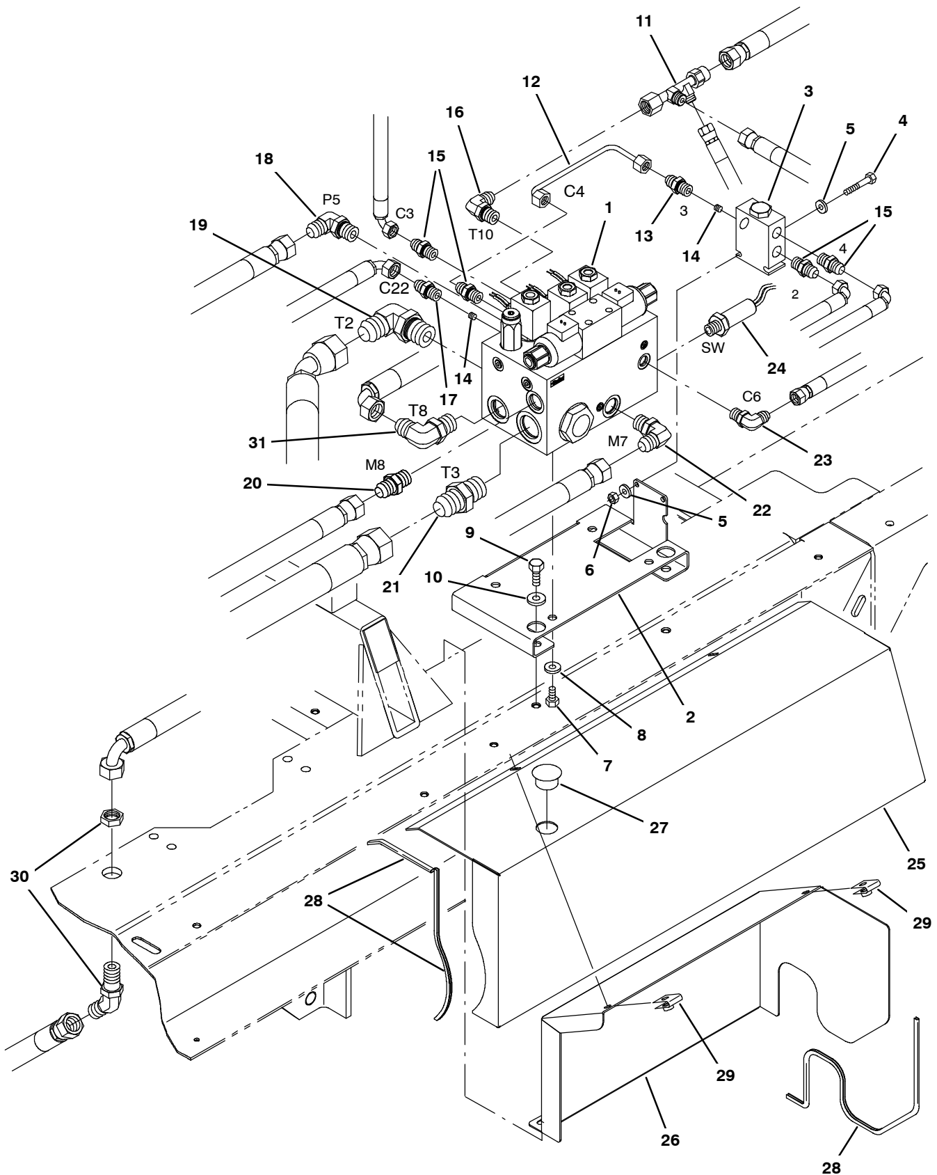
Fig. 63 - Hydraulic Main Brush/Conveyor Lift Valve Group (000000-008742)
