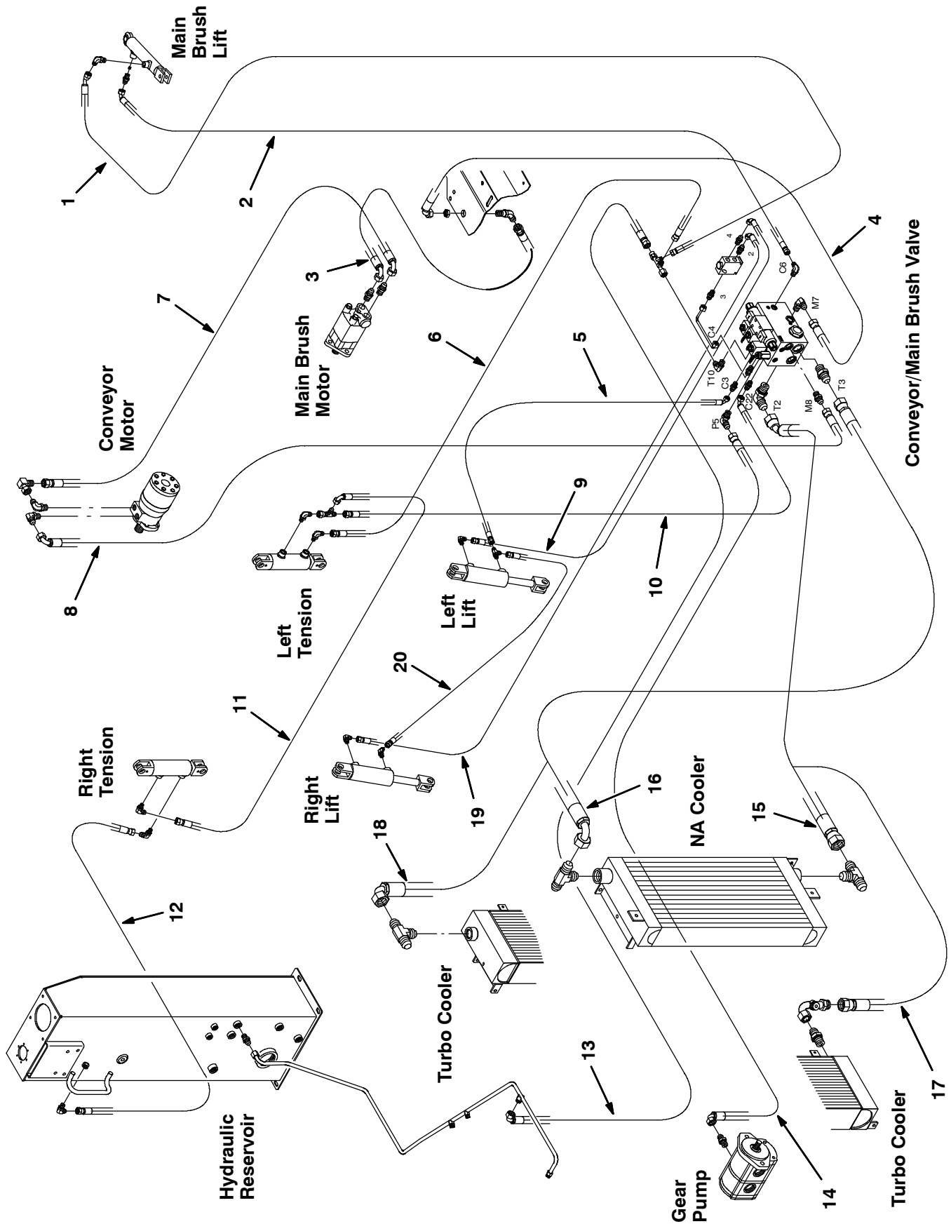
Fig. 56 - Hydraulic Hose Group, Conveyor and Main Brush (000000-008742)
