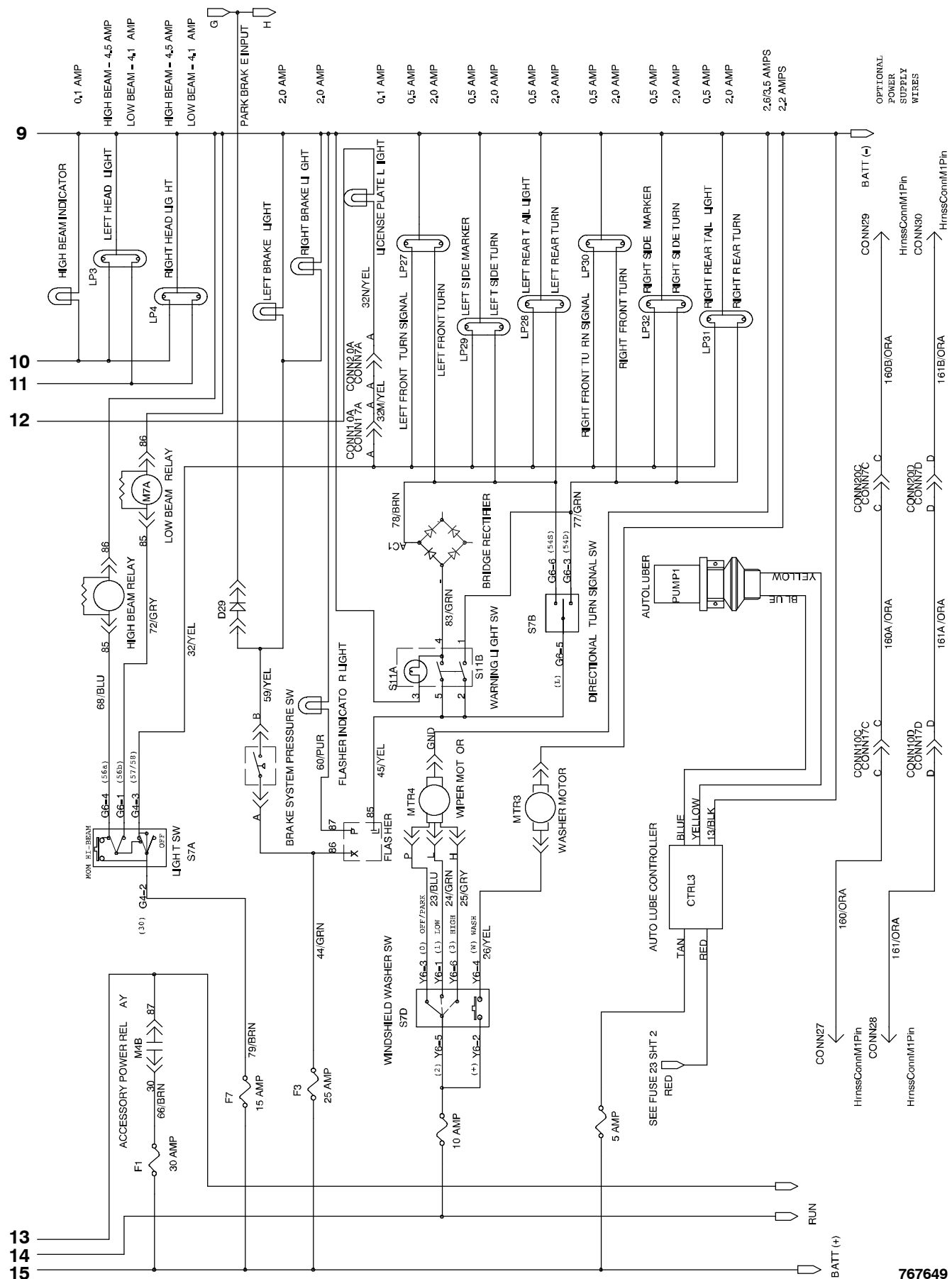
Fig. 71 - Electrical Schematic (000000-008499)
