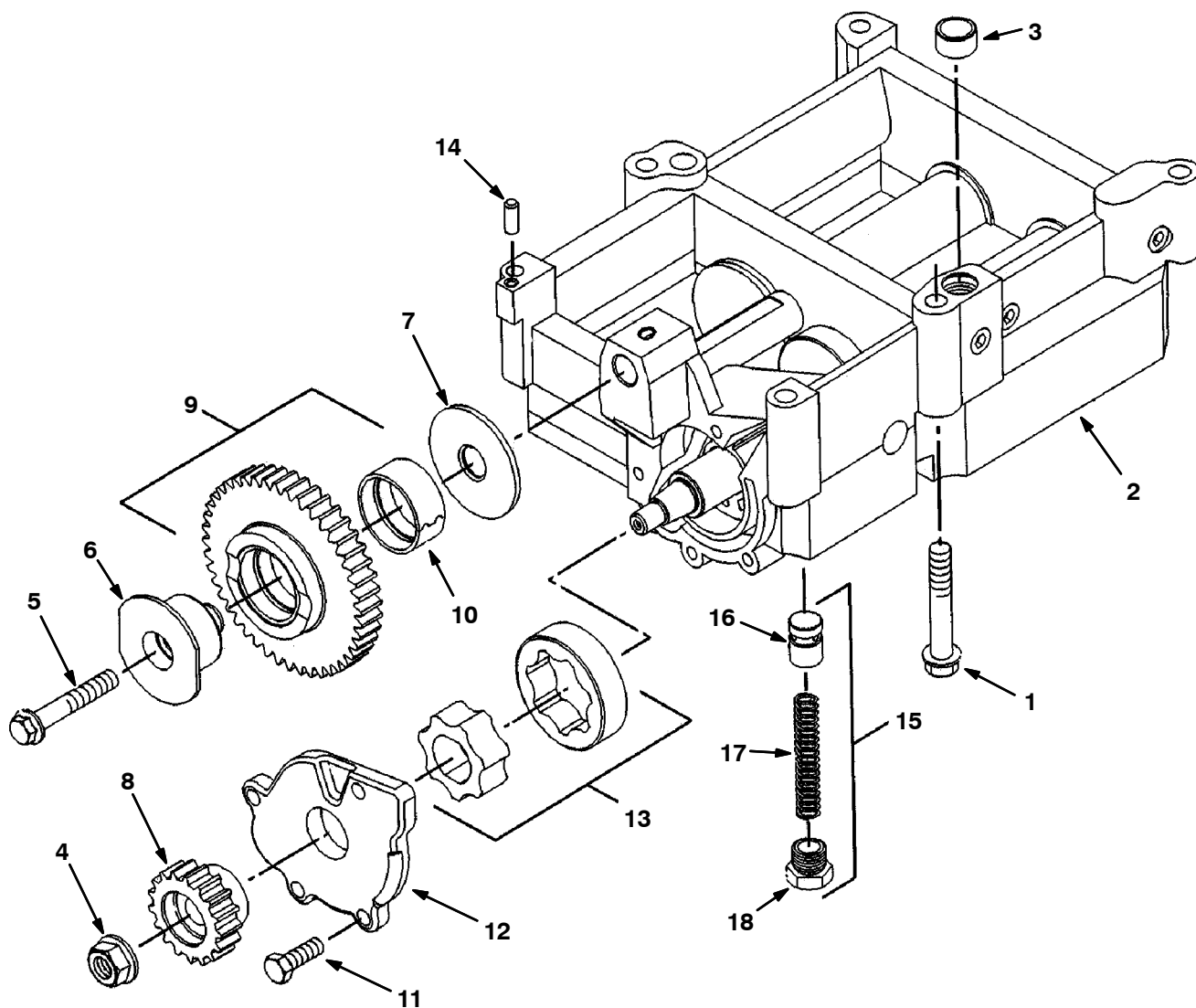
Fig. 1 - Balancer Group
