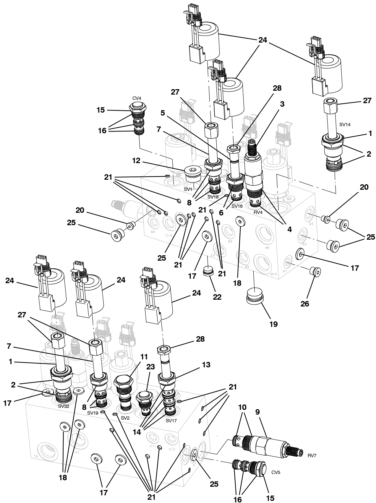
Fig. 22 - Hydraulic Solenoid Valve Breakdown, 1053642
