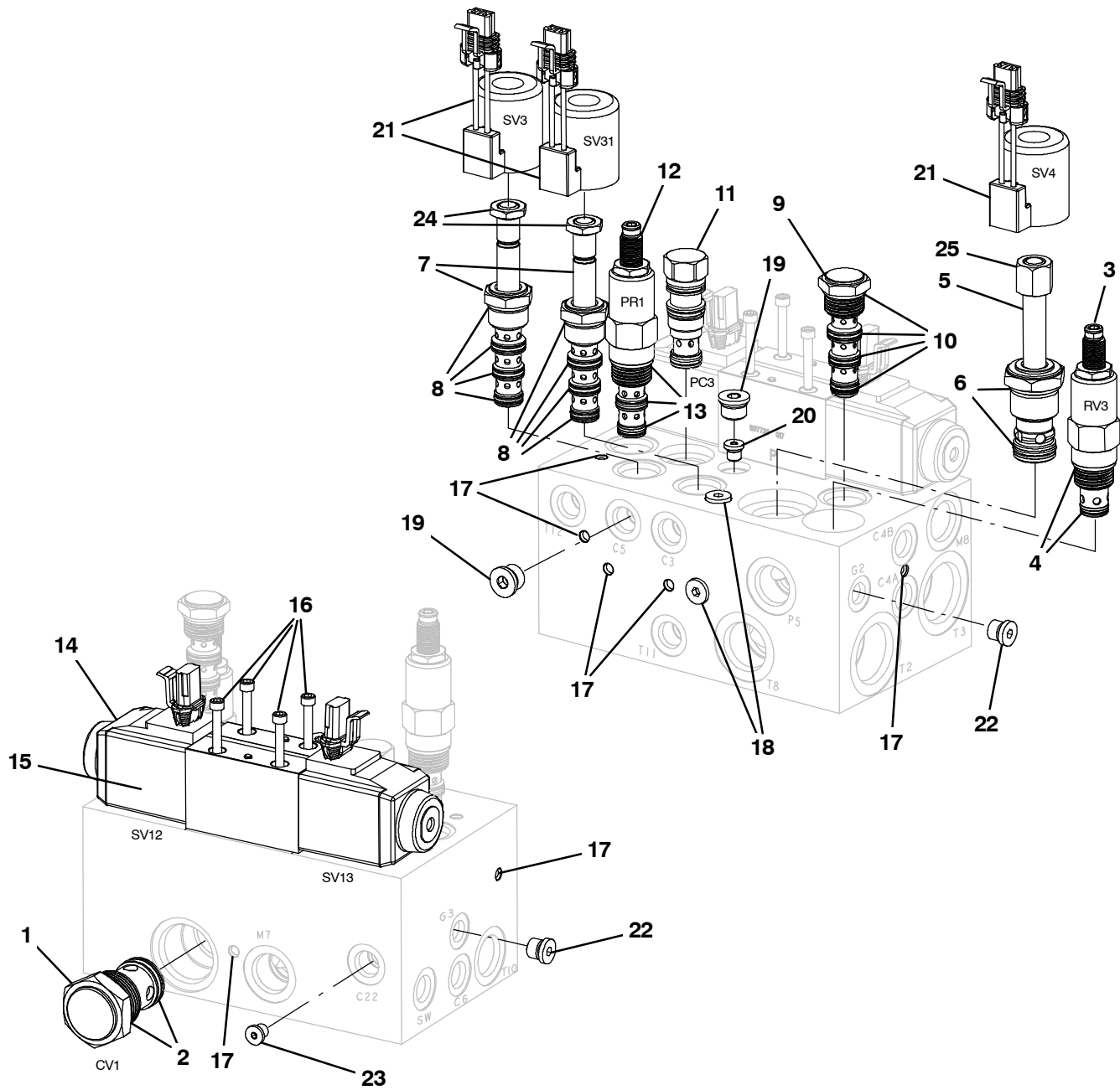
Fig. 24 - Hydraulic Solenoid Valve Breakdown, 1053650
