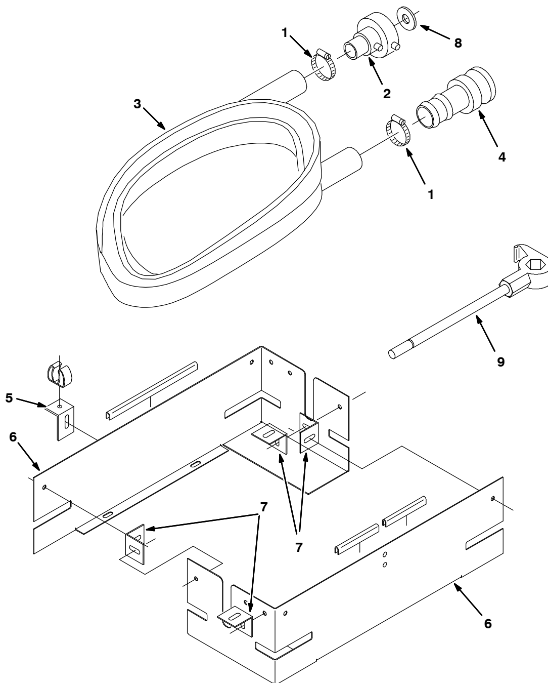
Fig. 31 - Hydrant Hose Group
