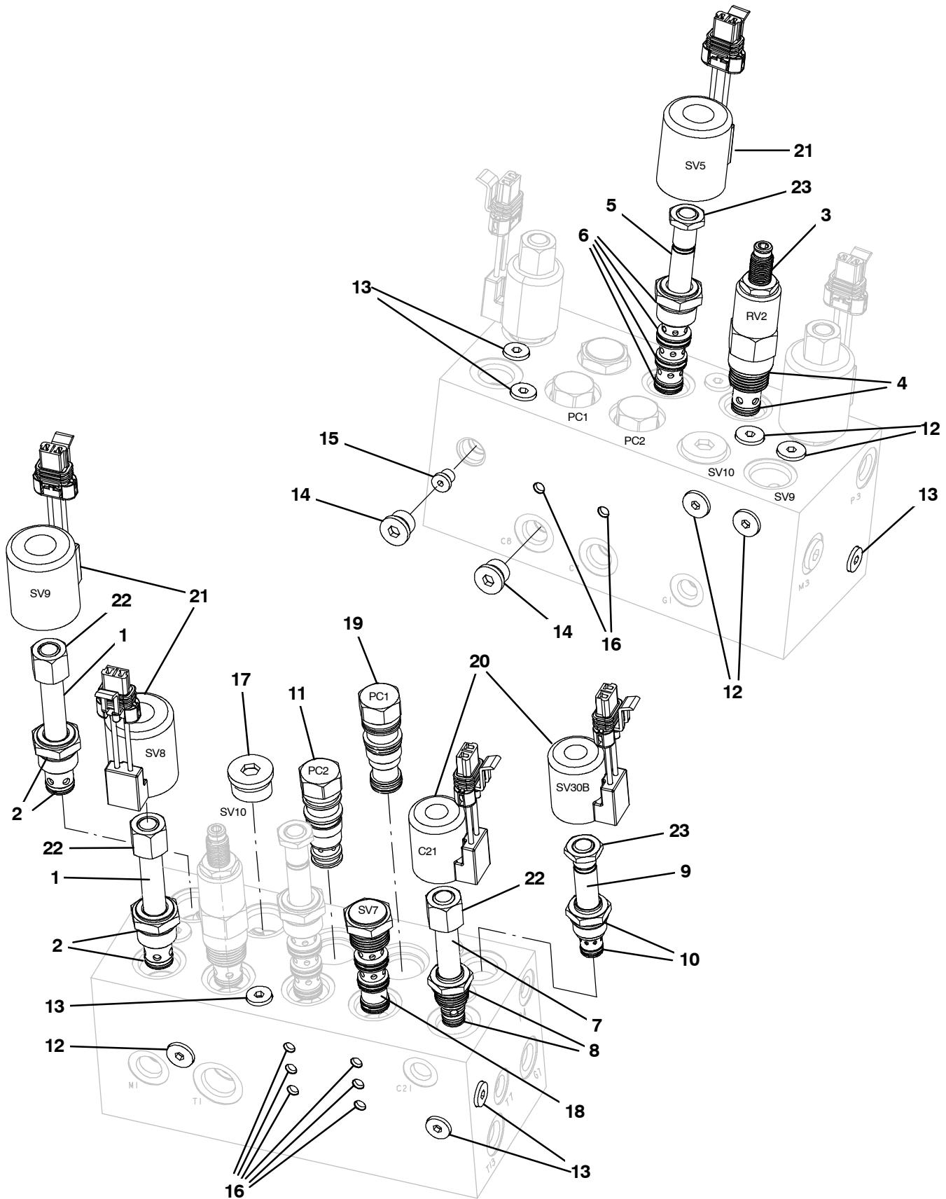
Fig. 25 - Hydraulic Solenoid Valve Breakdown, 1048792
