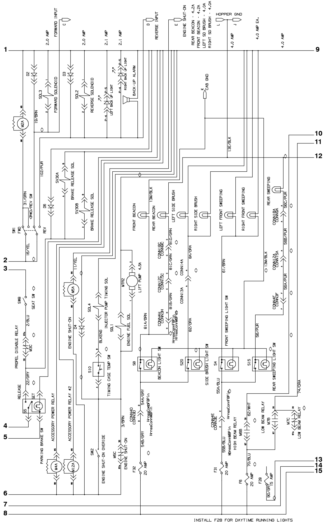
Fig. 72 - Electrical Schematic (008500- )
