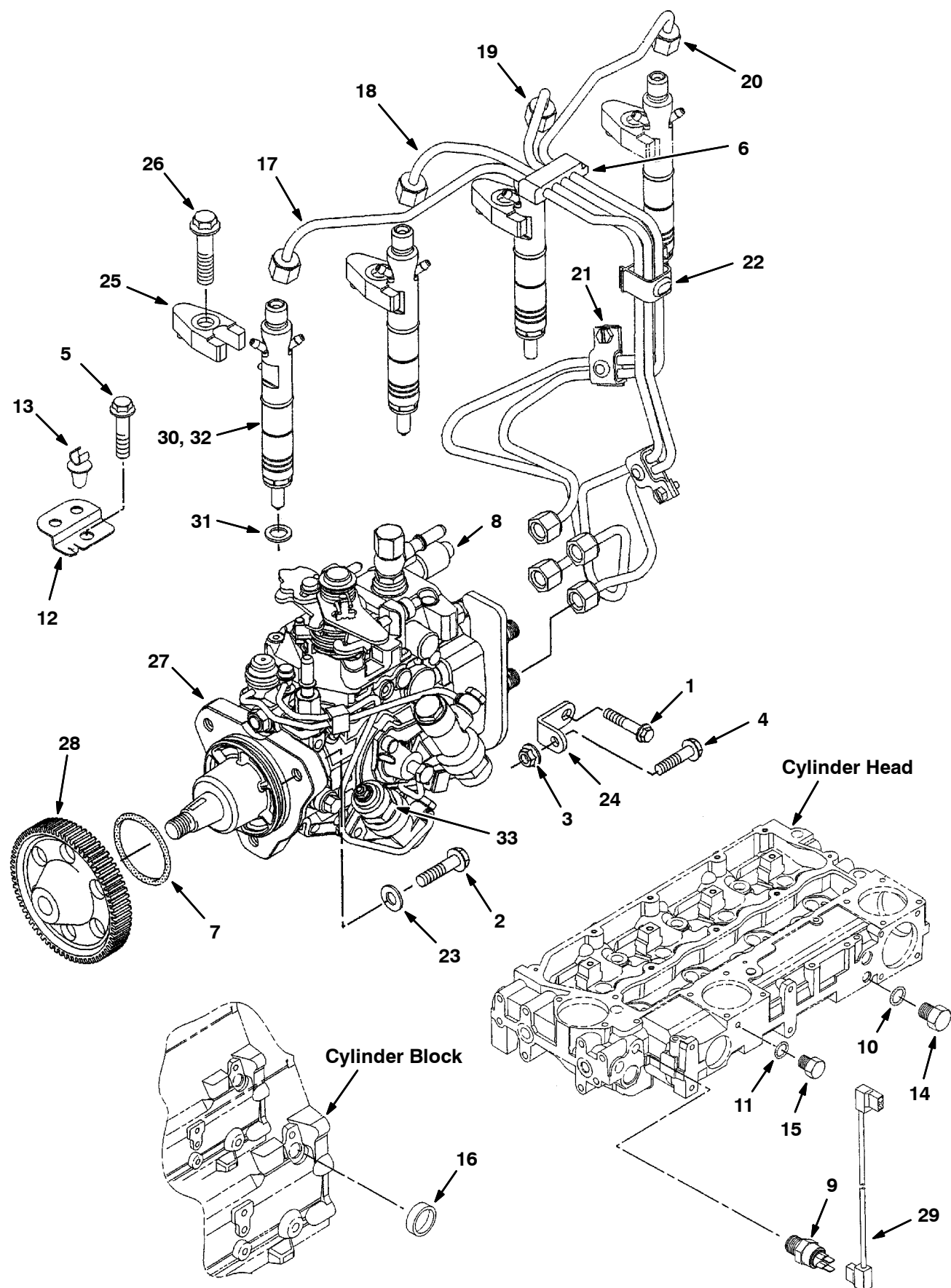
Fig. 18 - Fuel Injection Pump Group
