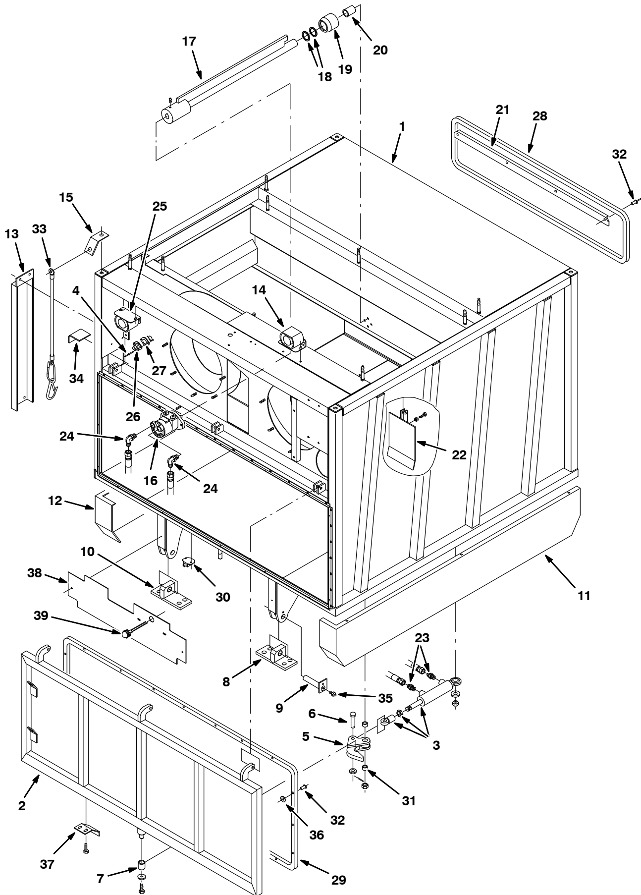
Fig. 34 - Hopper Group
