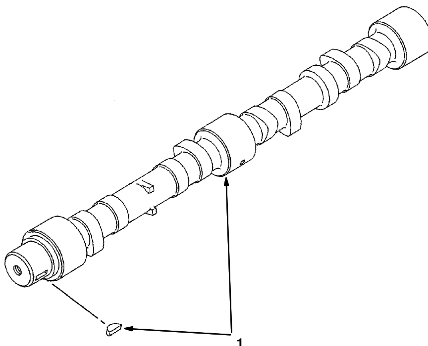
Fig. 19 - Camshaft Group
