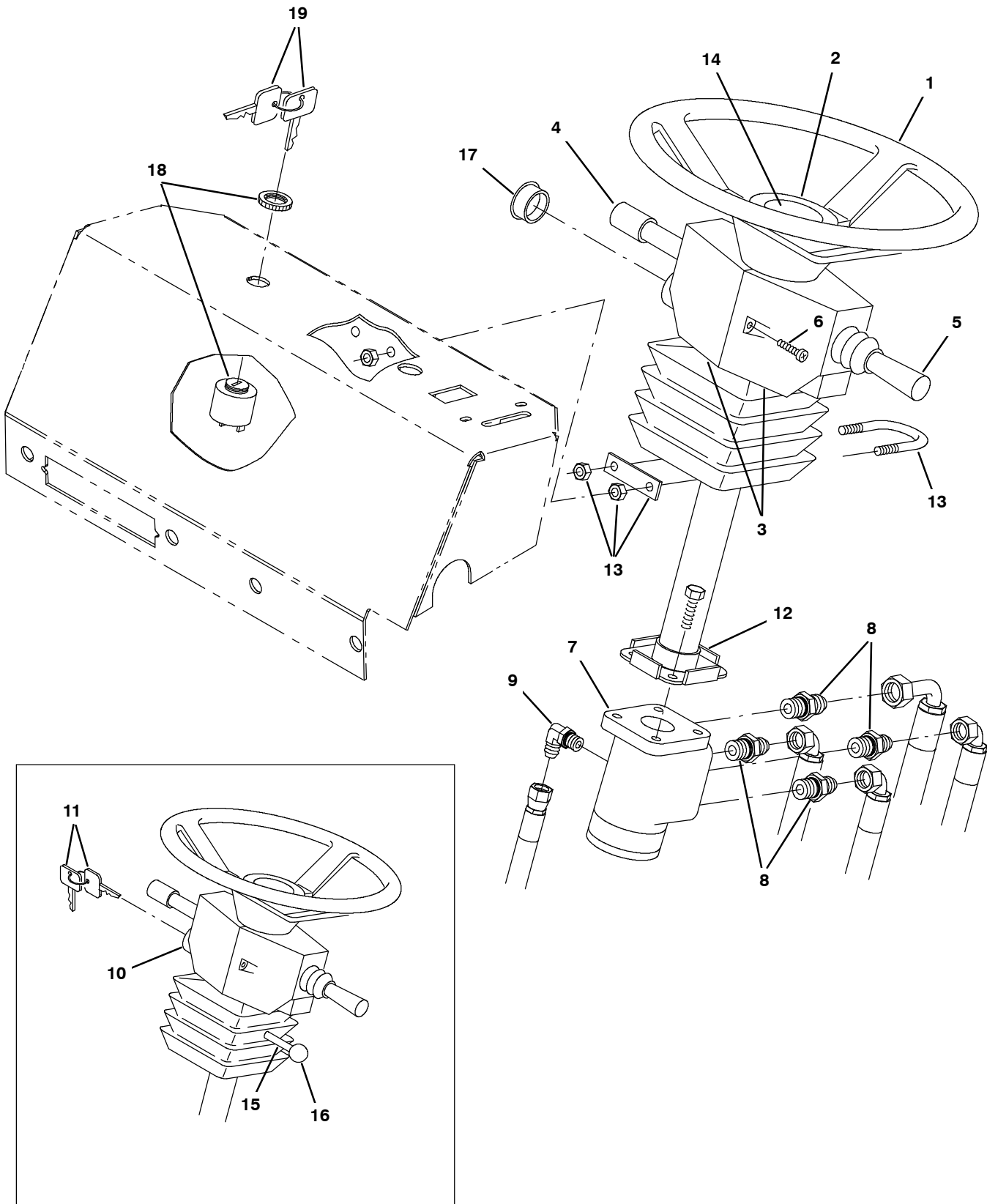
Fig. 50 - Steering Wheel Group
