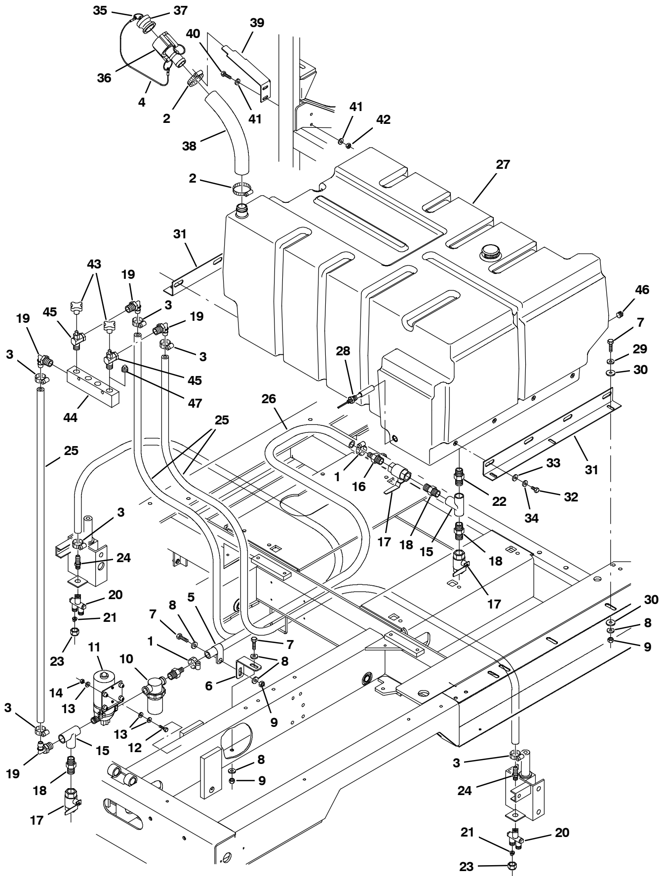
Fig. 68 - Water Tank Group
