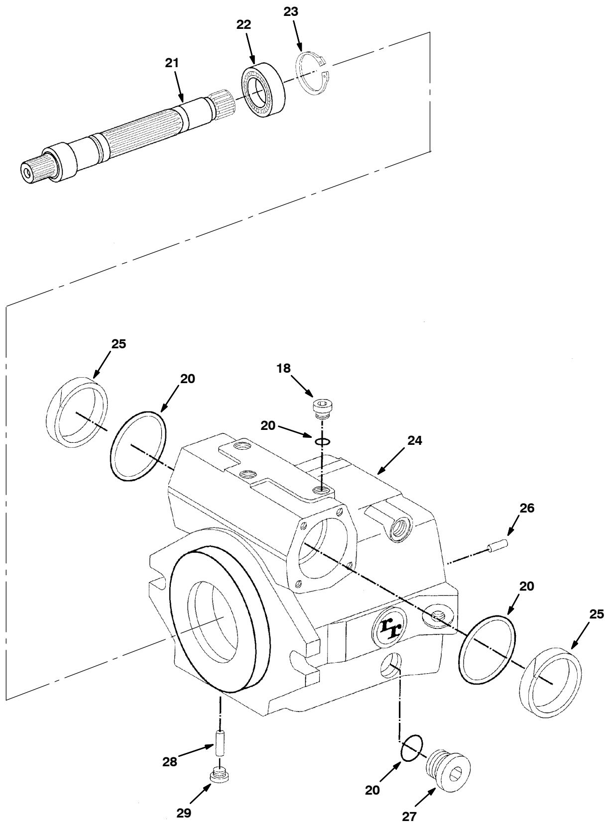
Fig. 1 - Hydraulic Piston Pump Breakdown, 767200
