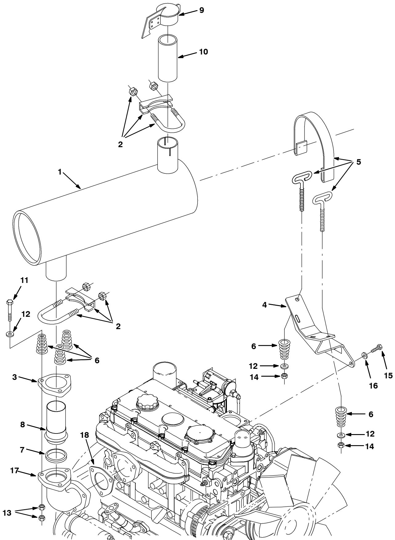
Fig. 21 - Engine Muffler Group, NA (000000-008499)
