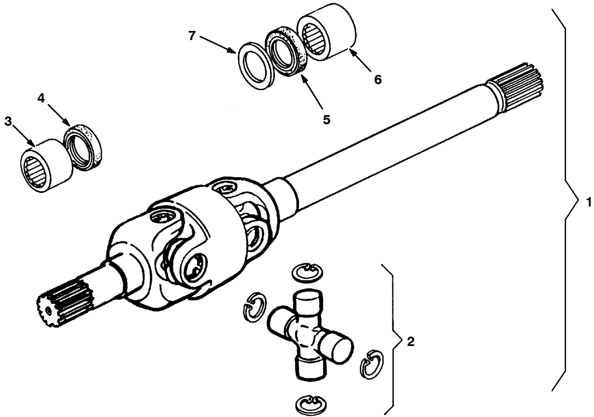
Fig. 9 - Axle CV Joint Breakdown, Front
