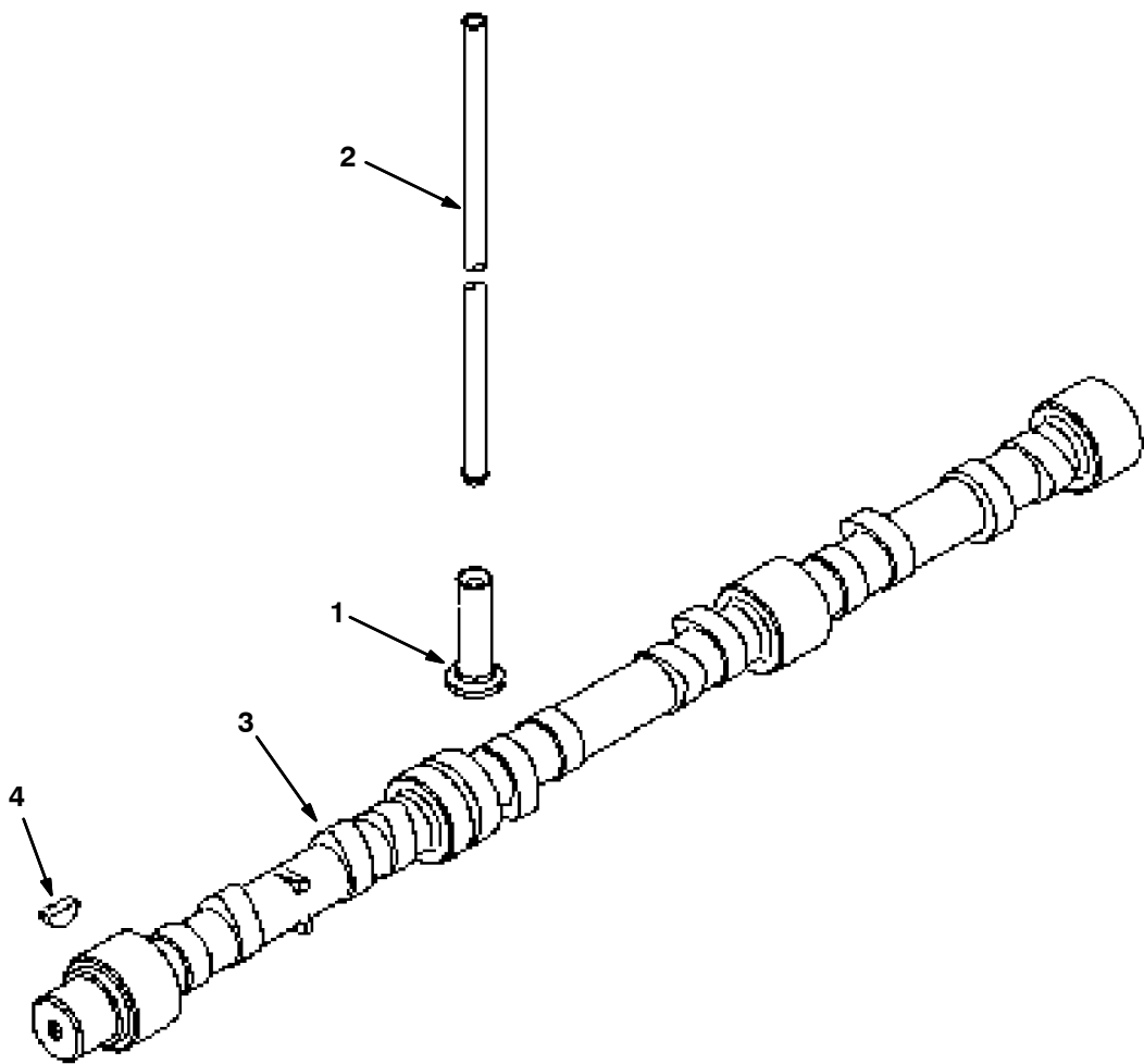
Fig. 16 - Camshaft Group
