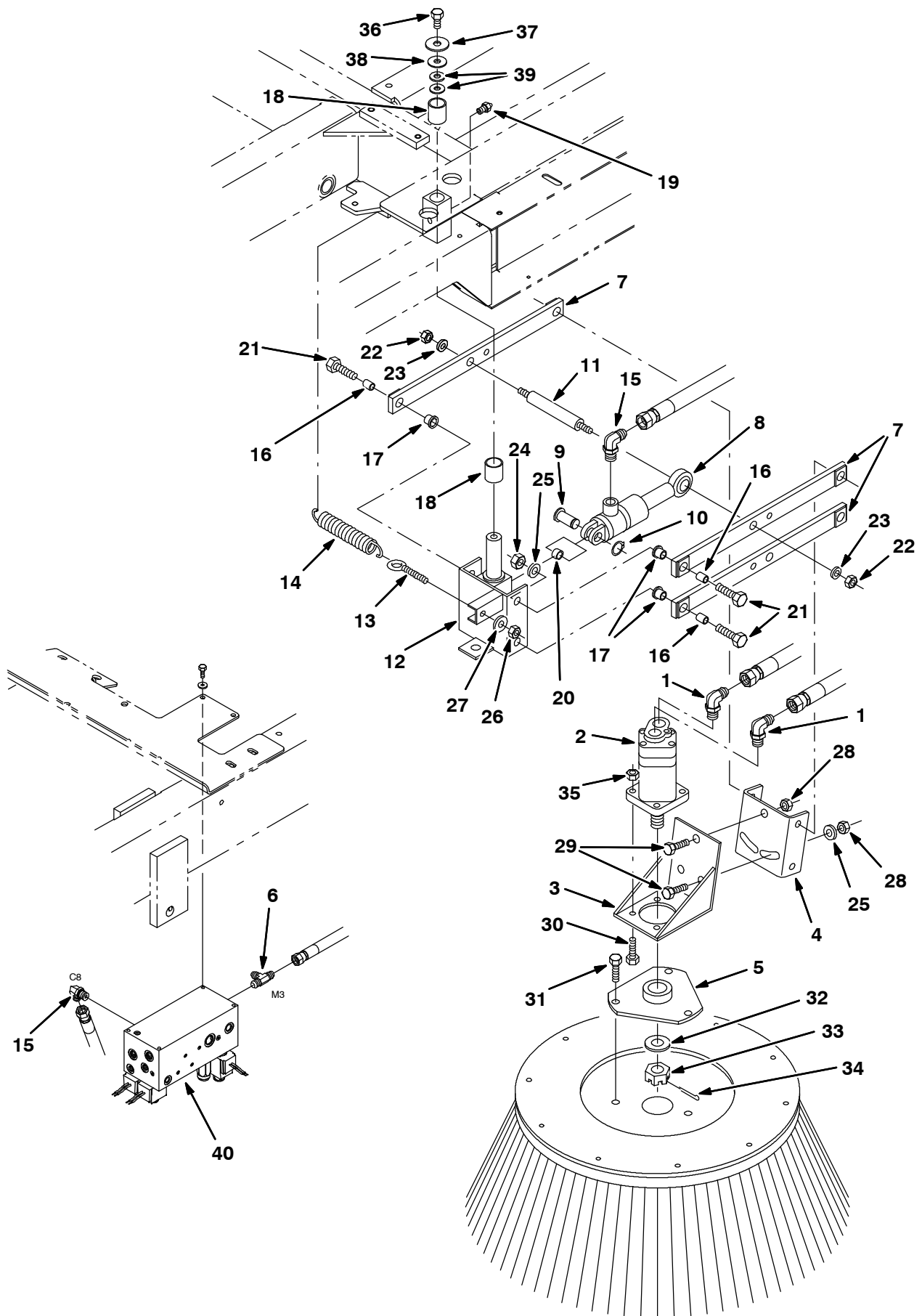
Fig. 4 - Left Side Brush Group
