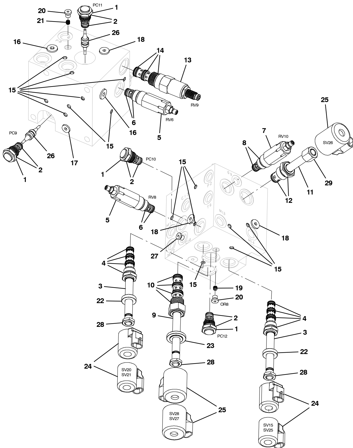
Fig. 27 - Hydraulic Solenoid Valve Breakdown, 1053645
