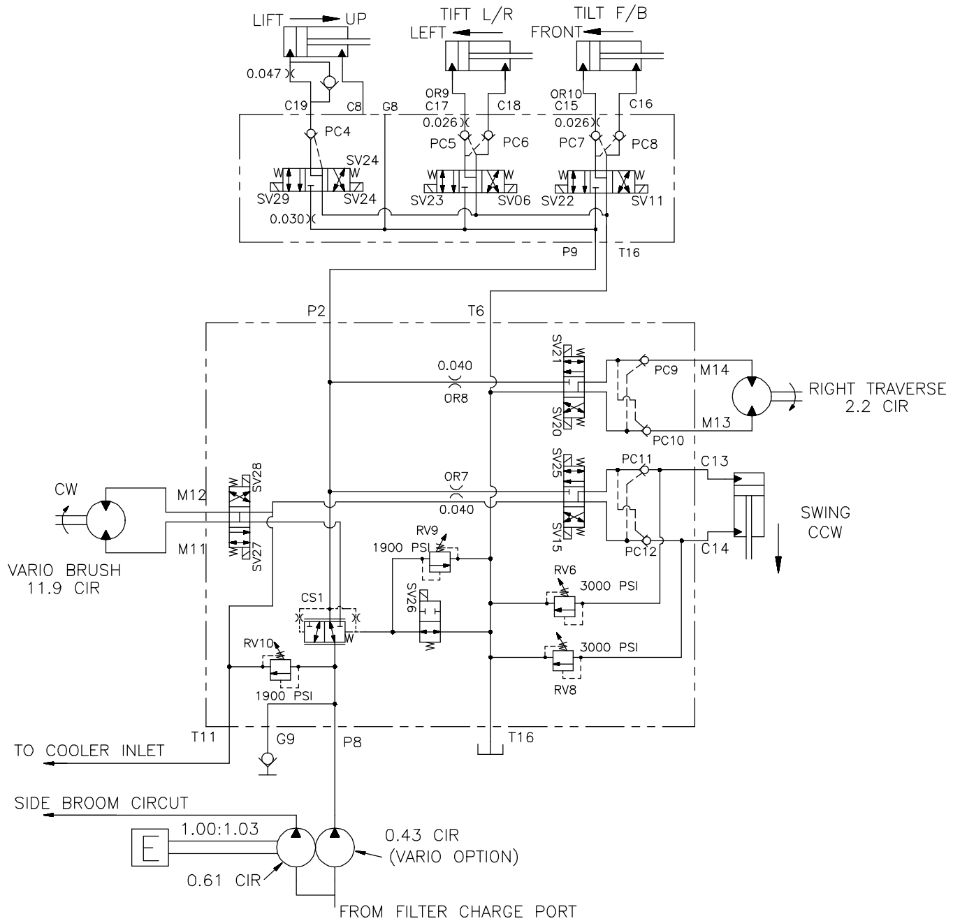
Fig. 52 - Hydraulic Schematic (000000-008742)
