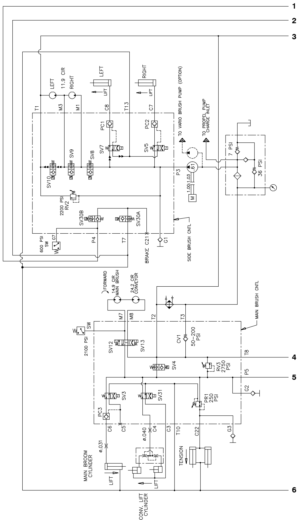
Fig. 52 - Hydraulic Schematic (000000-008742)
