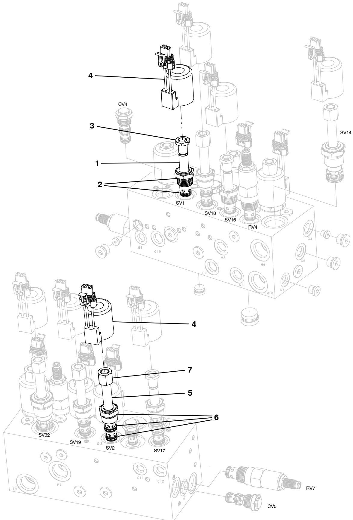
Fig. 23 - Hydraulic Solenoid Valve Breakdown, 1053642 (For High Dump Hopper Lift Option)
