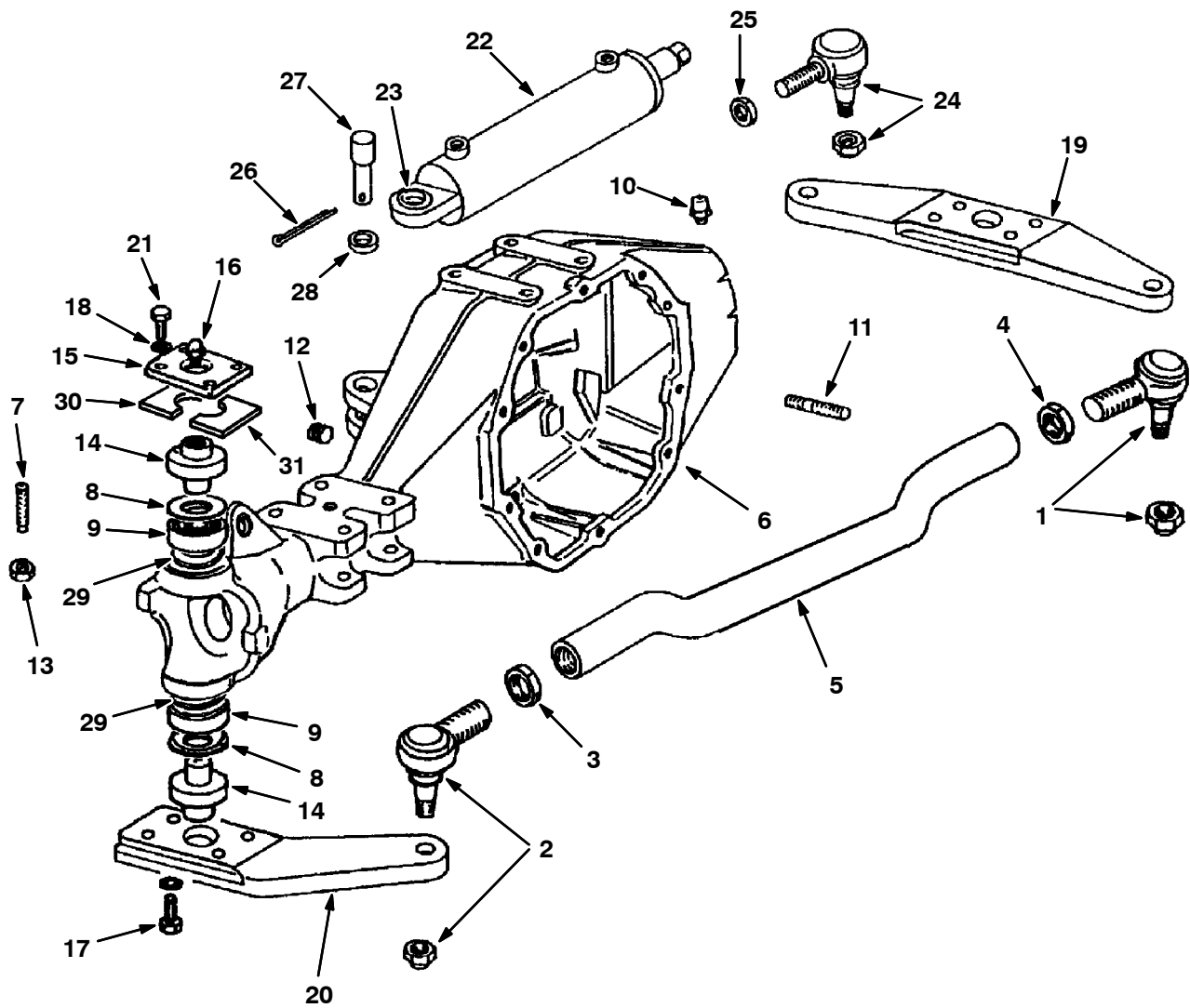
Fig. 5 - Axle And Spindle Breakdown, Front
