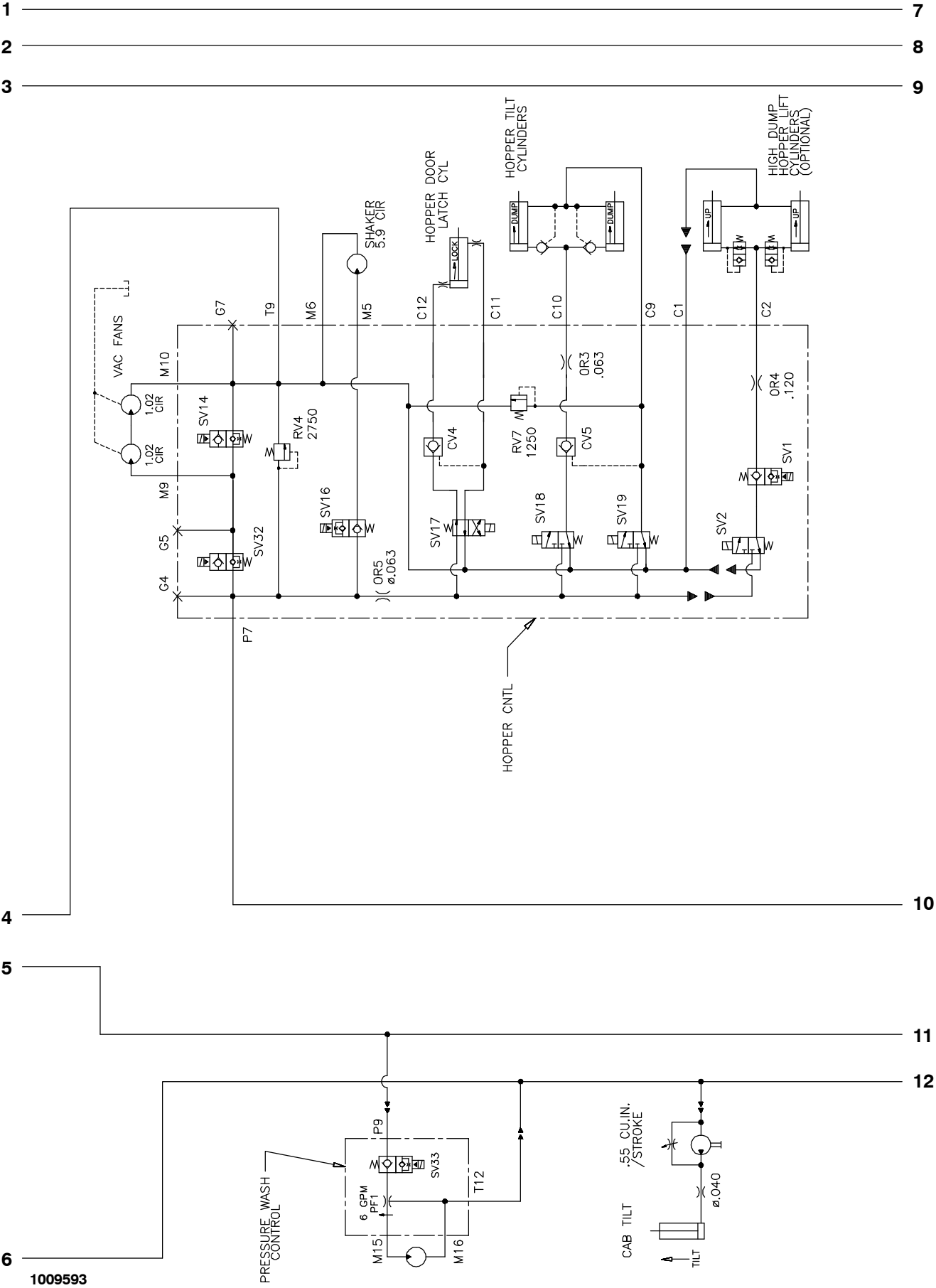
Fig. 52 - Hydraulic Schematic (000000-008742)
