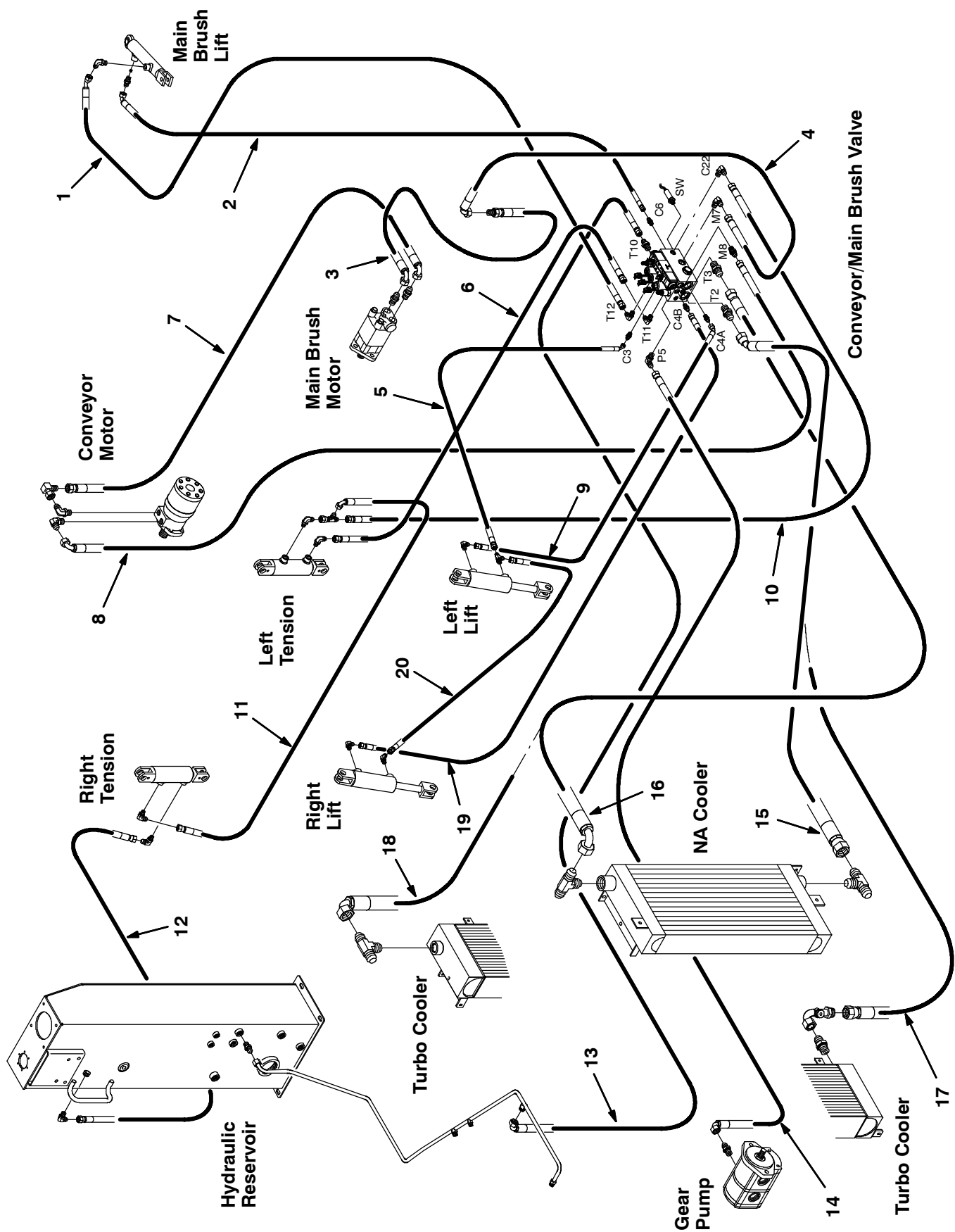
Fig. 57 - Hydraulic Hose Group, Conveyor and Main Brush (008743- )
