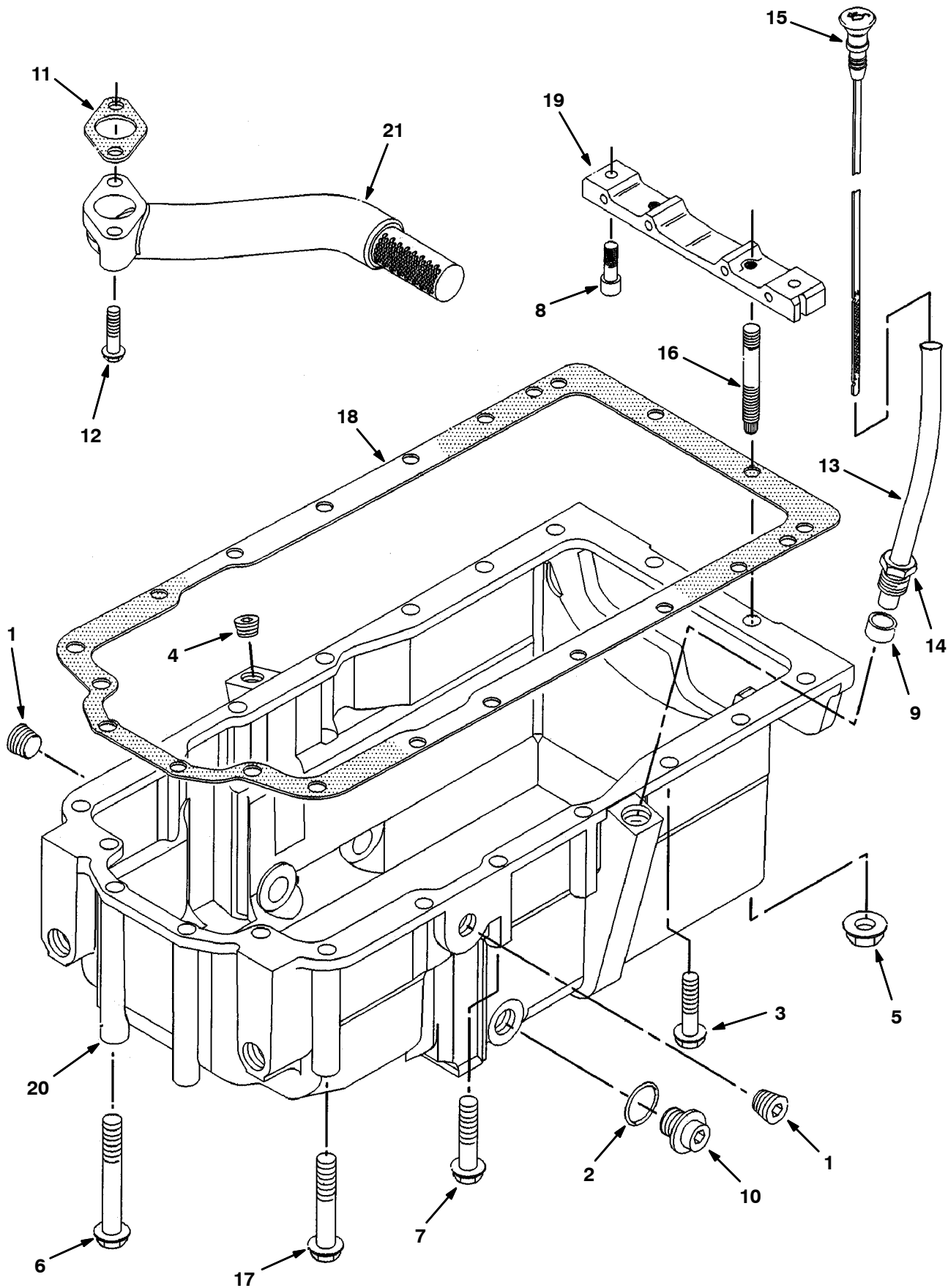
Fig. 16 - Oil Pan Group
