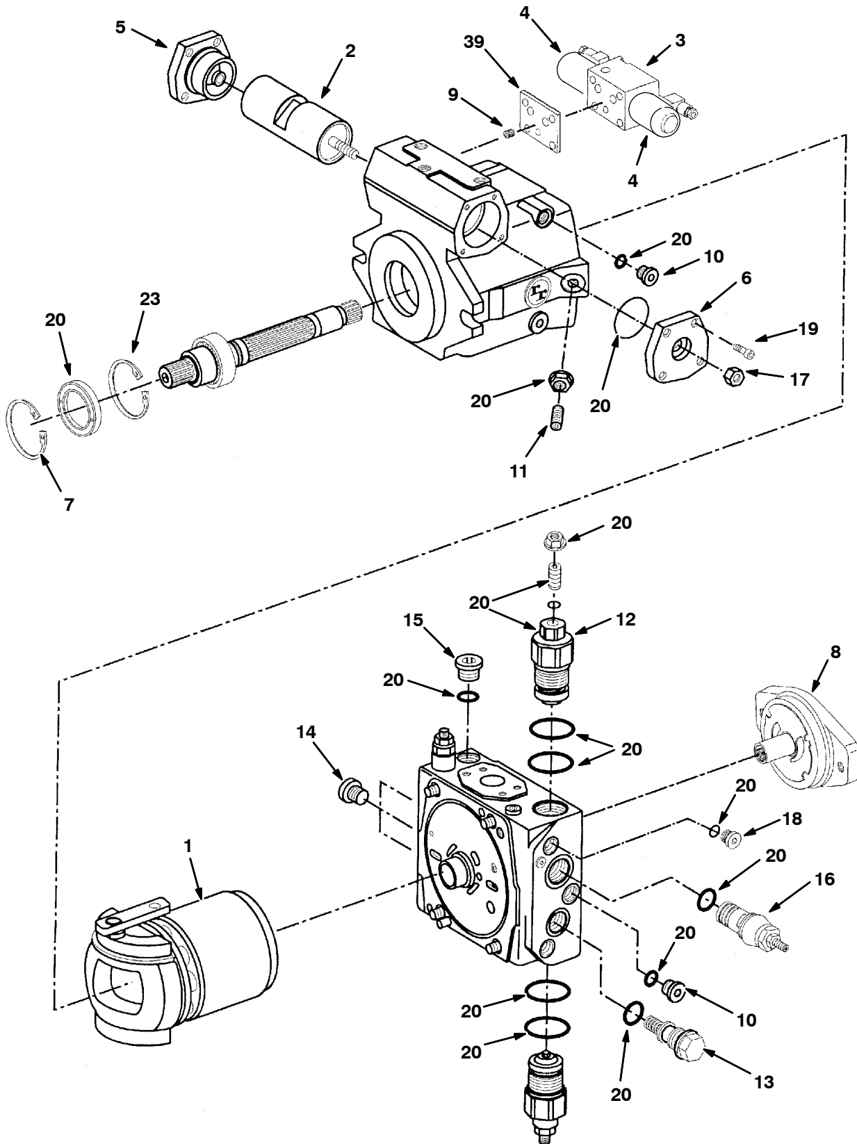
Fig. 1 - Hydraulic Piston Pump Breakdown, 767200
