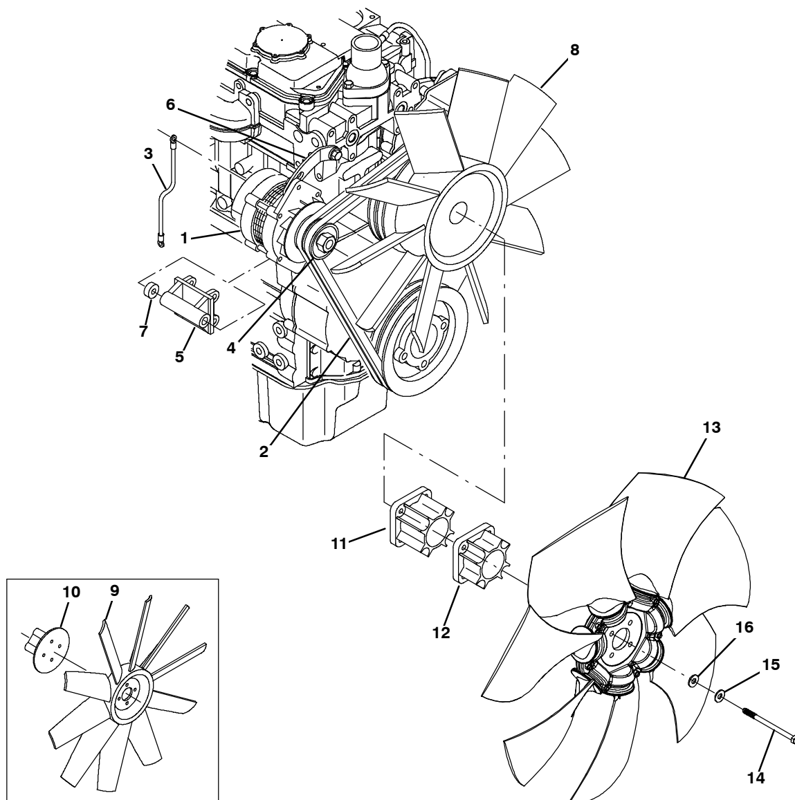
Fig. 14 - Engine Fan and Alternator Group (000000-008499)
