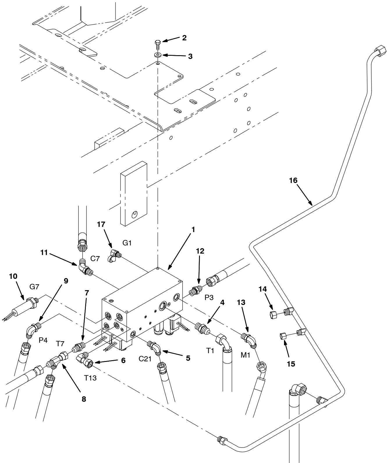
Fig. 66 - Hydraulic Side Brush Valve Group
