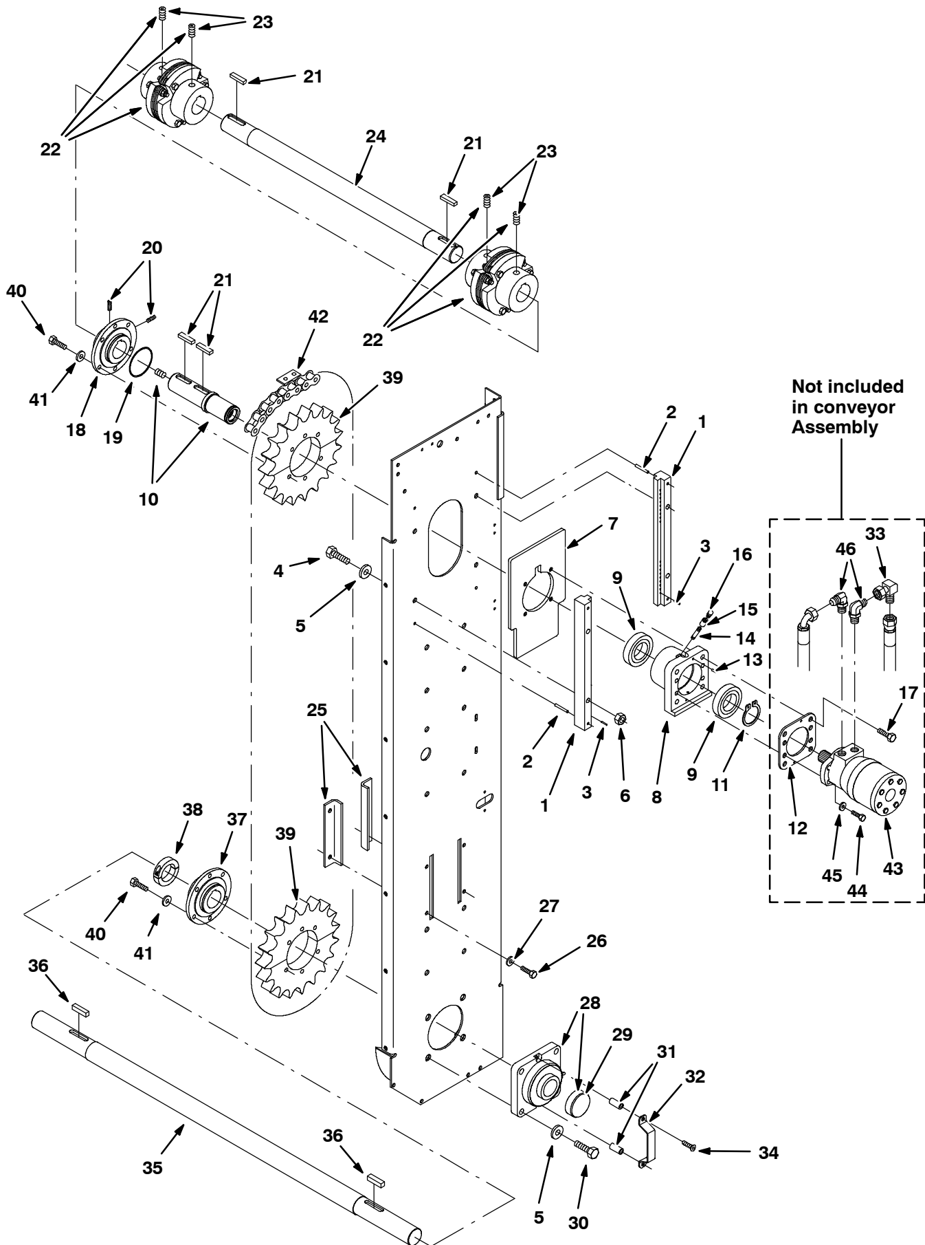
Fig. 29 - Conveyor Drive Group
