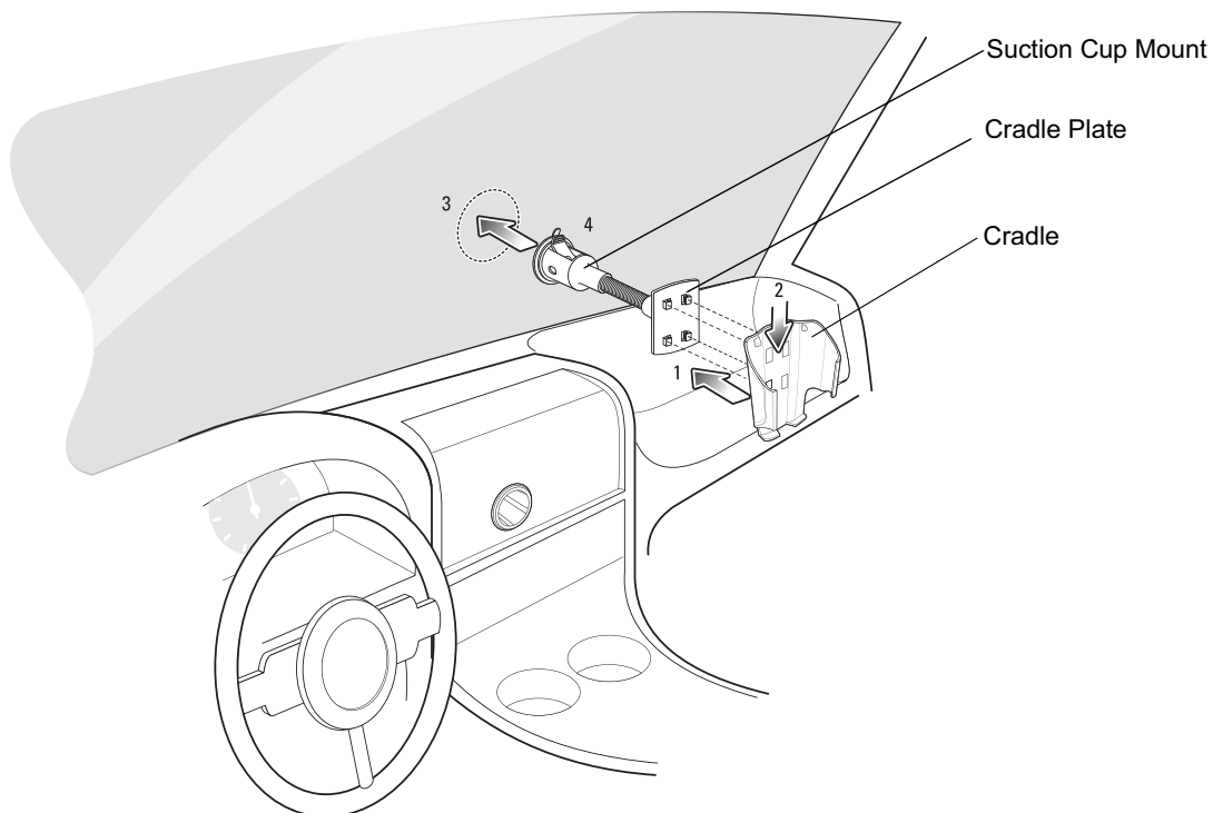
Figure 2-25 Windshield Installation
