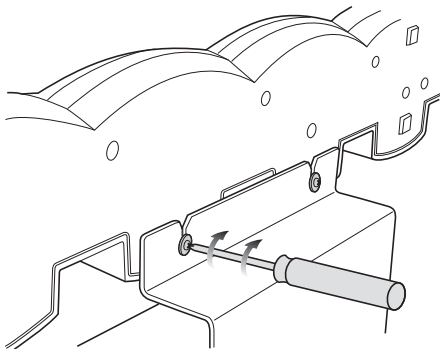
Figure 2-14 Mounting Screws
