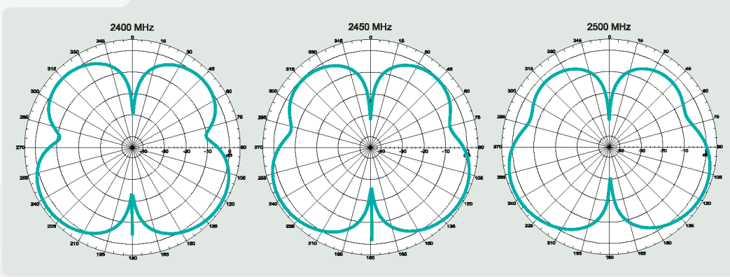
Figure 4: Pulse W1027 Antenna Gain Performance
