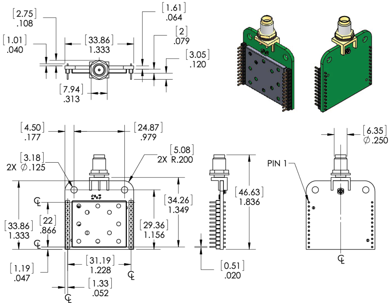
Figure 1: RF220SUMechanical Drawing
