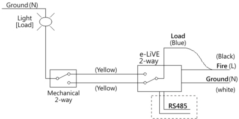
A-1 [ Mechanical 2-way directly control the Light ]
