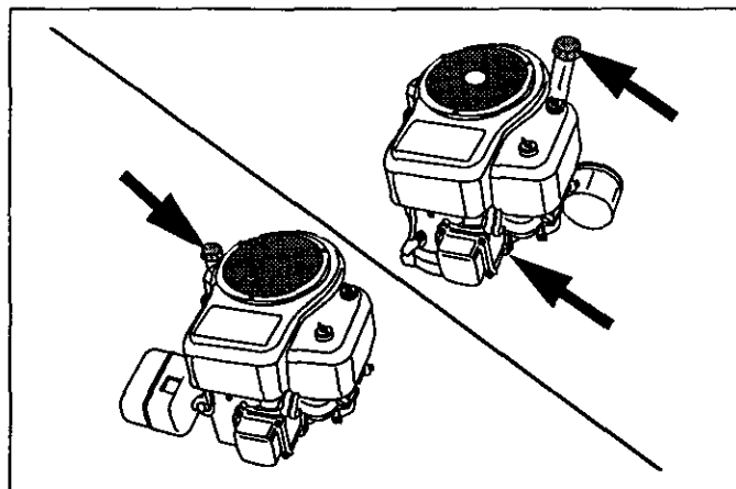
Figure 20. Oil Filler Locations
