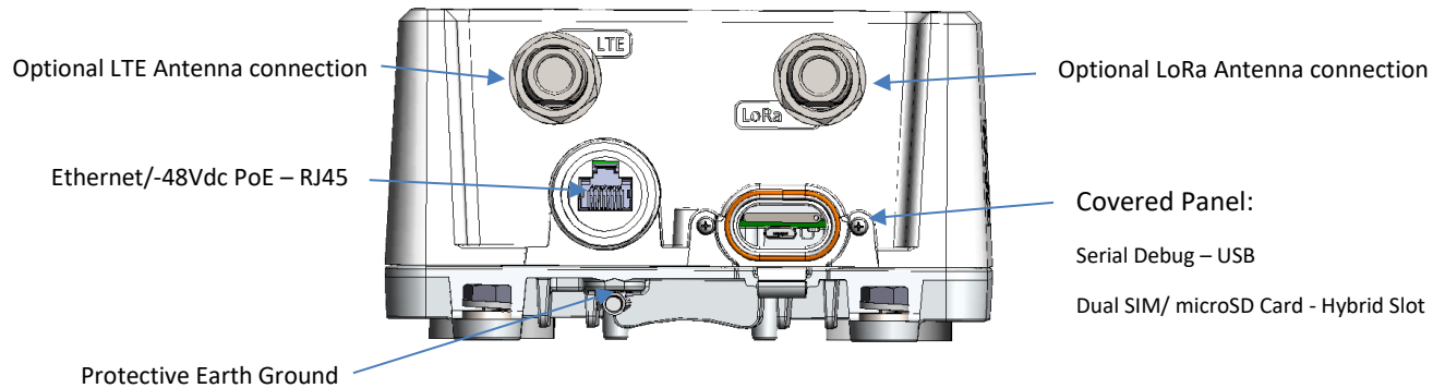
Figure 3: Kona Enterprise Gateway Bulkhead Layout
