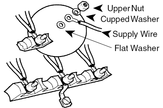
FIG. 10 Conductor Securement
