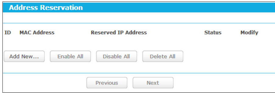
Figure 5-42 Address Reservation
