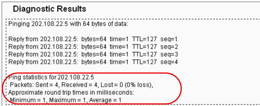
Figure 5-106 Diagnostic Results
