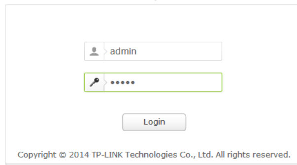
Figure 3-2 Login Windows
