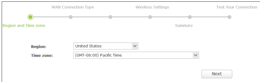
Figure 3-3 Quick Setup
