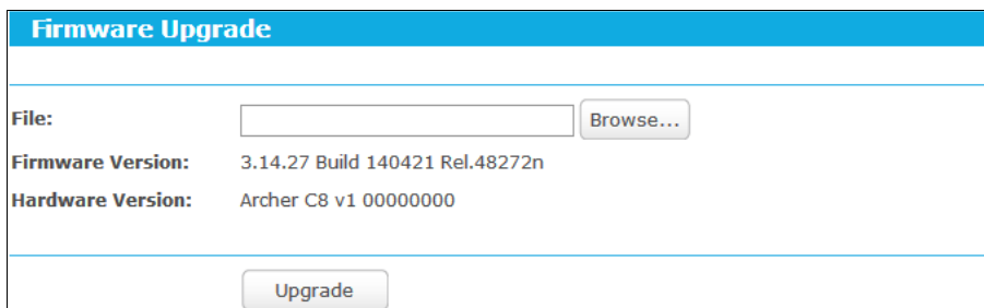
Figure 5-107 Firmware Upgrade
