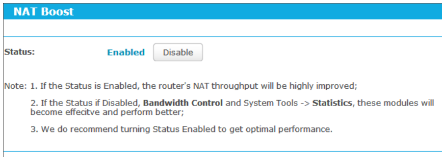
Figure 5-49 NAT Boost
