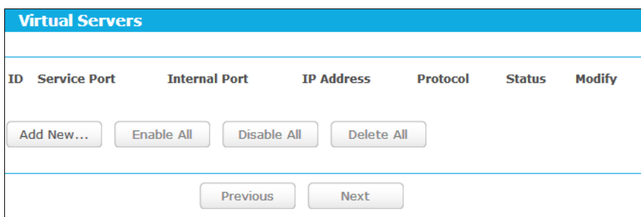
Figure 5-51 Virtual Servers
