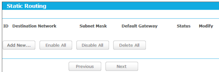
Figure 5-80 Static Routing
