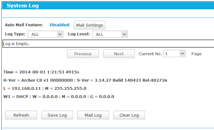
Figure 5-112 System Log
