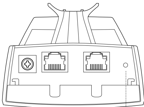
RESET Button
