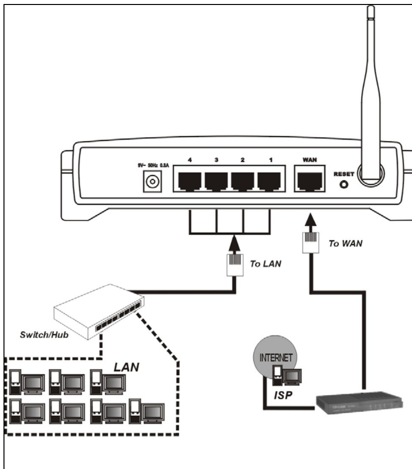
Figure 3-1 Hardware Installation of the MR0-WR541G 54Mbps Wireless Router
