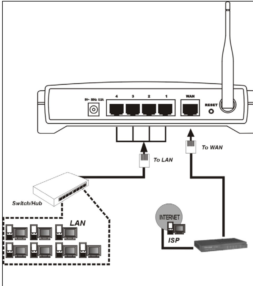
Figure 3-1 Hardware Installation of the MR0-WR641G 108Mbps Wireless Router
