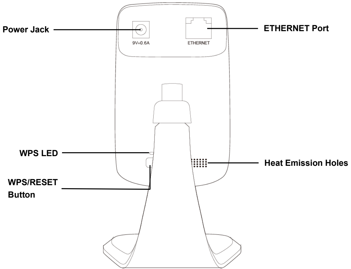
Figure 2-2 Rear Panel
