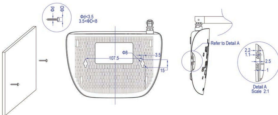
Figure 2-1 Wall-mount Install
