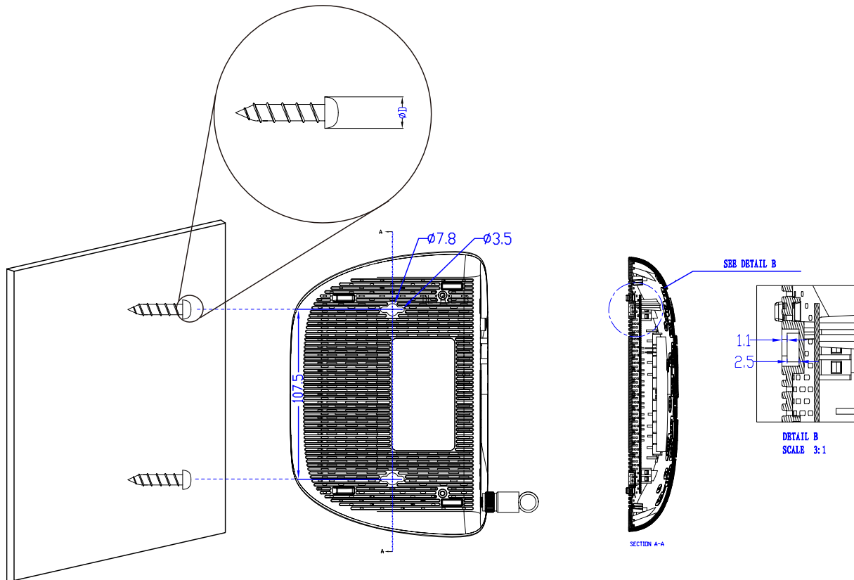
Figure 2-3 Wall-mount Install
