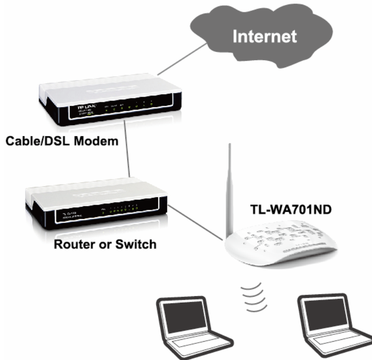
Figure 2-1 The Example of Infrastructure Network Incorporating the TL-WA701ND
