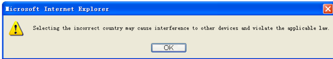
Figure 4-29 Note Dialog
