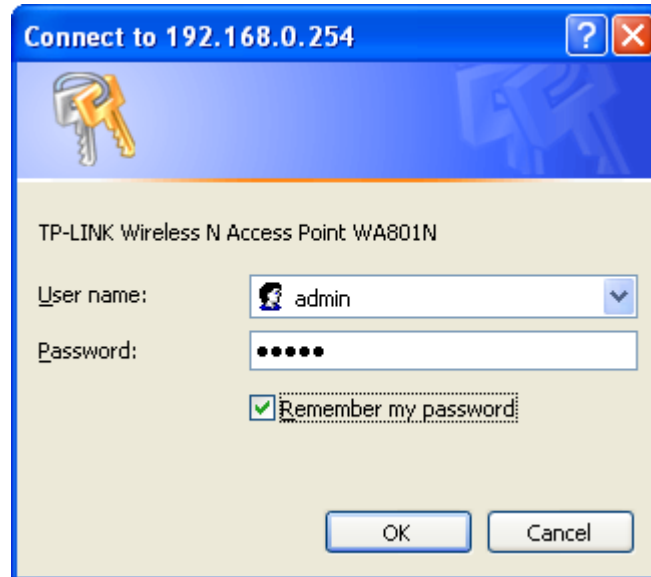
Figure 4-2 Login Windows
