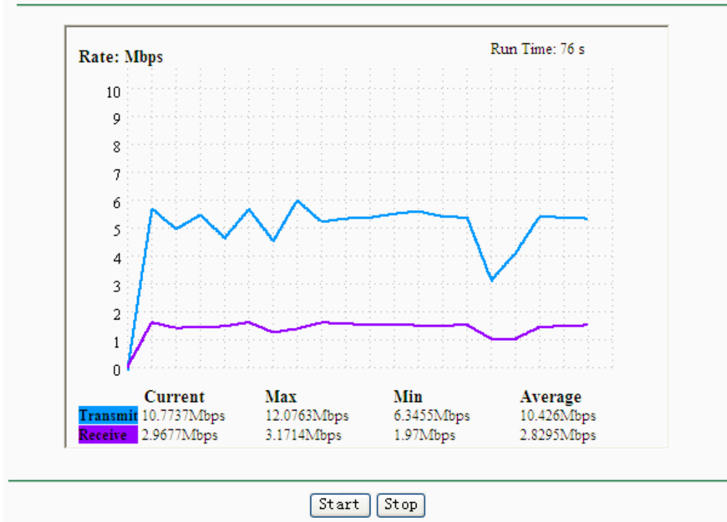
Figure 4-40 Throughput Monitor
