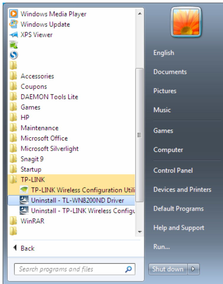
Figure 6-4 Uninstall Driver
