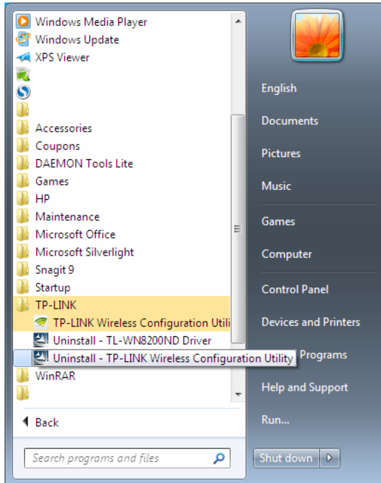
Figure 6-1 Uninstall Utility
