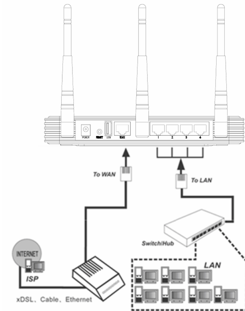
Figure 2-1 Hardware Installation of the TL-WR1043ND Wireless N Gigabit Router
