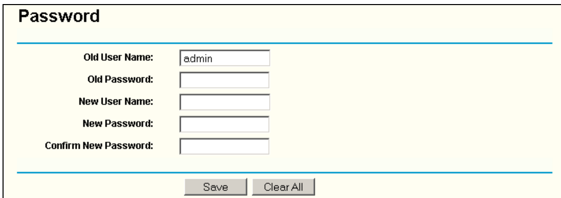
Figure 5-53 Password
