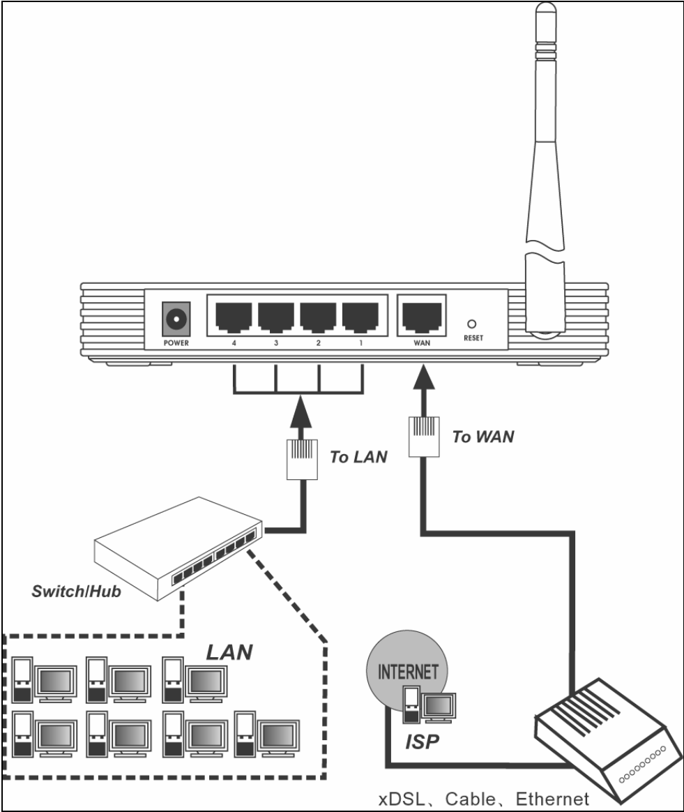
Figure 3-1 Hardware Installation of the TL-WR541G 54Mbps Wireless Router
