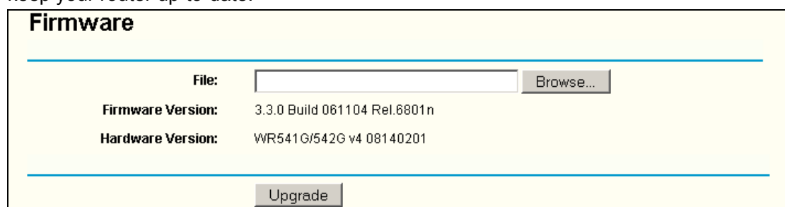
Figure 5-49 Firmware Upgrade
