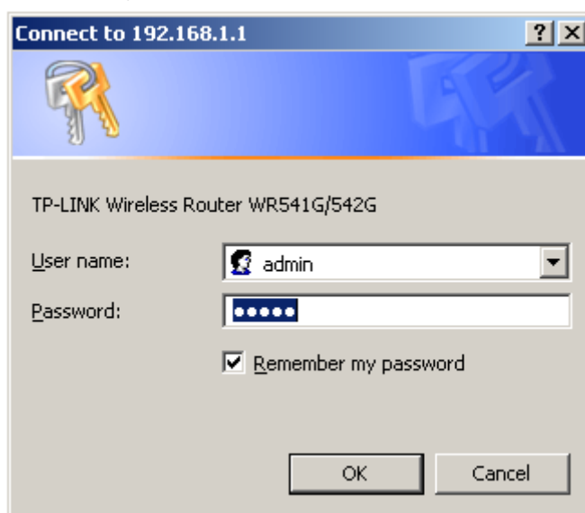
Figure 4-4 Login Windows
