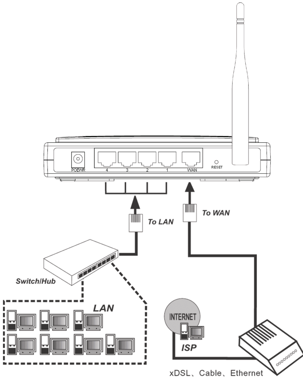
Figure 3-1 Hardware Installation of the MR4-WR642G 108Mbps Wireless Router
