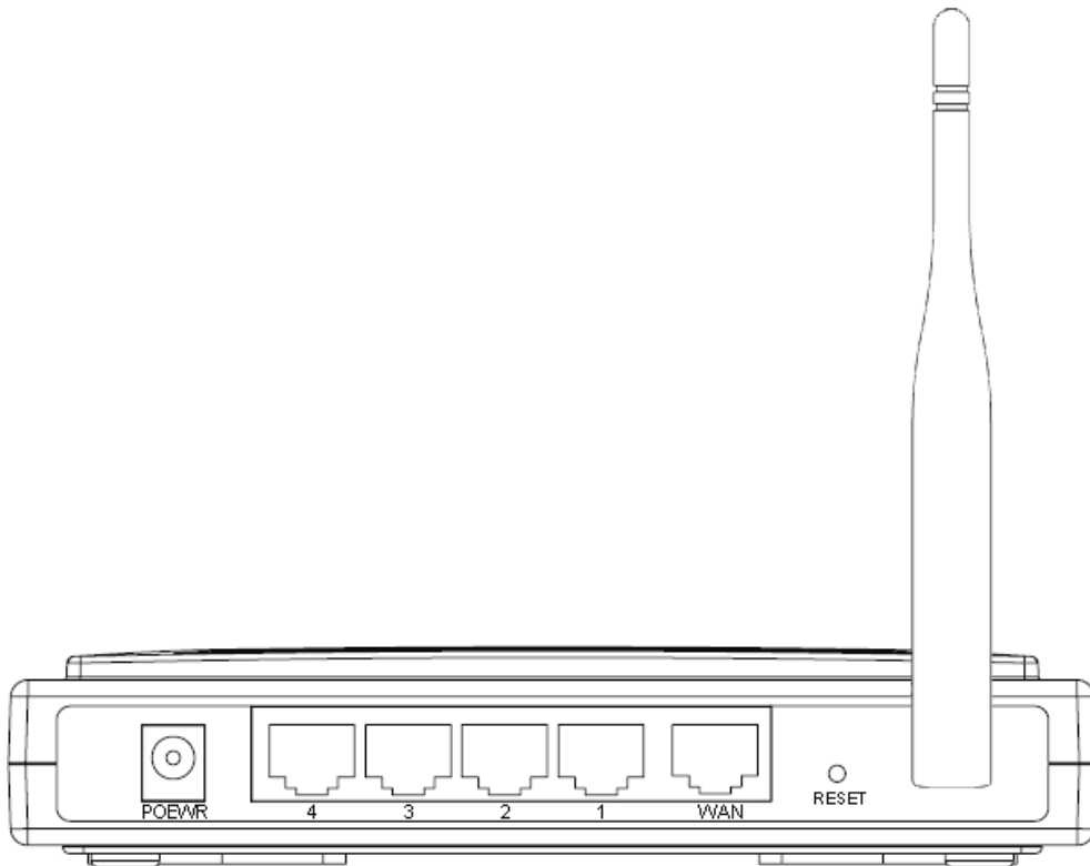
Figure 2-2 Rear Panel sketch
