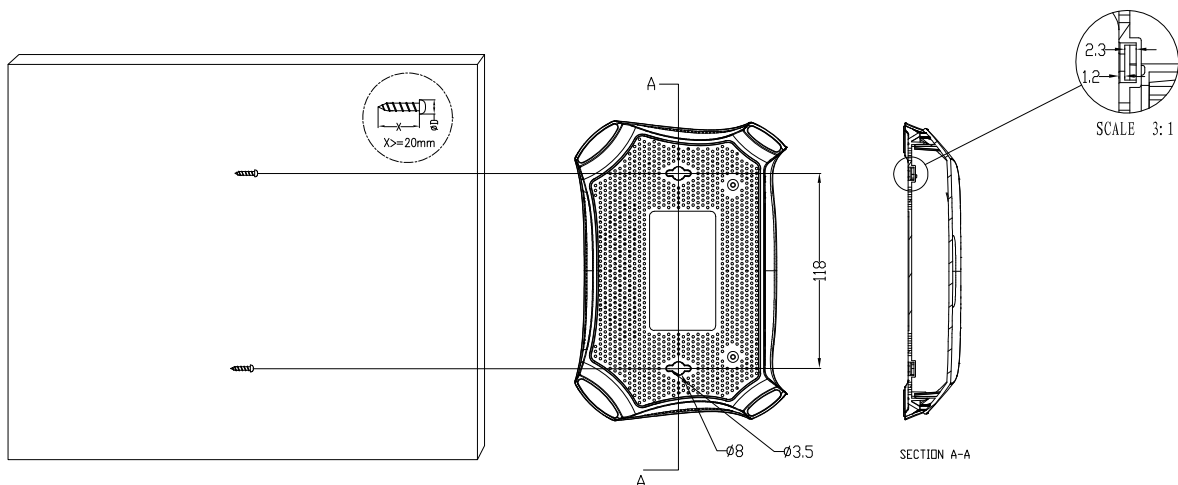
Figure 2-2 Wall-mount Install
