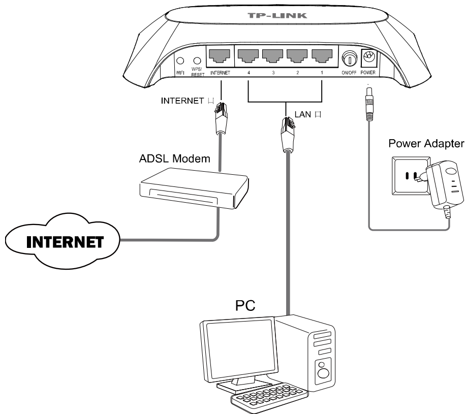
Figure 2-1 Hardware Installation of the TL-WR840N 300Mbps Wireless N Router
