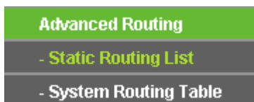
Figure 4-58 Advanced Routing
