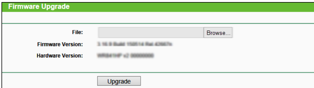
Figure 4-78 Firmware Upgrade
