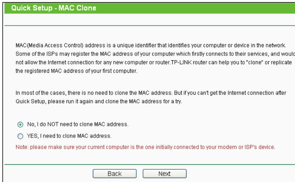
Figure 3-7 MAC Clone
