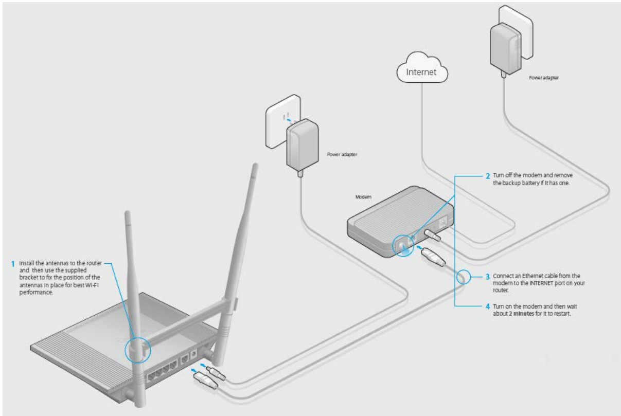
Figure 2-1 Hardware Installation
