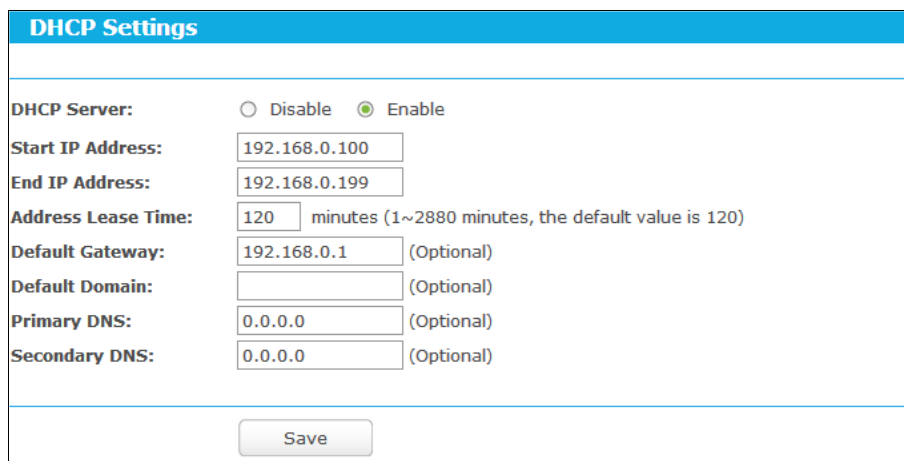
Figure 3-31 DHCP Settings
