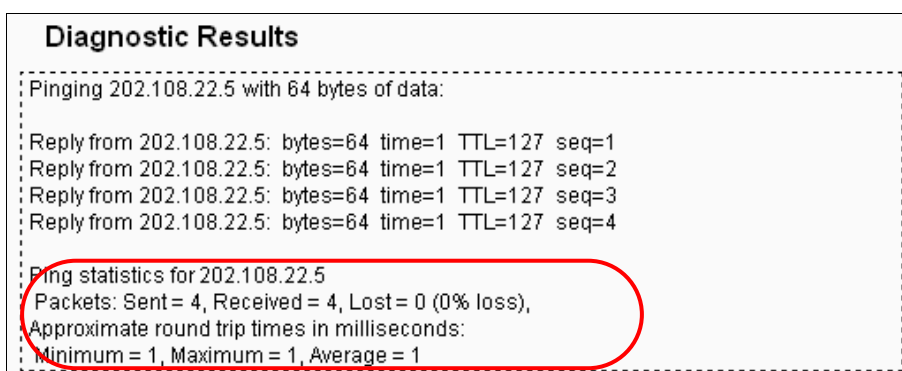
Figure 3-87 Diagnostic Results
