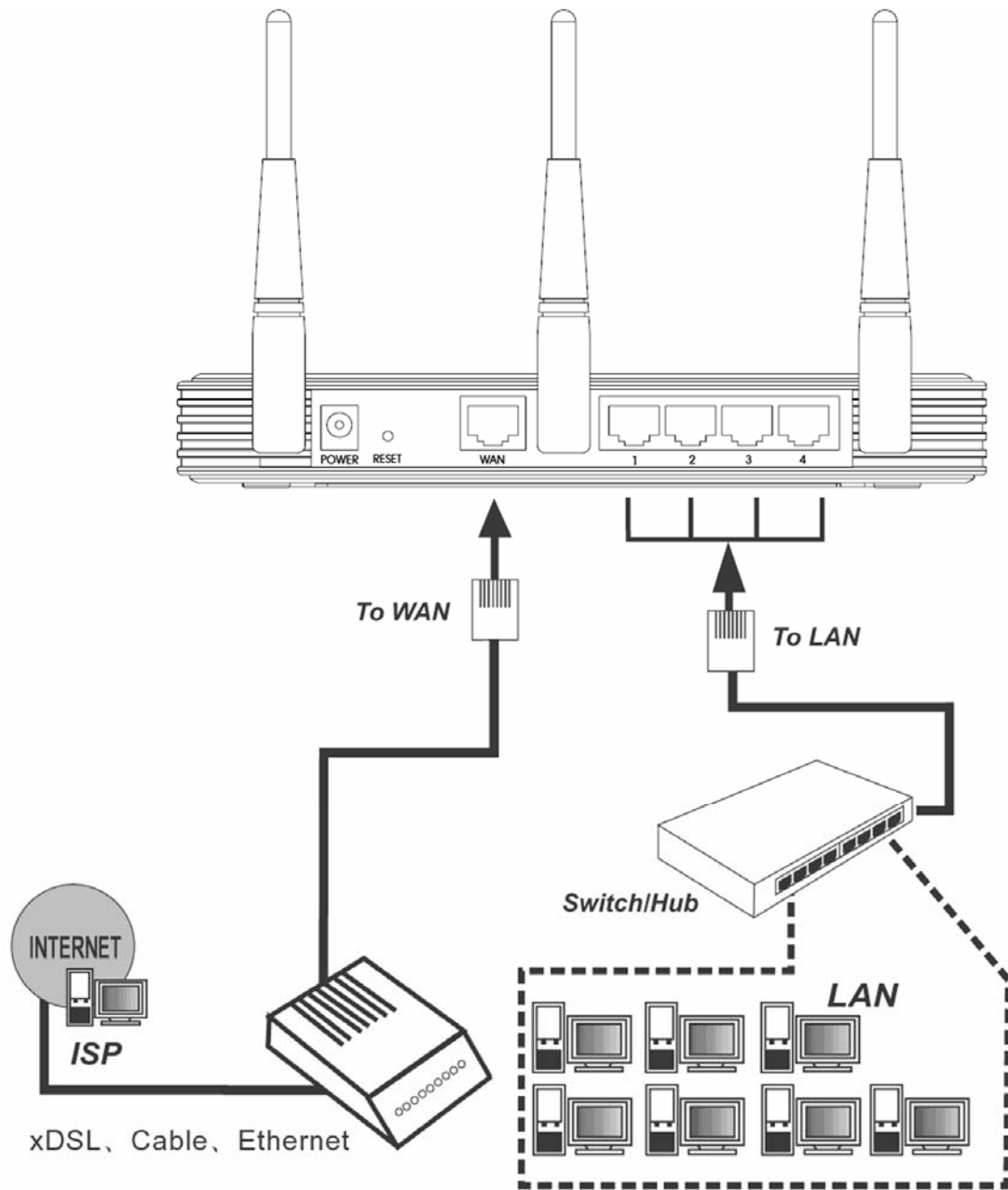
Figure 2-1 Hardware Installation of the TL-WR940N Wireless N Router
