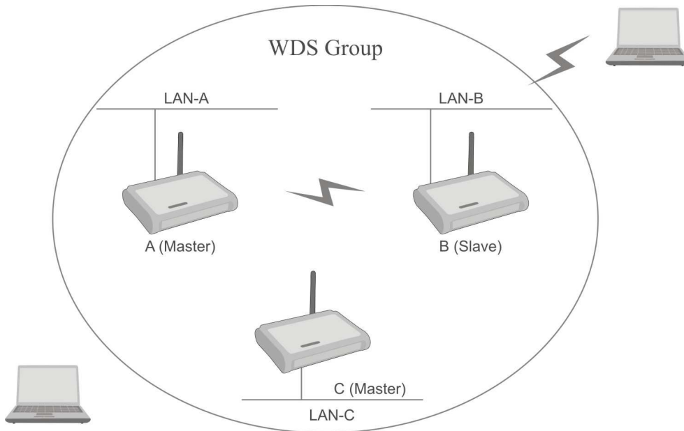
WDS + AP Mode Application
