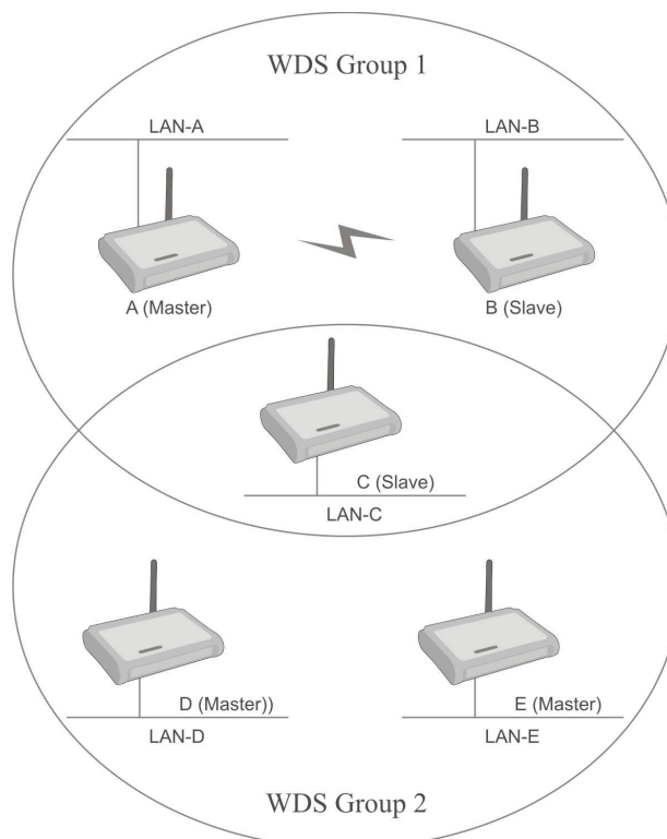
WDS Mode Application (Multiple WDS Group)
