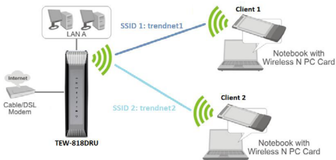
Access Point Mode with Multiple SSID
