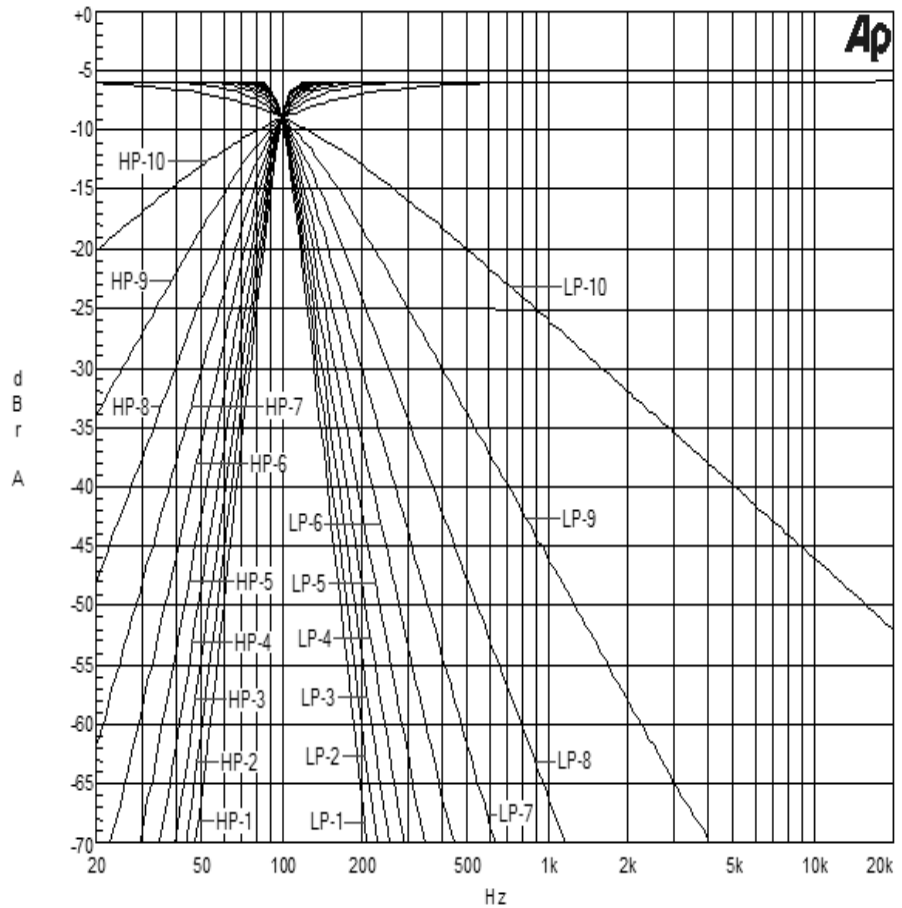
Fig. 7 Amp#1 and Amp#2 Left/Right channel frequency response. Output signal level at -6 dB which is equivalent to 37.5 W into 8 Ohms or 70 W into 4 Ohms.
