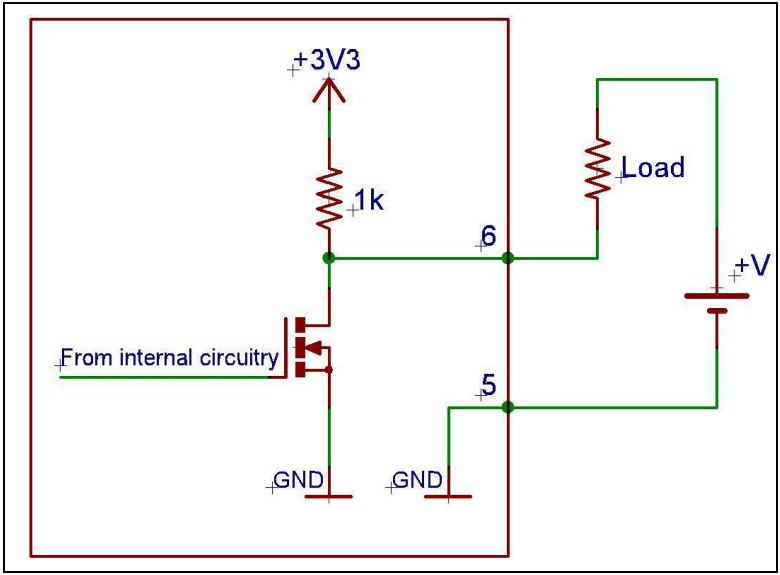
Figure 25: Connecting an external load to output #1
